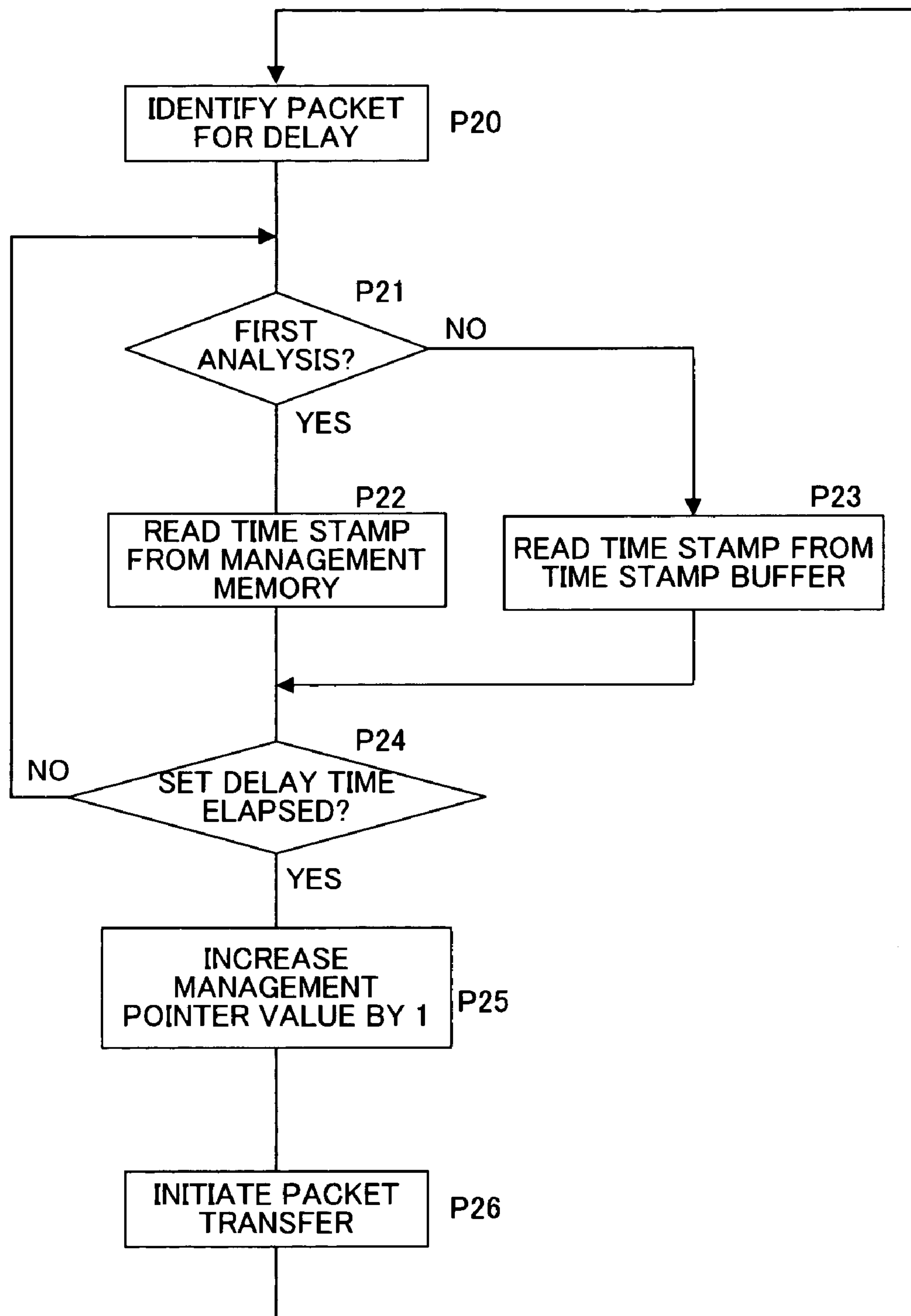
FLOWCHART OF OPERATIONS IN PACKET DELAY
