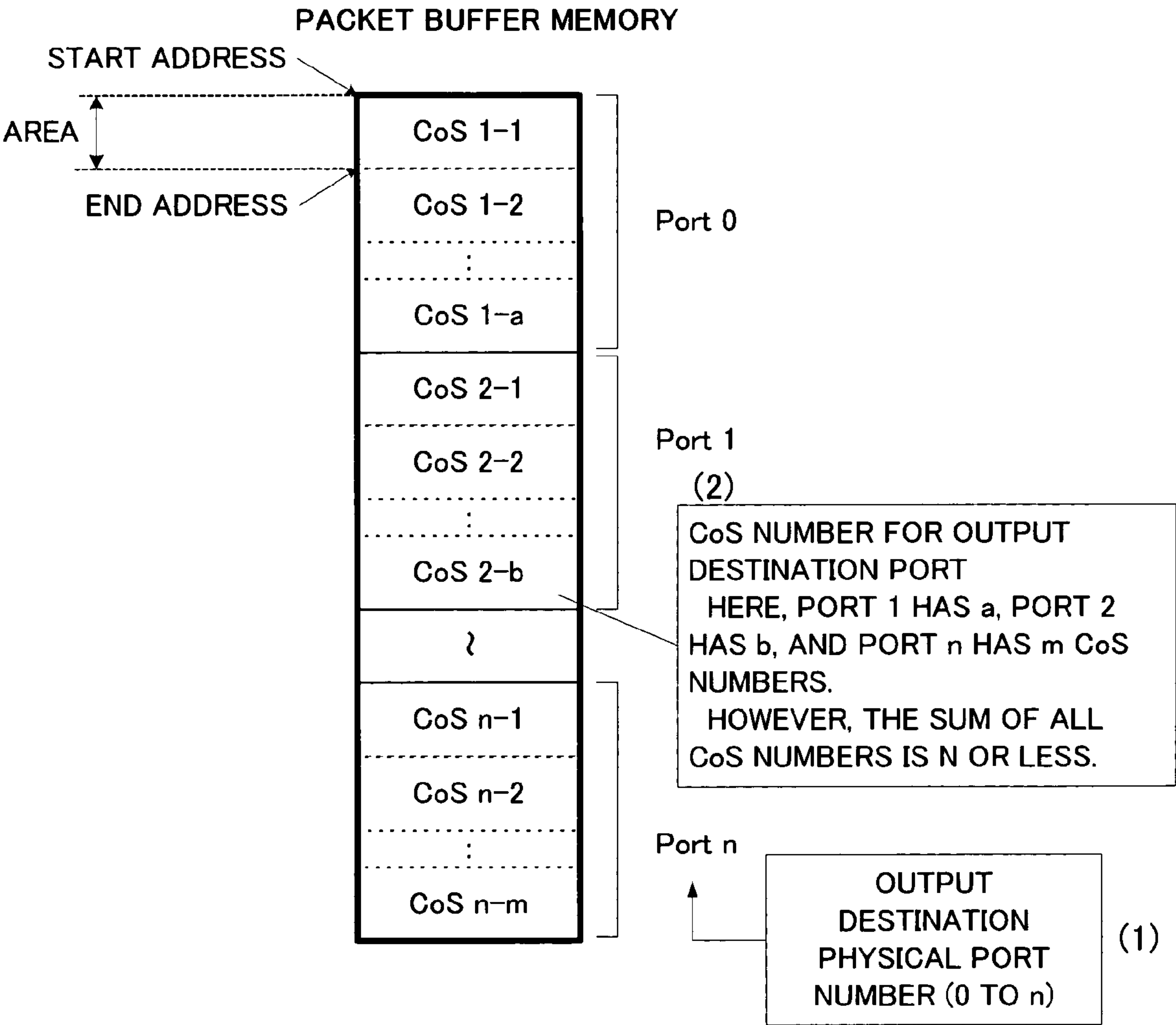
DIAGRAM OF PACKET BUFFER CONFIGURATION
