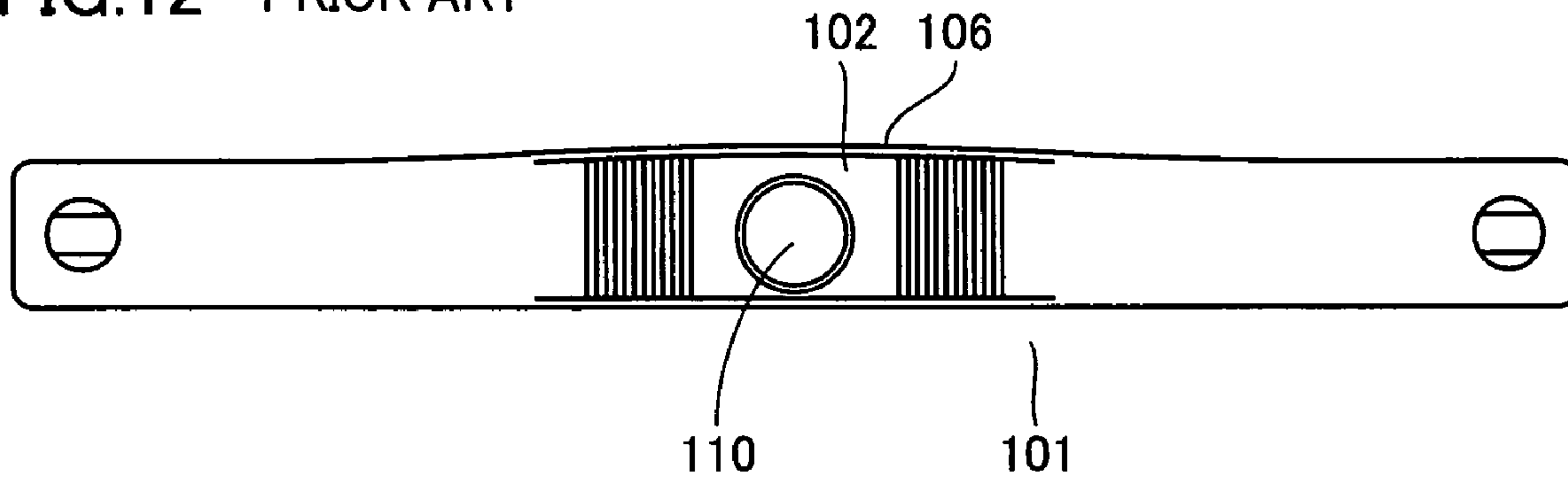
FIG.12 PRIOR ART
