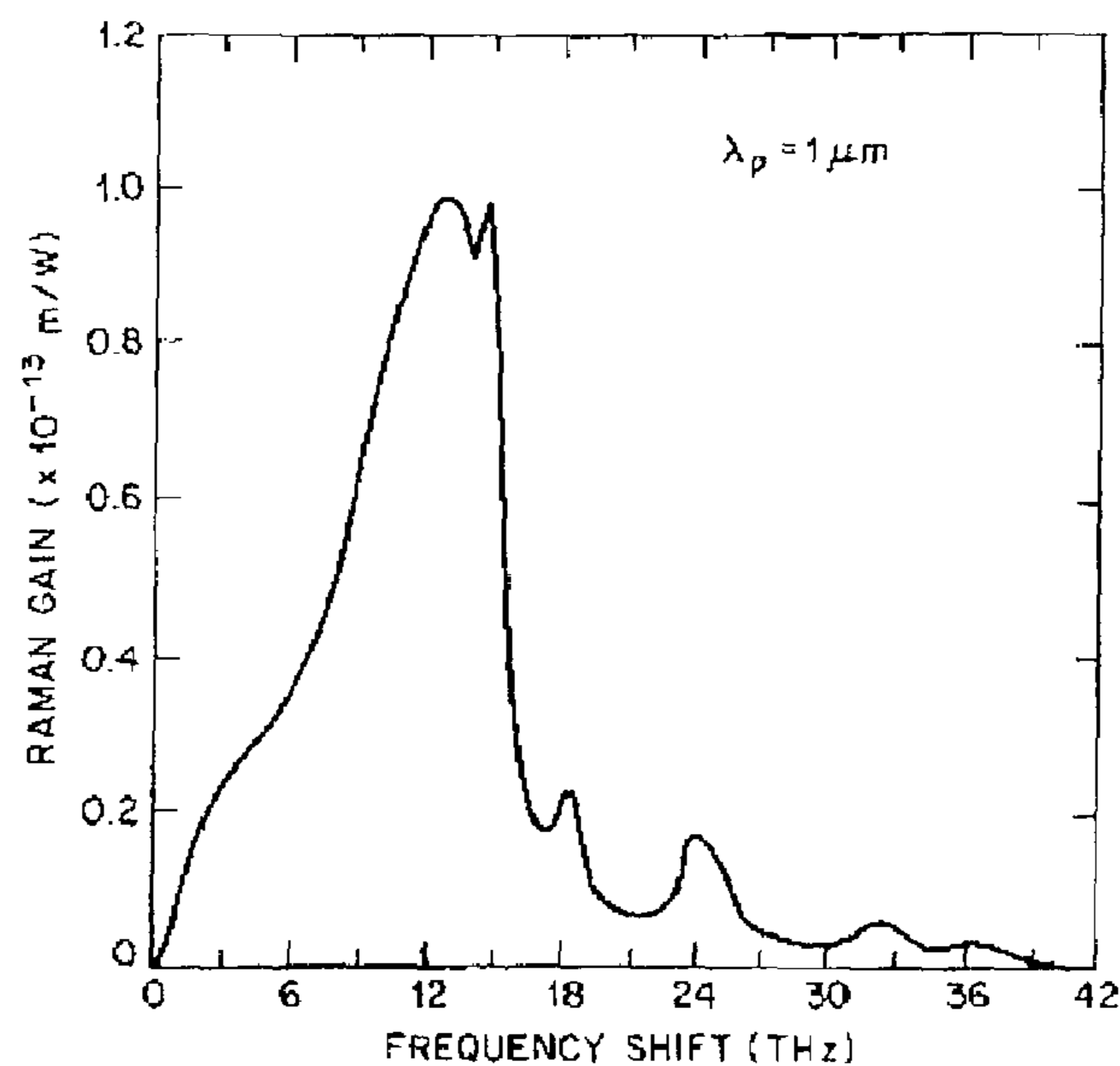
Fig. 8.1 Measured Raman gain spectrum for fused silica at a pump wavelength \lambda_p = 1 \mu m . The Raman gain scales inversely with \lambda_p (after Ref. 11 ©1980 IEEE).
