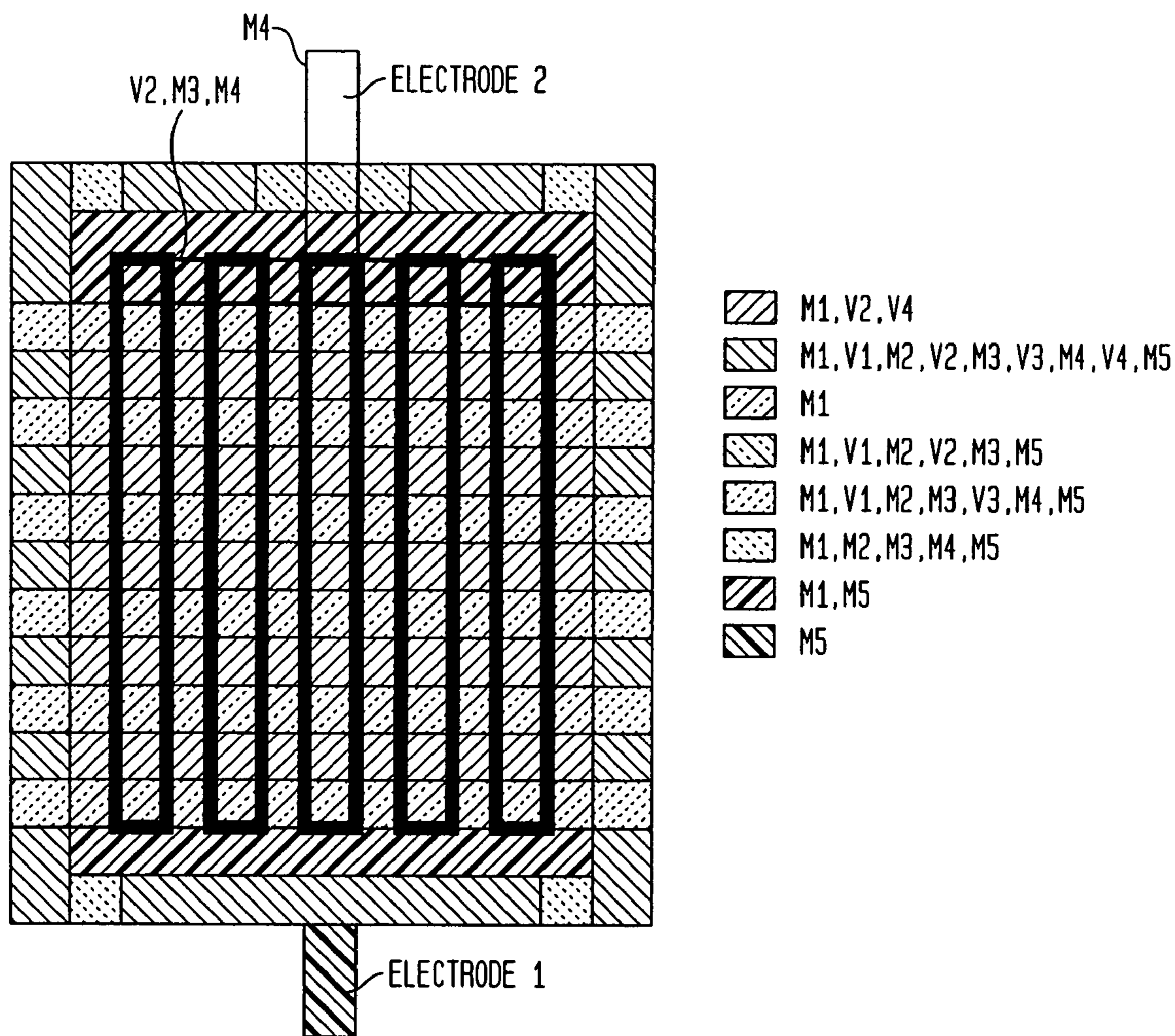
FIG. 16A (CASE 1 ALL LAYERS)
