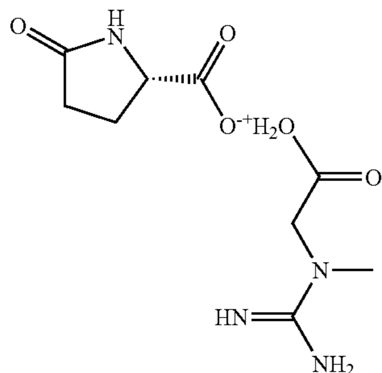
(2-(1-methylguanidino)acetyl)oxonium pyroglutamate
