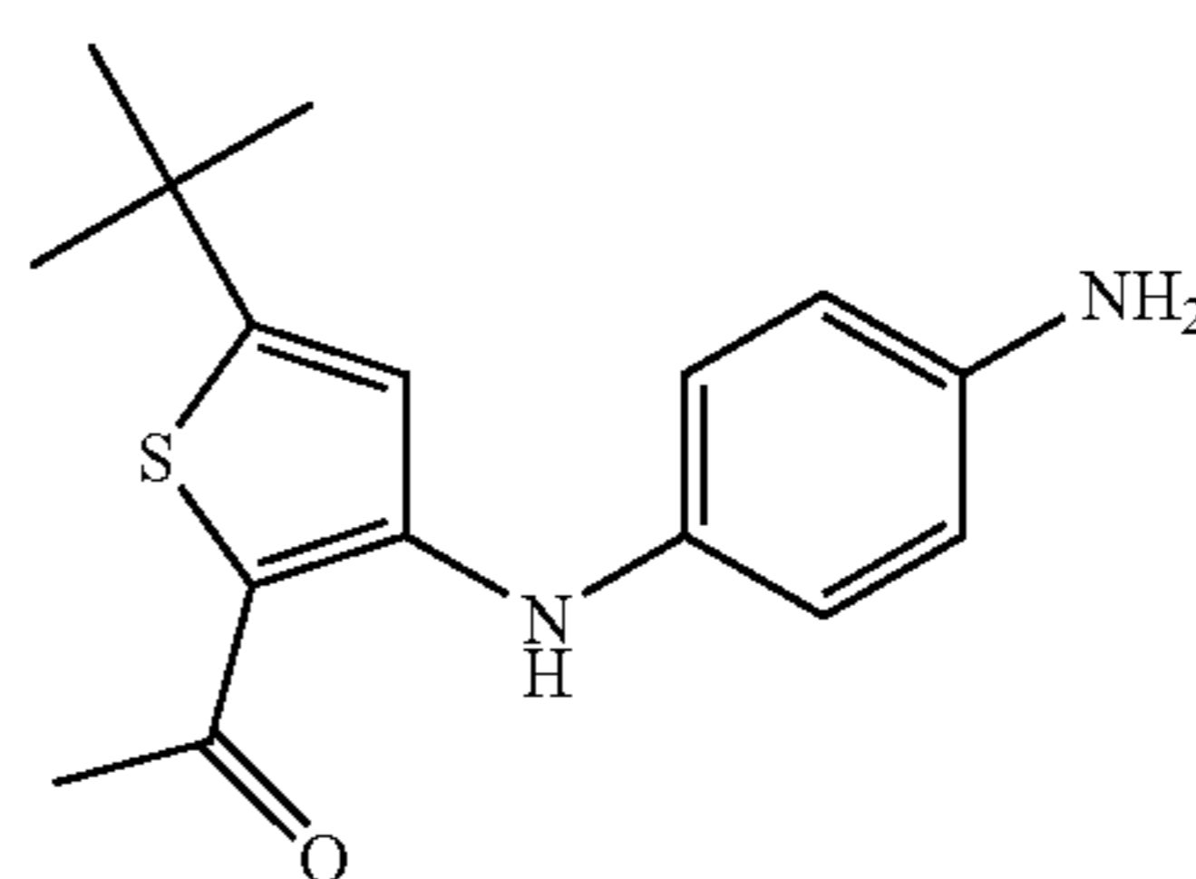
1-[3-(4-Amino-phenyl-amino)-5-tert-butyl-thiophen-2-yl]ethanone
