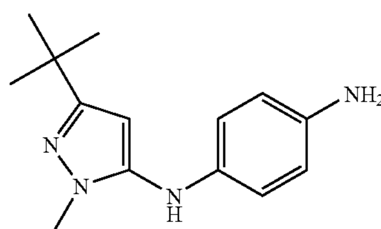
N-(5-tert-Butyl-2-methyl-2H-pyrazol-3-yl)-benzene-1,4-diamine
