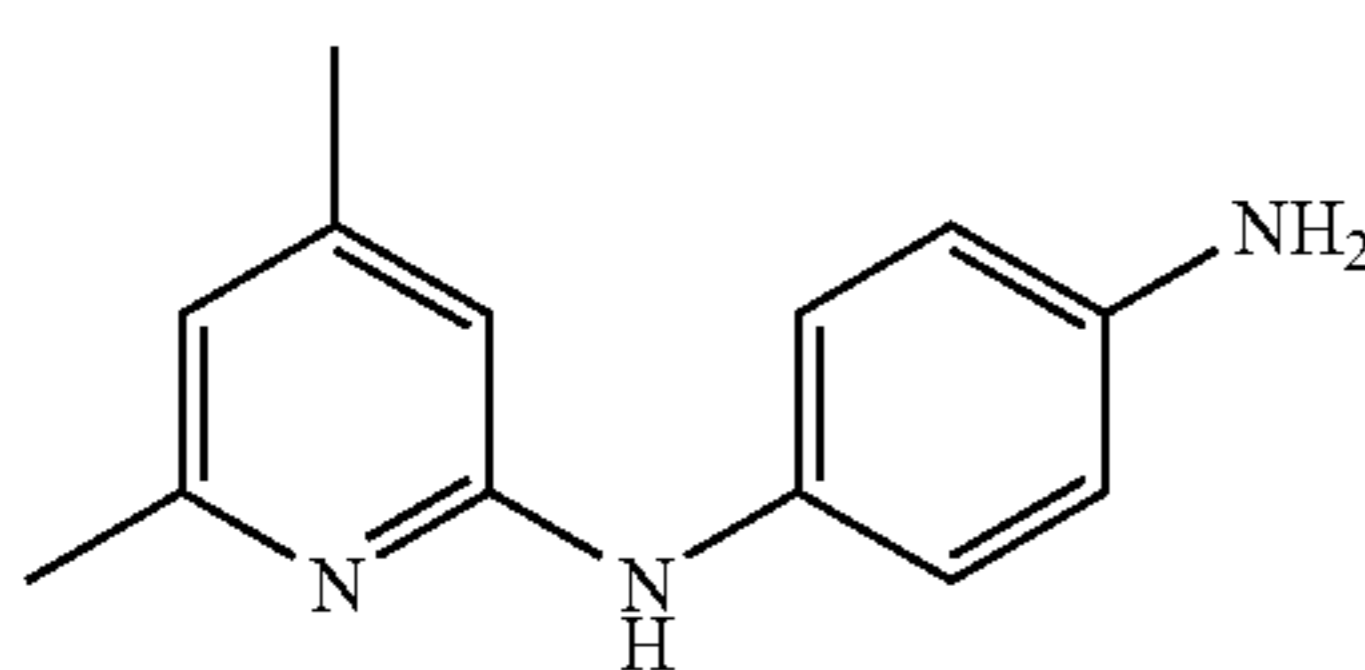
N-(4,6-Dimethyl-pyrid-2-yl)-benzene-1,4-diamine
