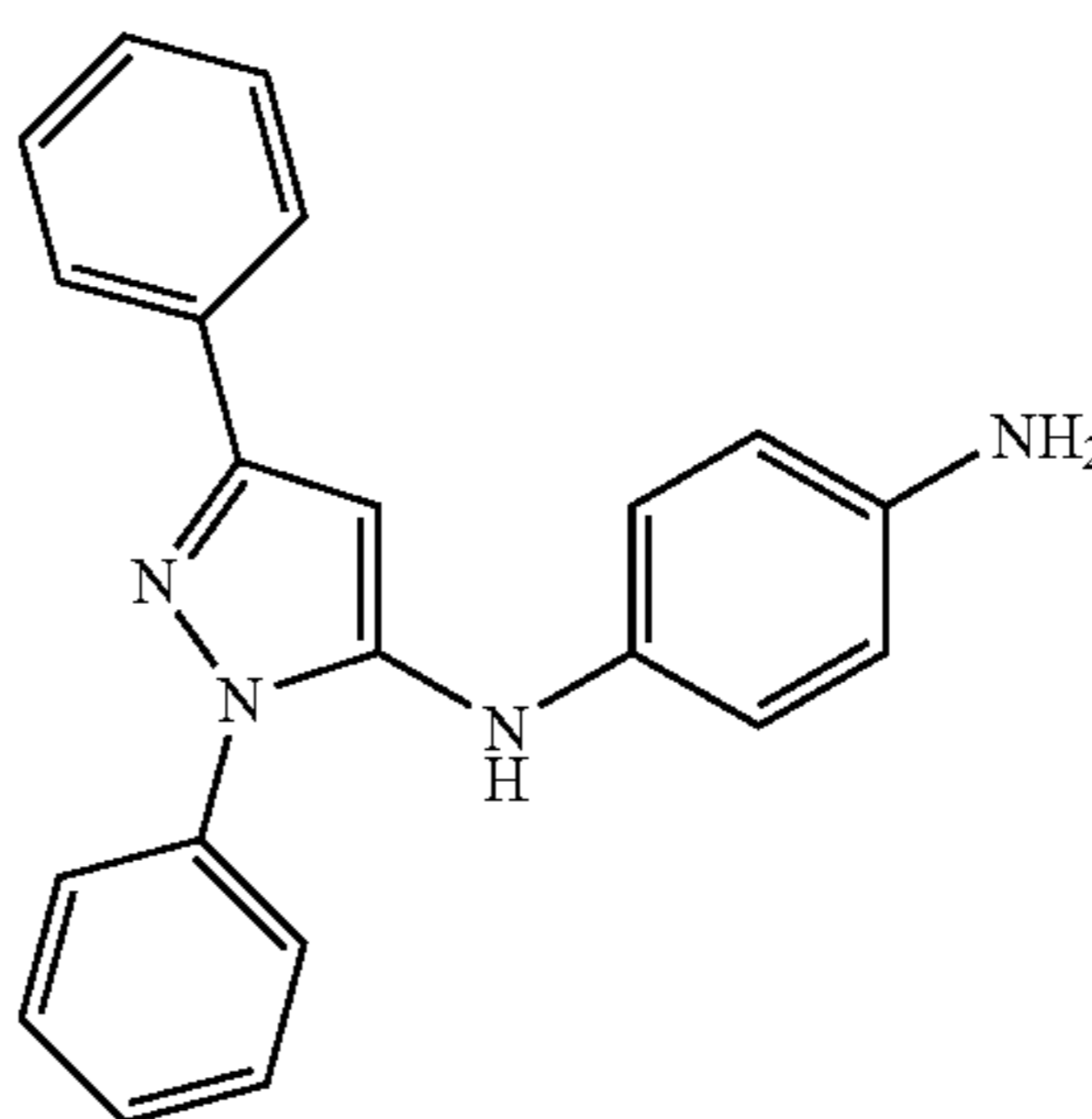
N-(2,5-Diphenyl-2H-pyrazol-3-yl)-benzene-1,4-diamine
