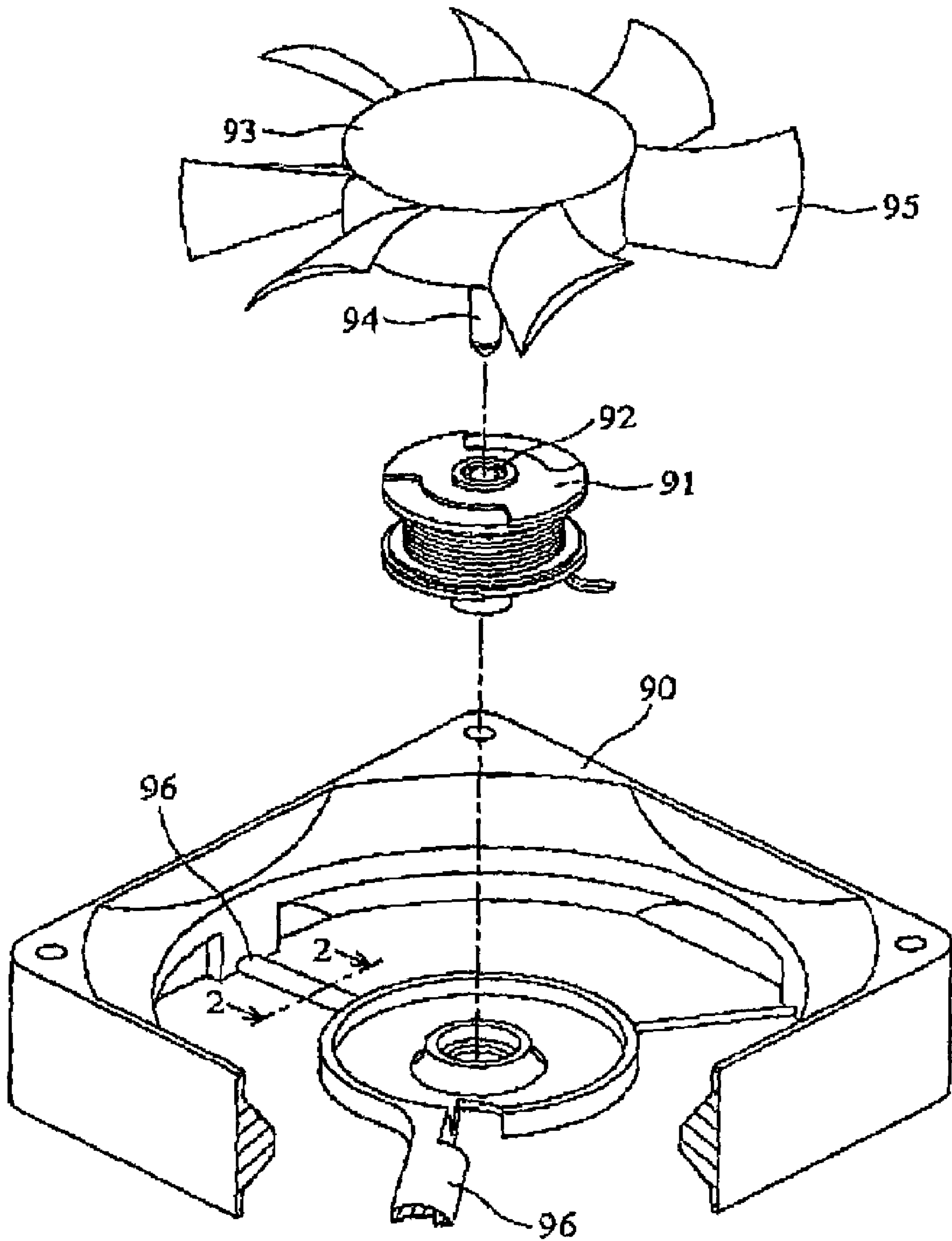
FIG. 1 (PRIOR ART)
