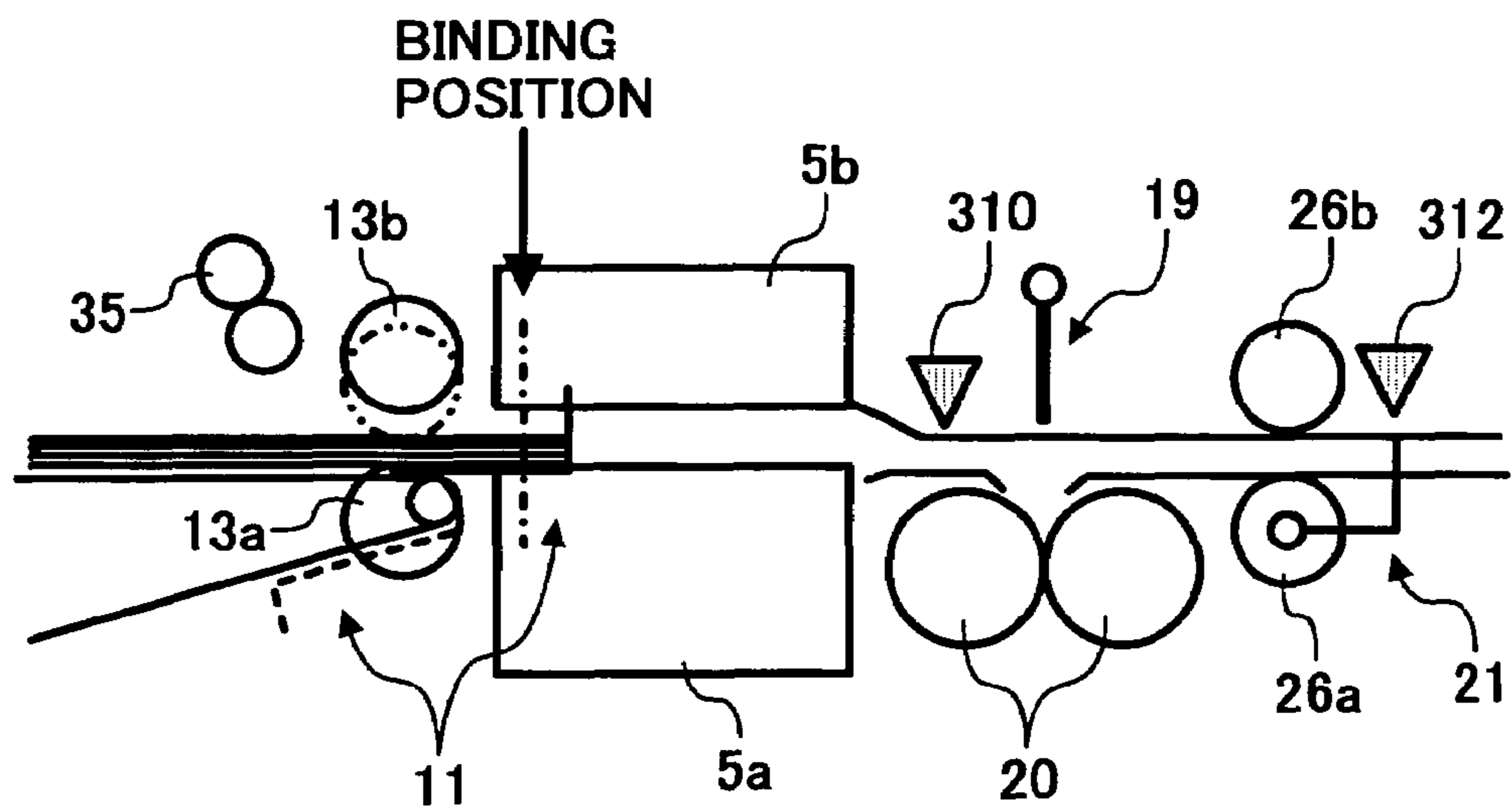
FIG. 10A ADJUSTMENT
