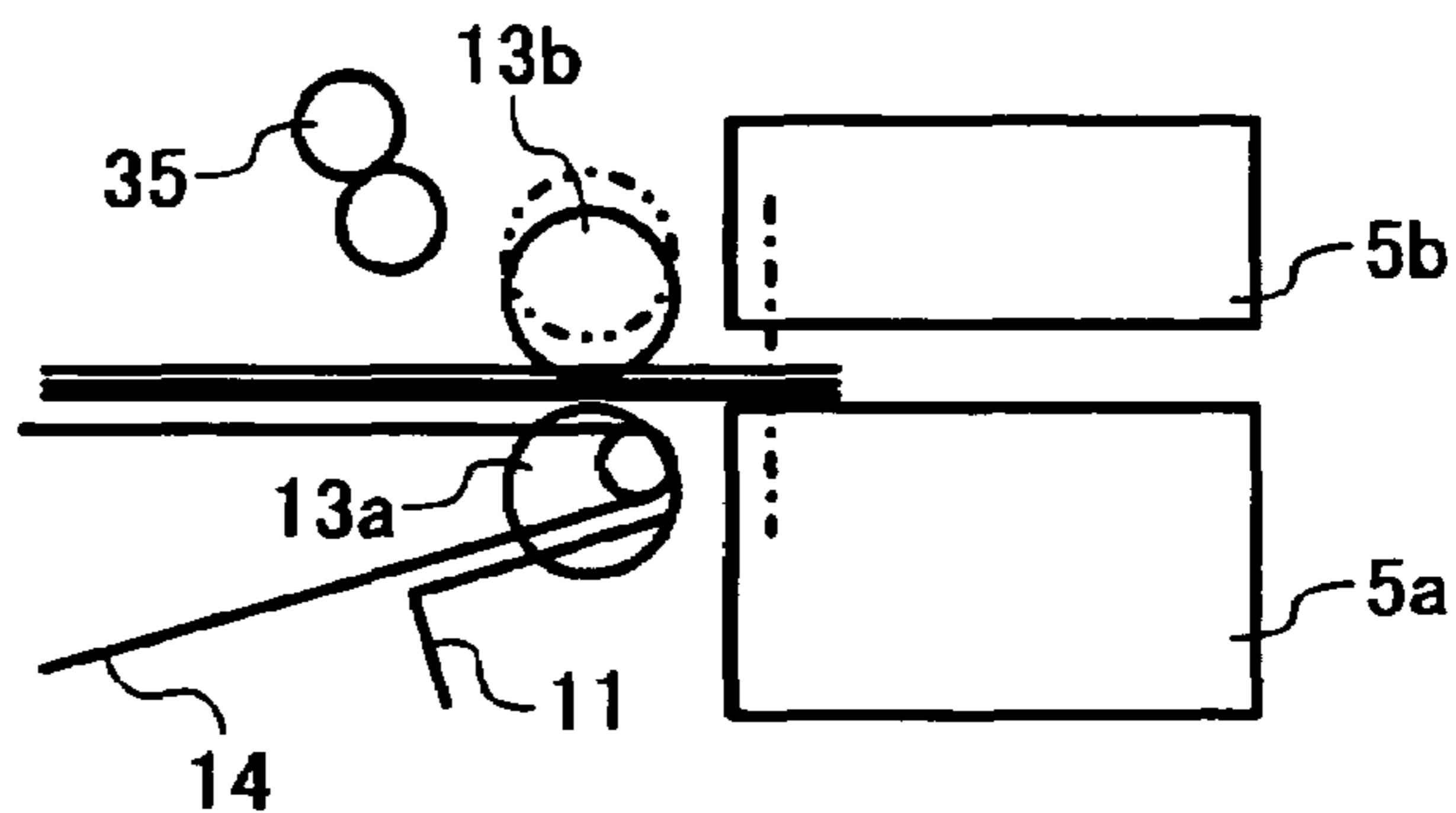
FIG. 9C STAPLER MOVEMENT
