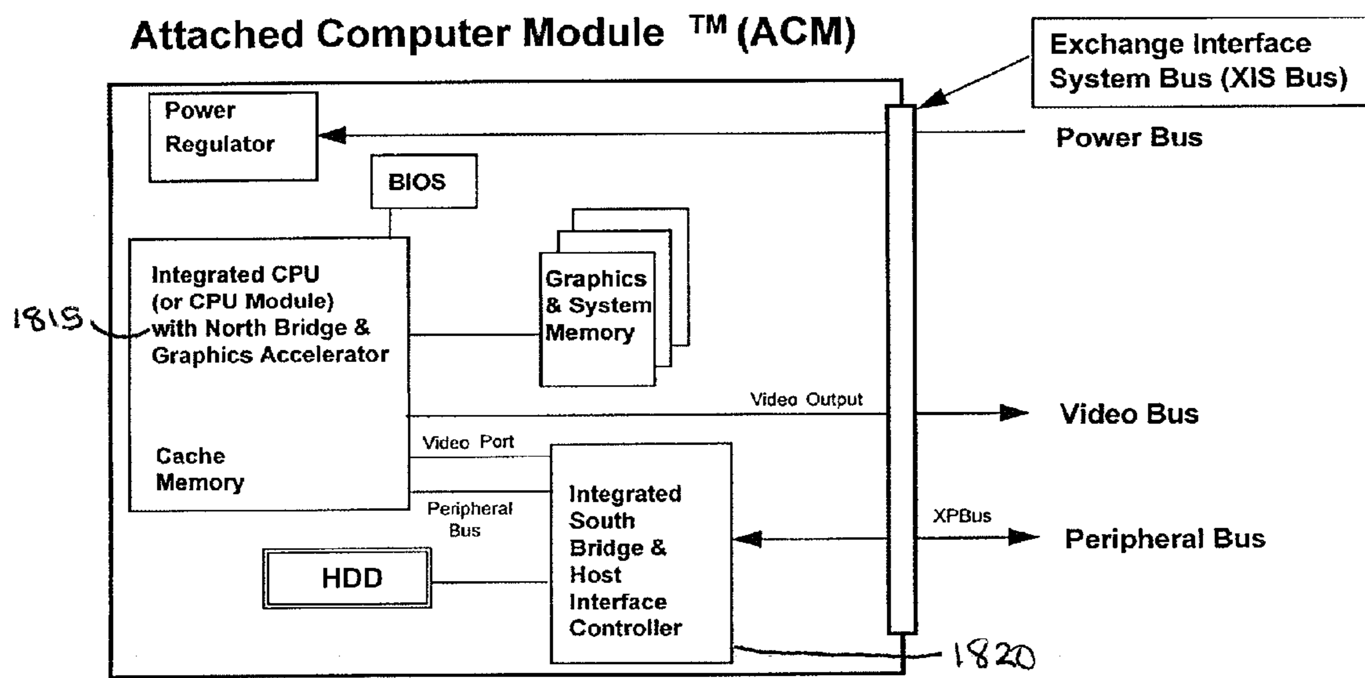
Attached Computer Module with Integrated CPU/NB/Graphics and Integrated HIC/SB
