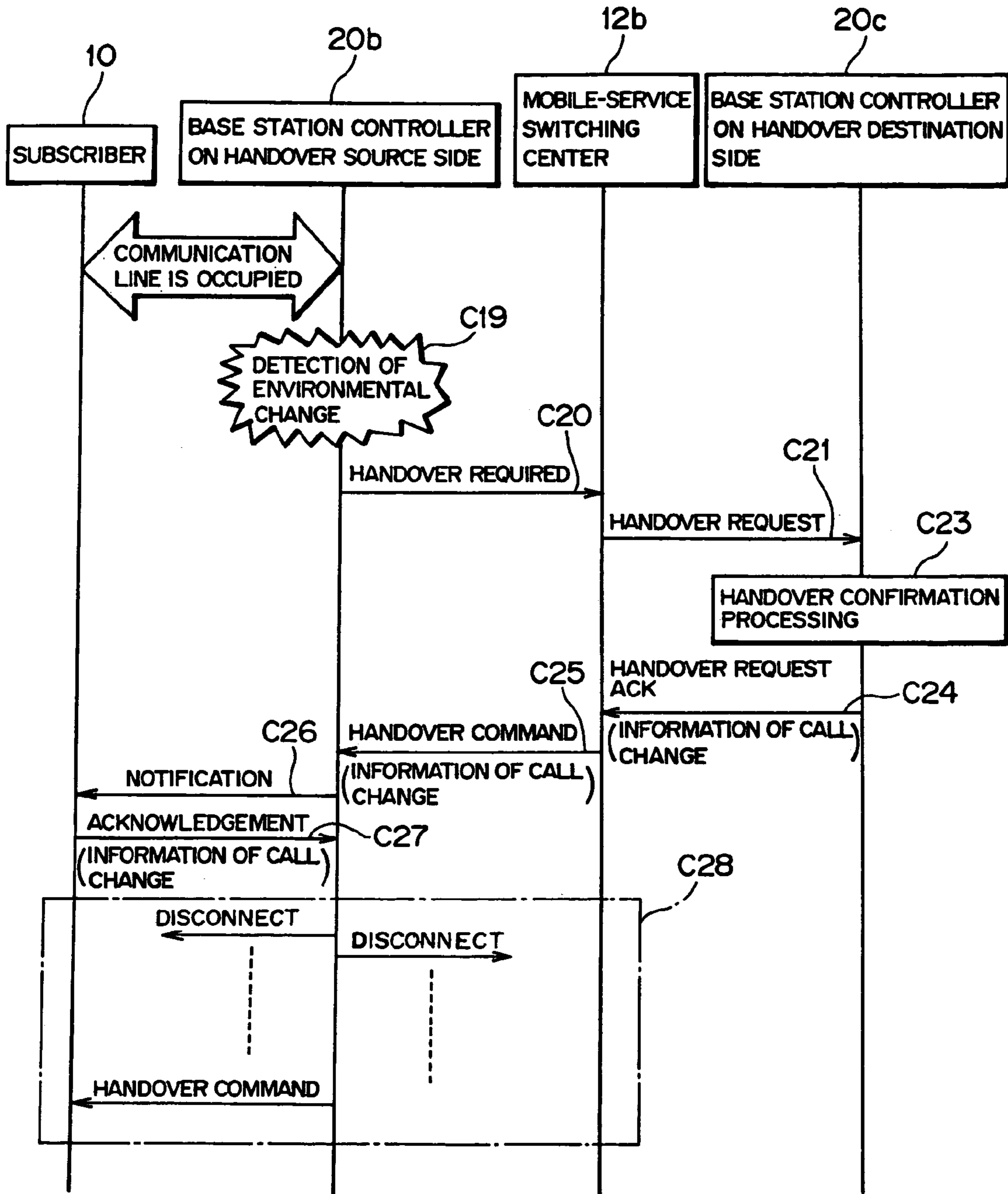
EXAMPLE OF SIGNALING SEQUENCE
