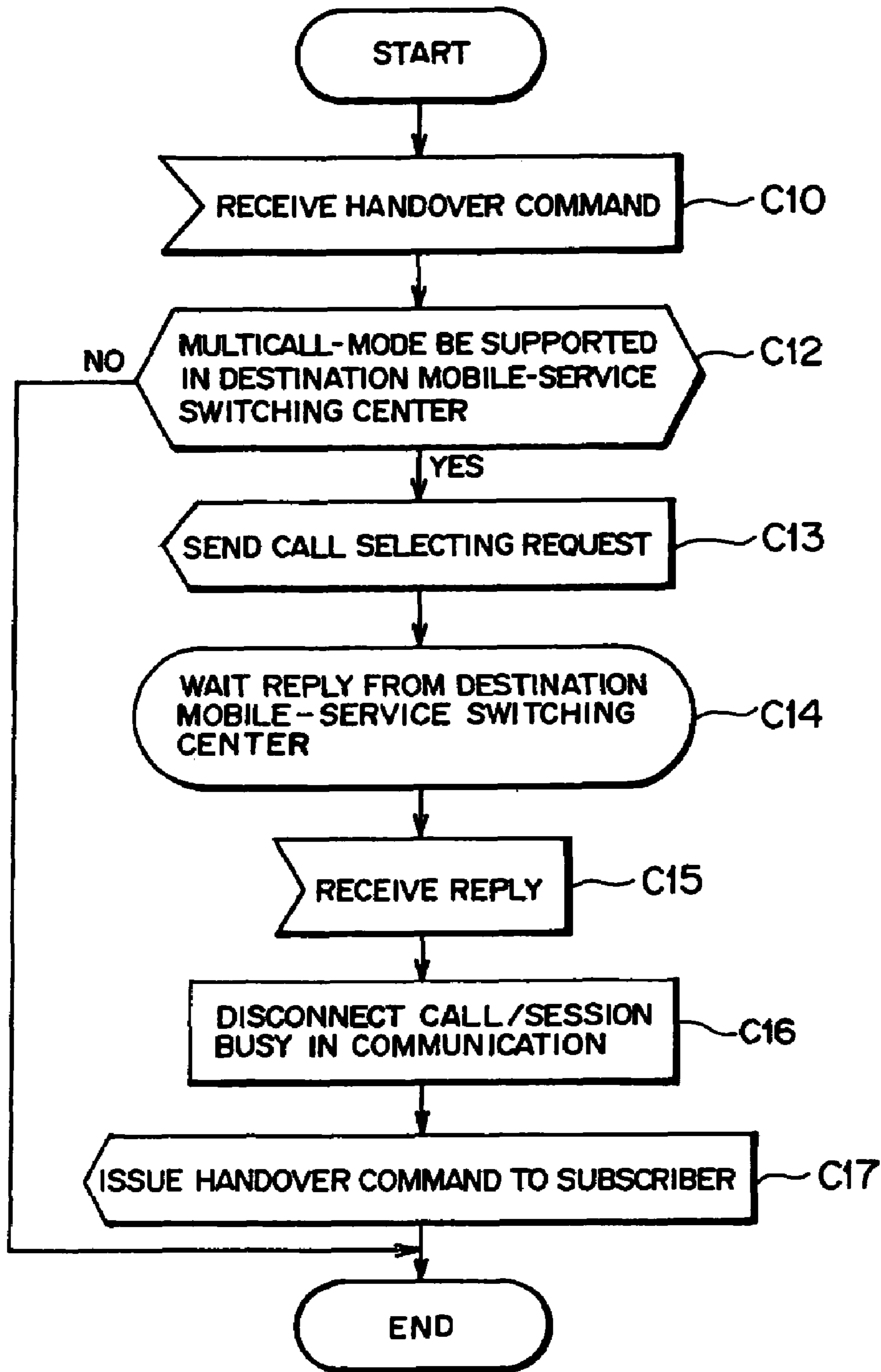
EXAMPLE OF PROCESSING EFFECTED IN BASE STATION CONTROLLER ON HANDOVER SOURCE SIDE
