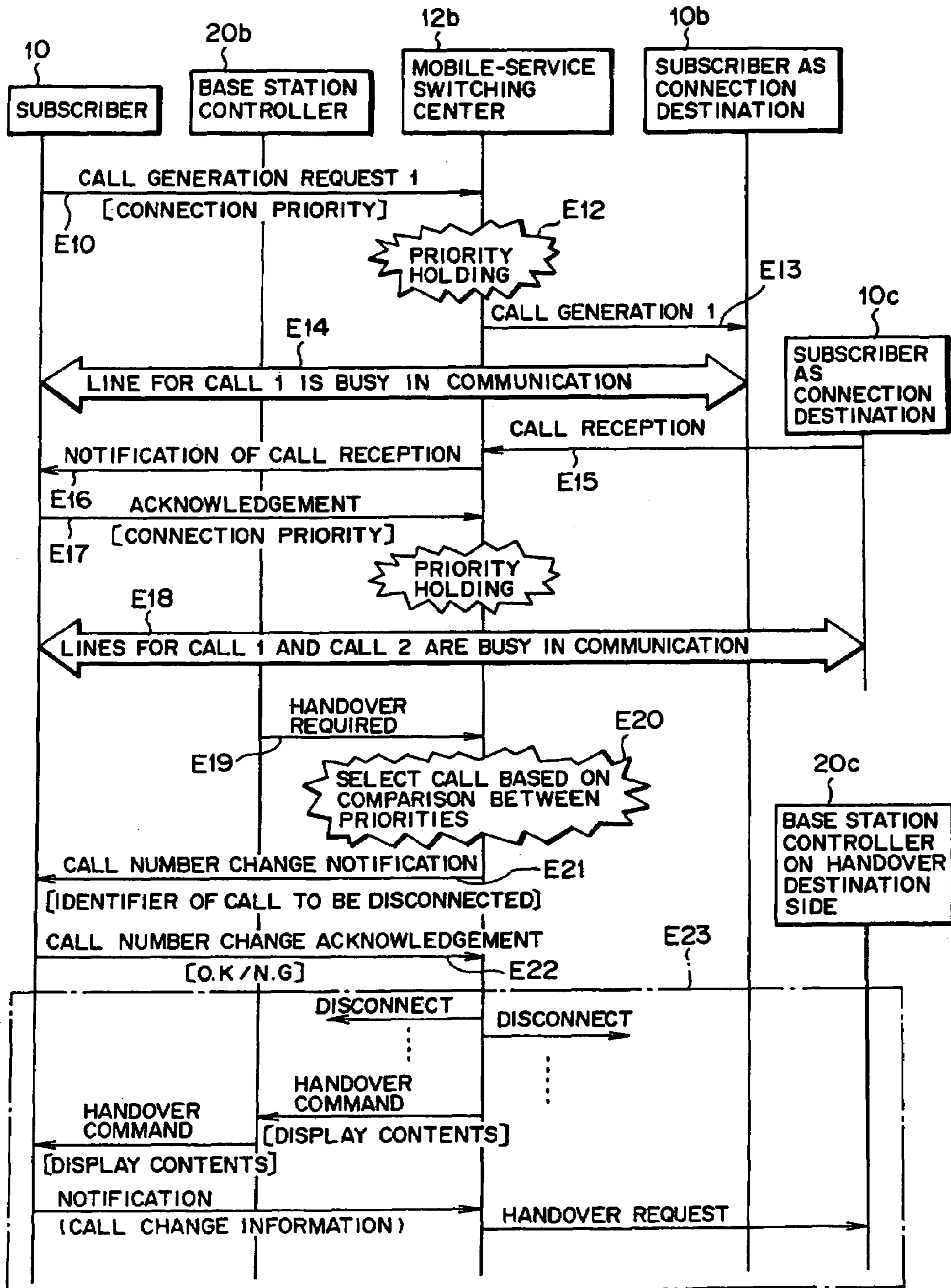
EXAMPLE OF SIGNALING SEQUENCE
