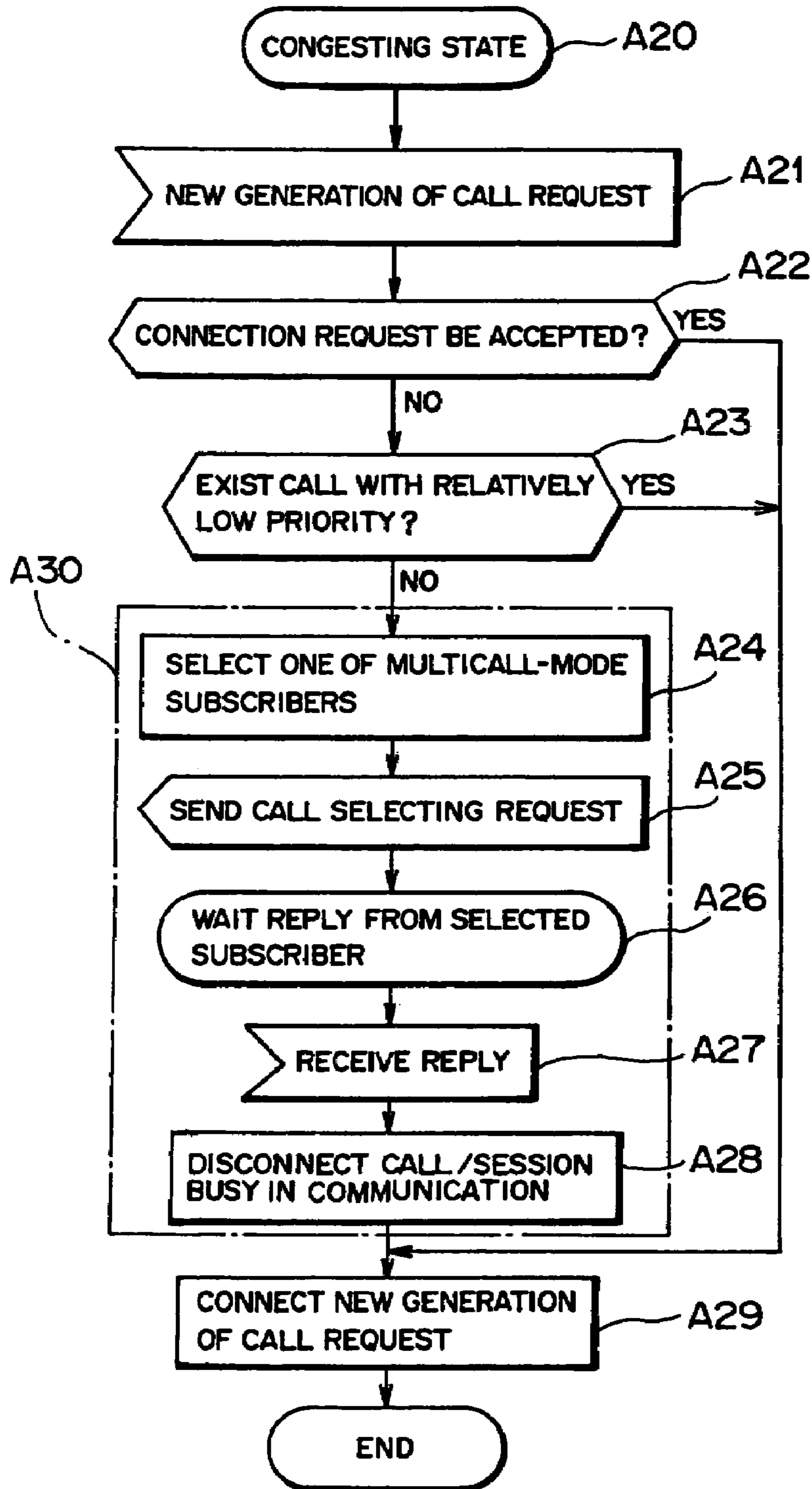
EXAMPLE OF PROCESSING EFFECTED ON THE SIDE OF MOBILE-SERVICE SWITCHING CENTER
