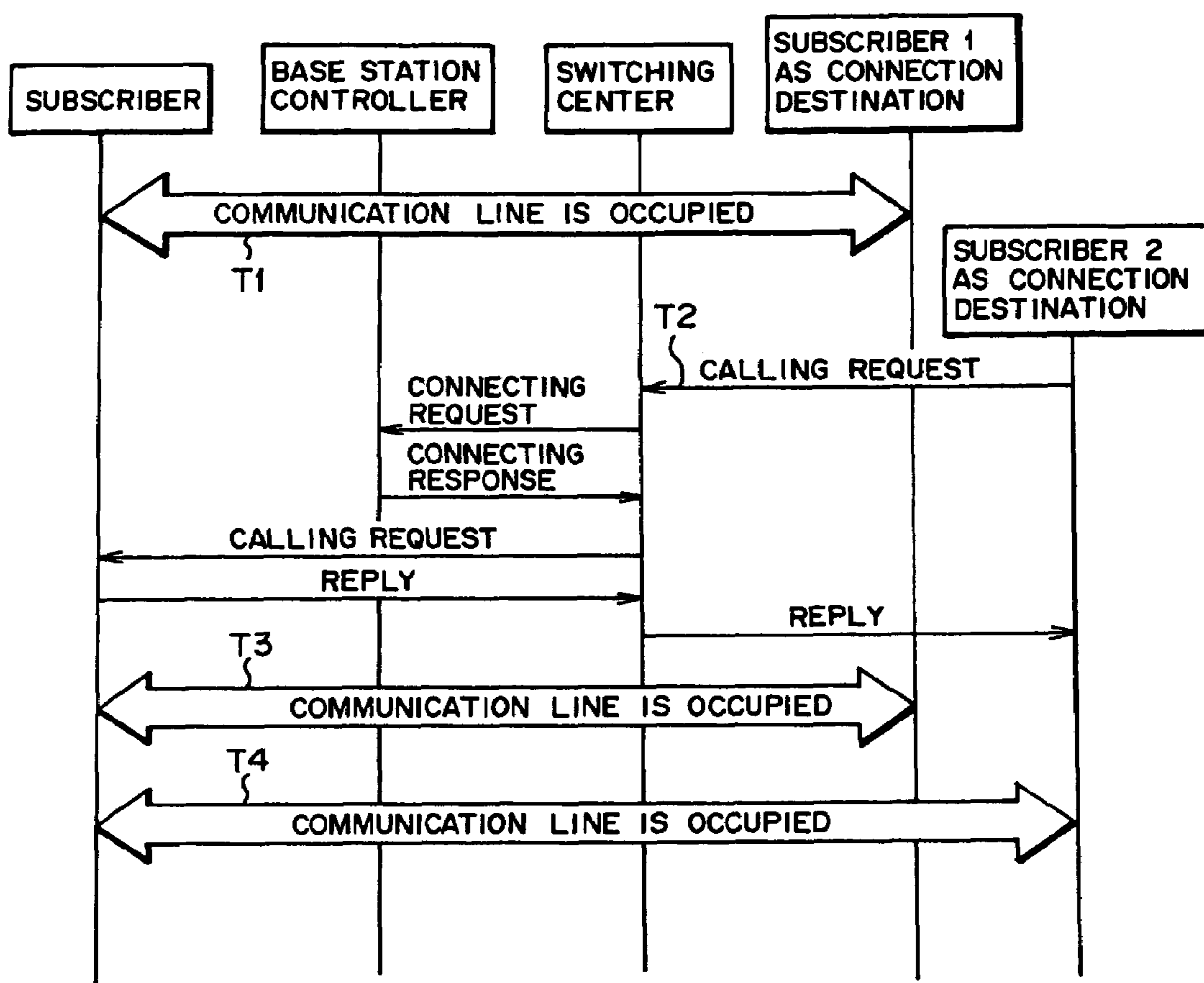
EXAMPLE OF CONNECTION SEQUENCE OF MULTI-SESSION (MULTICALL)
