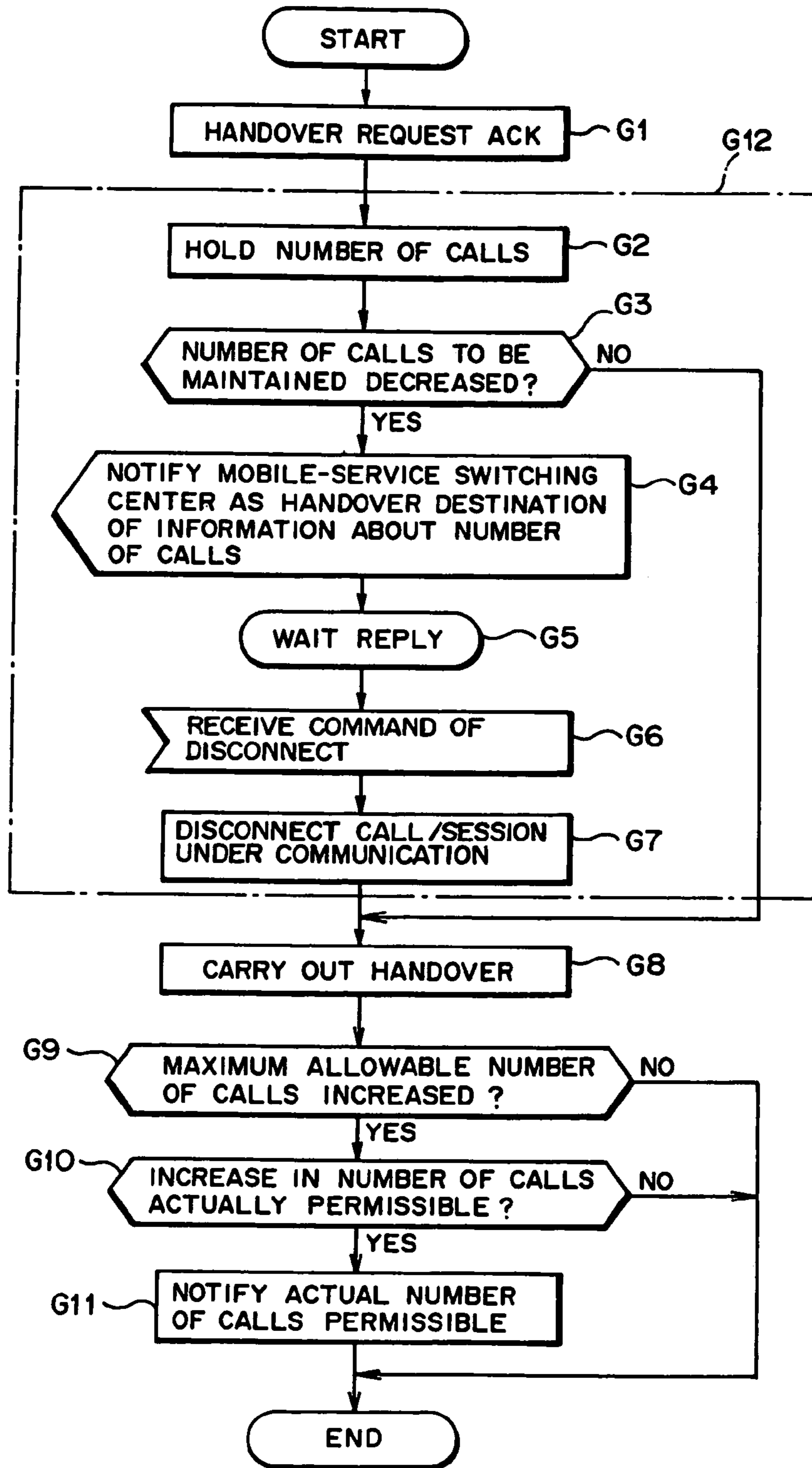
EXAMPLE OF PROCESSING EFFECTED IN MOBILE-SERVICE SWITCHING CENTER AS SOURCE OF HANDOVER
