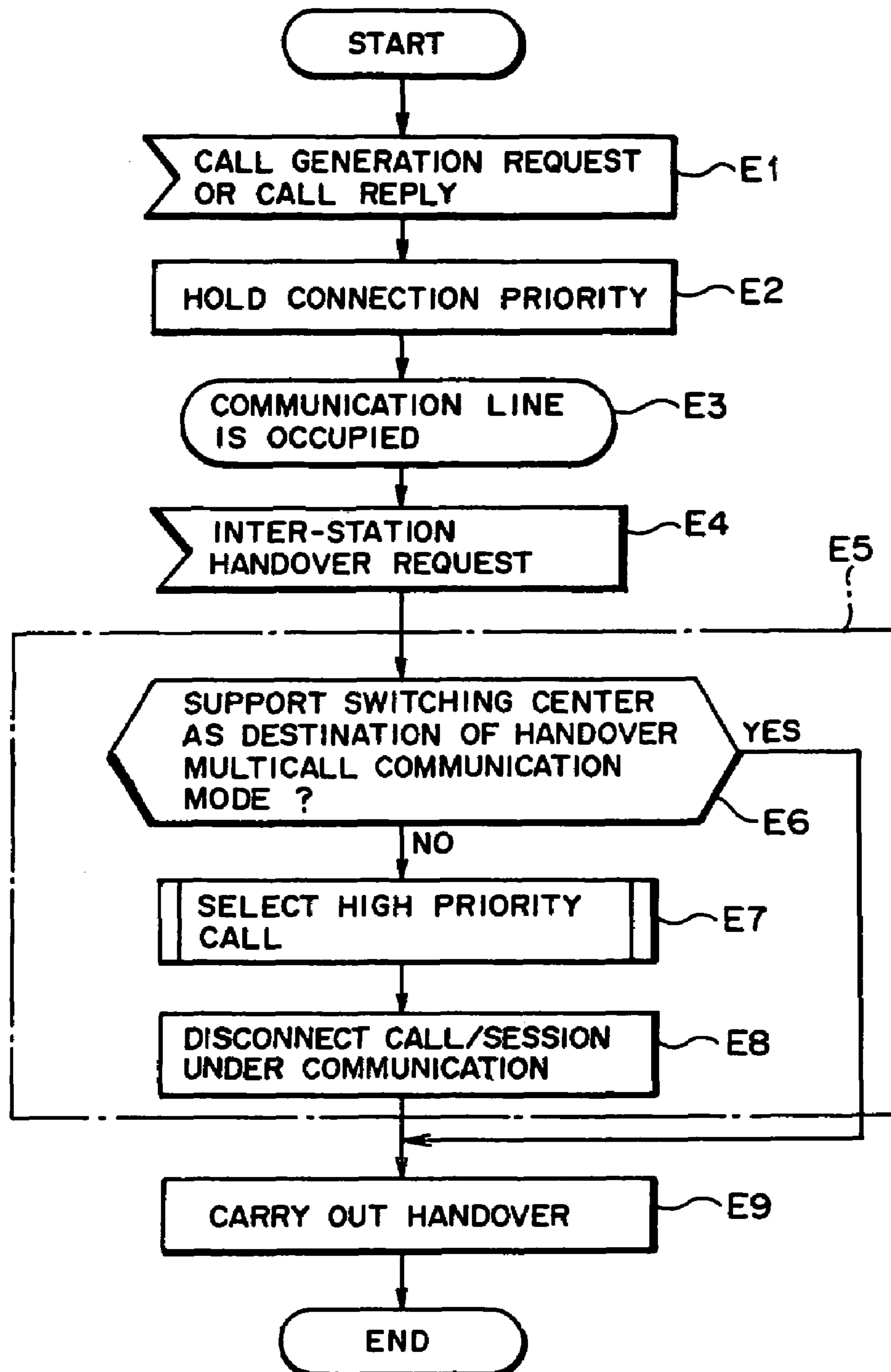
EXAMPLE OF PROCESSING EFFECTED IN SWITCHING CENTER
