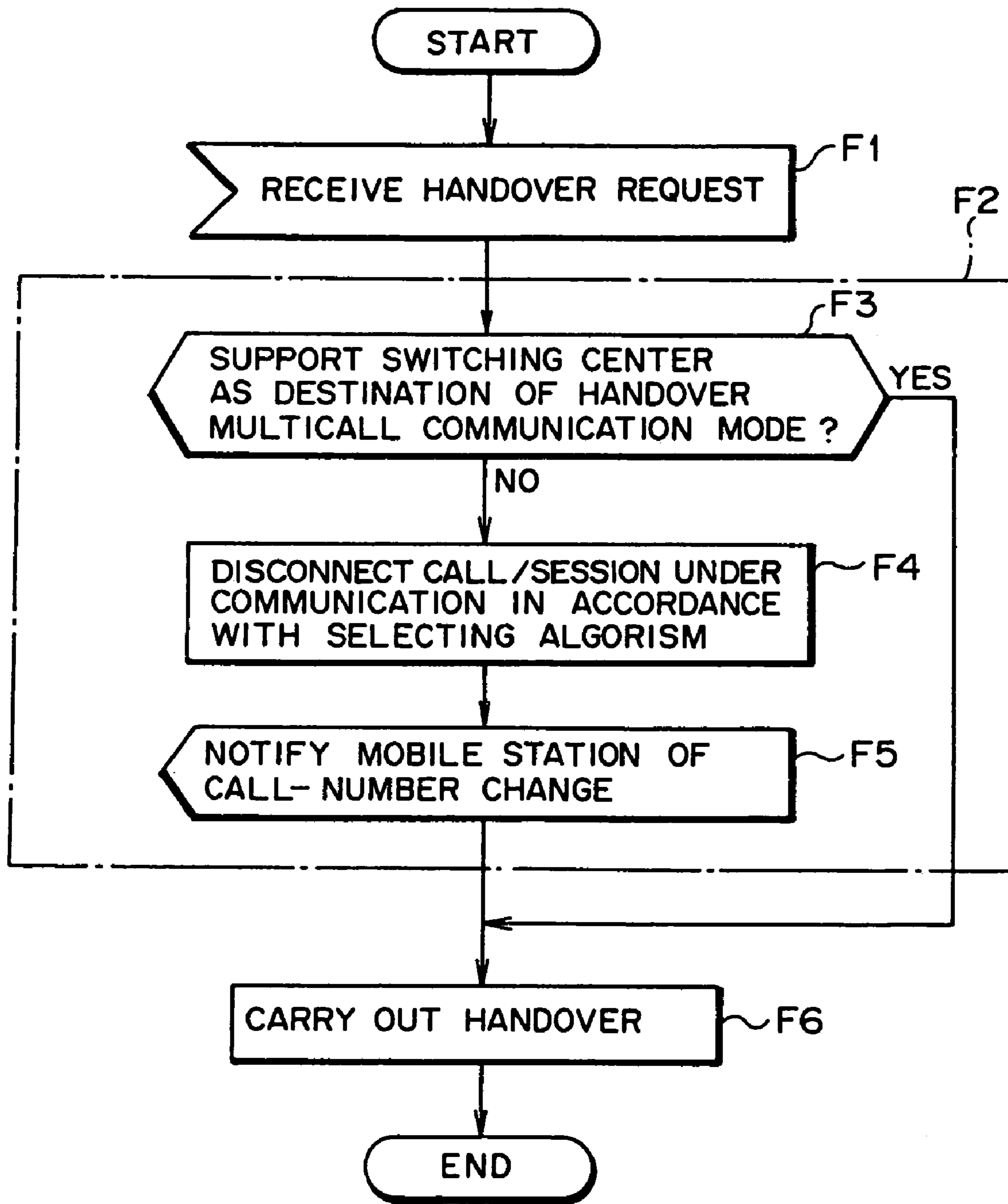
EXAMPLE OF PROCESSING EFFECTED IN SWITCHING CENTER
