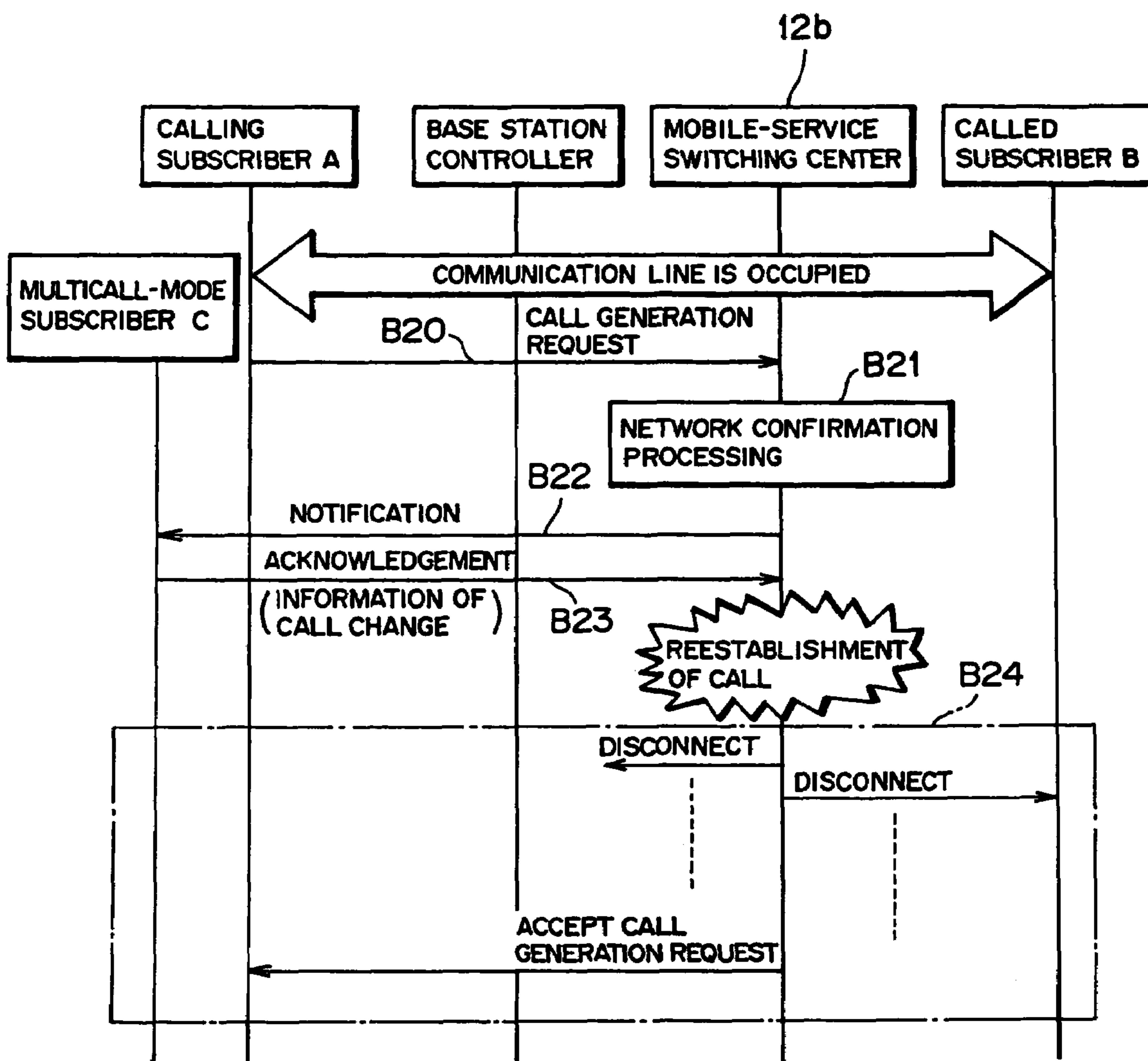
EXAMPLE OF SIGNALING SEQUENCE
