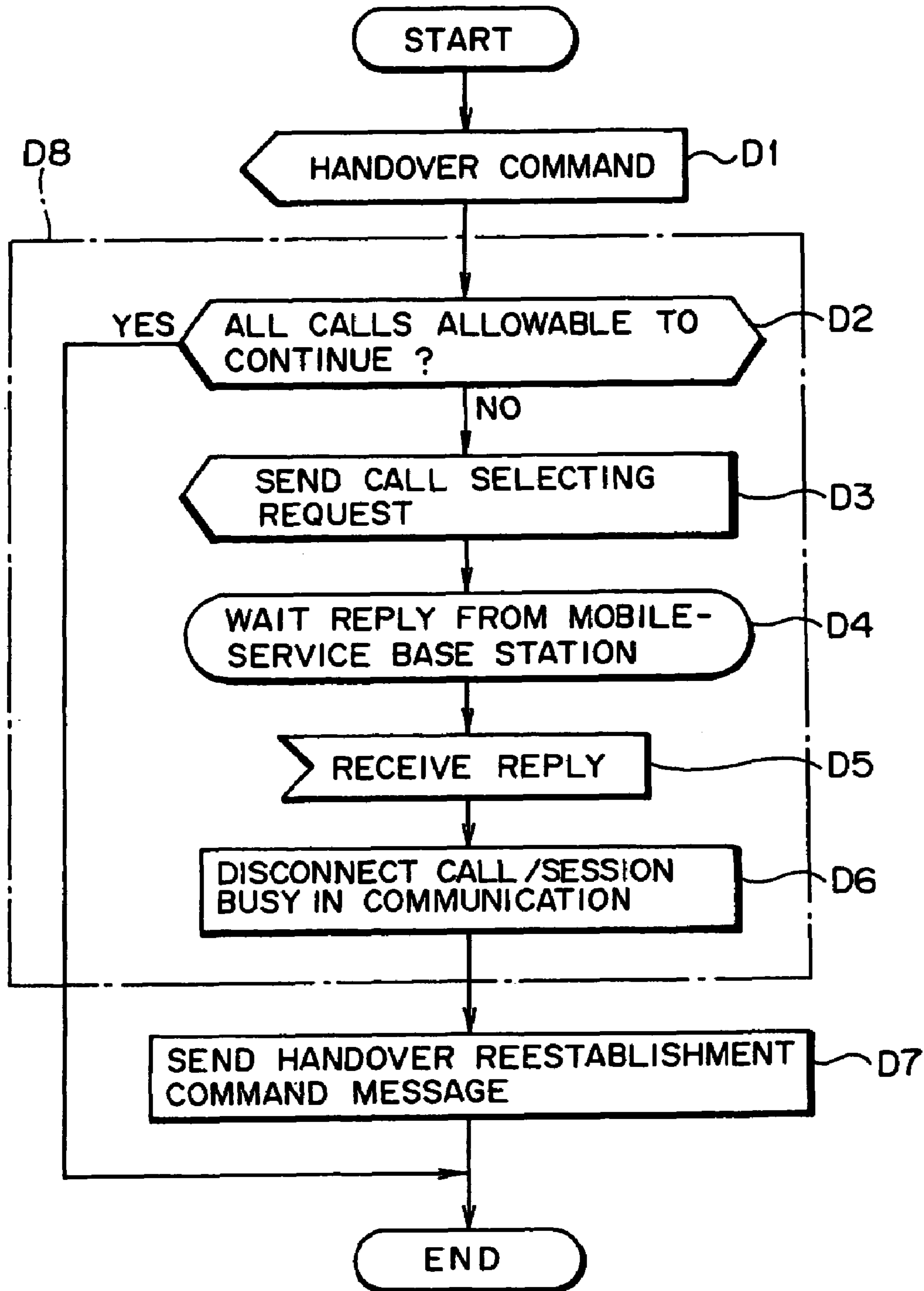
EXAMPLE OF PROCESSING EFFECTED ON THE SIDE OF MOBILE-SERVICE SWITCHING CENTER
