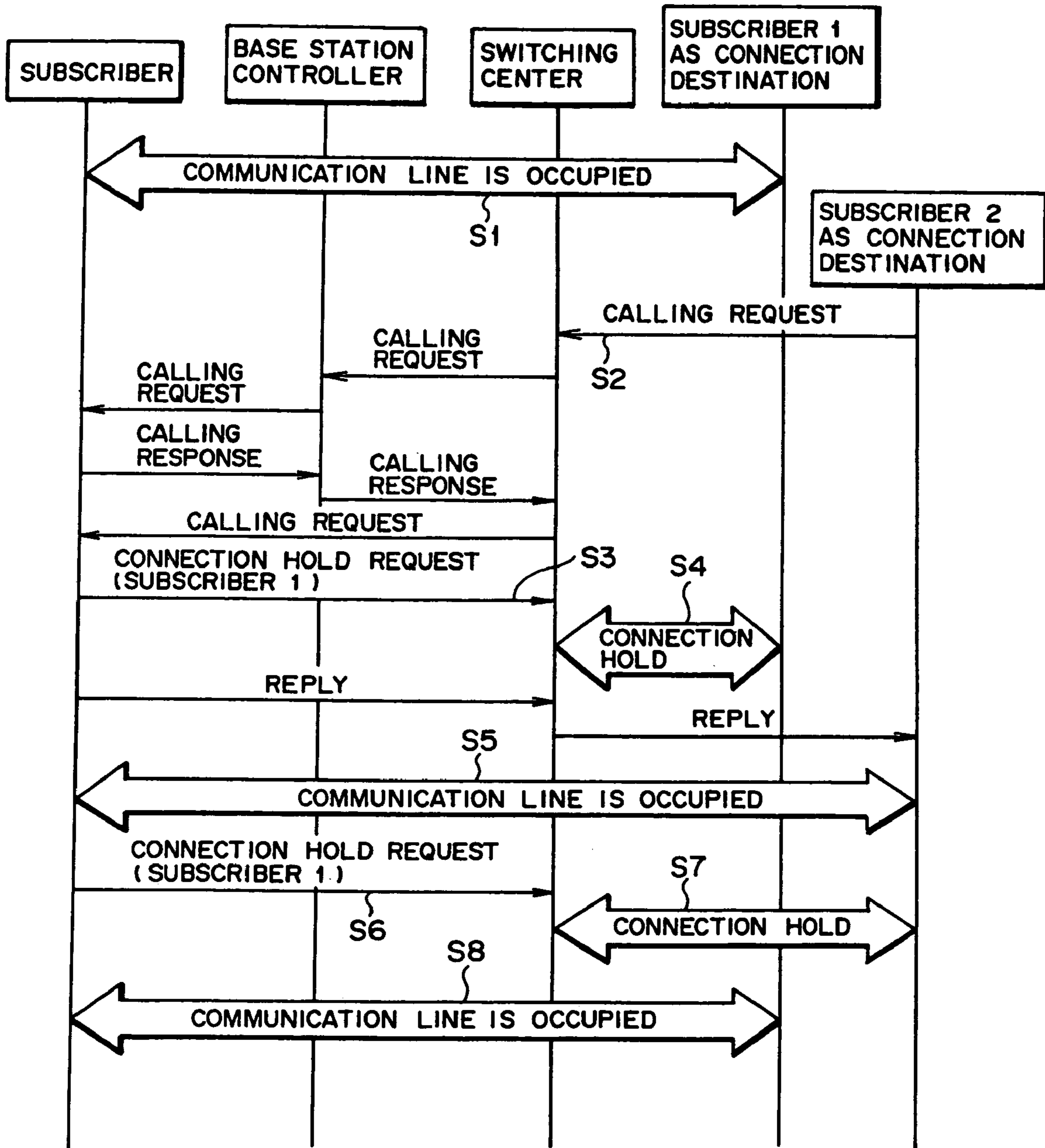
EXAMPLE OF CONNECTION SEQUENCE OF CATCH PHONE
