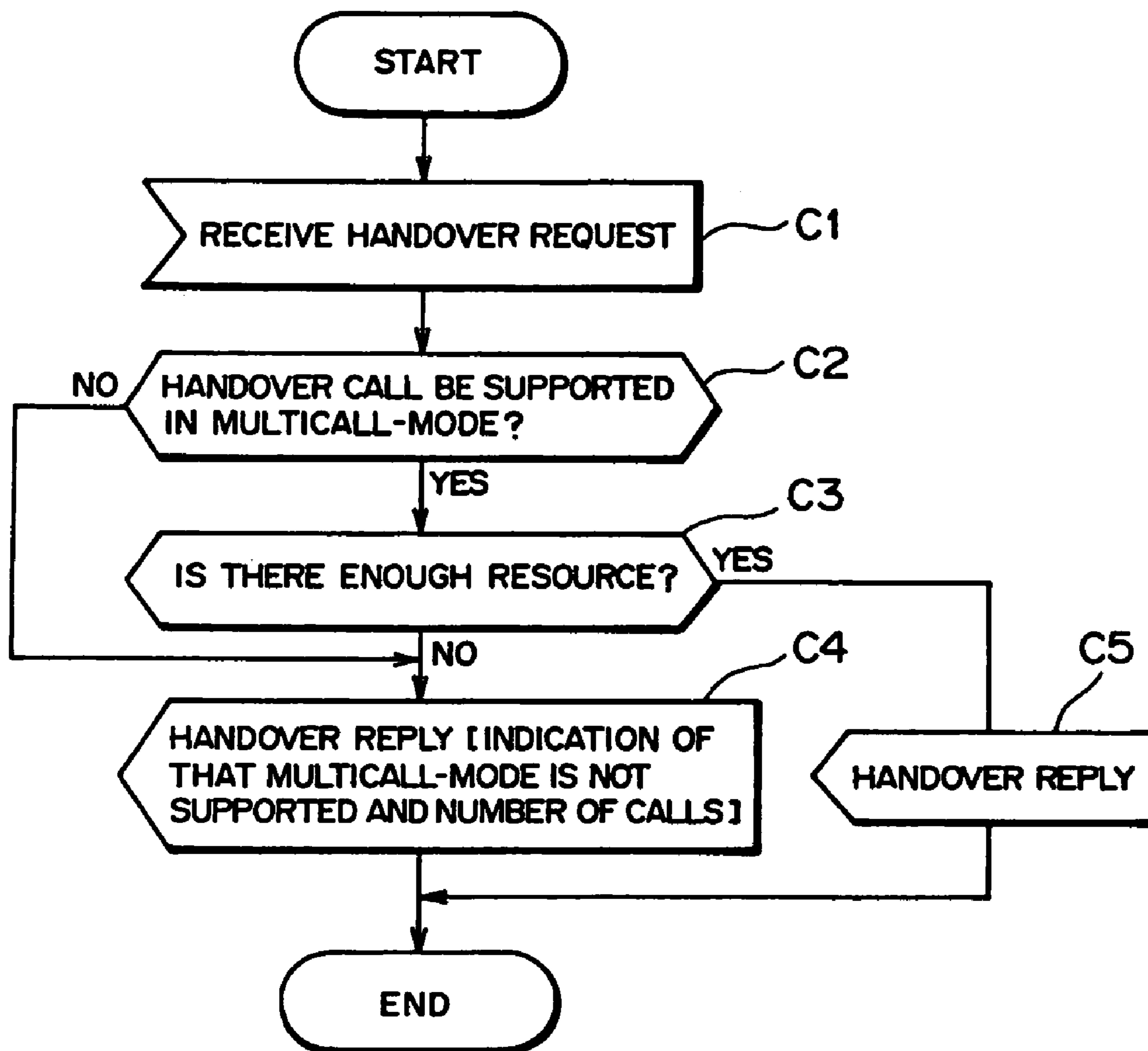
EXAMPLE OF PROCESSING EFFECTED IN BASE STATION CONTROLLER ON HANDOVER DISTINATION SIDE
