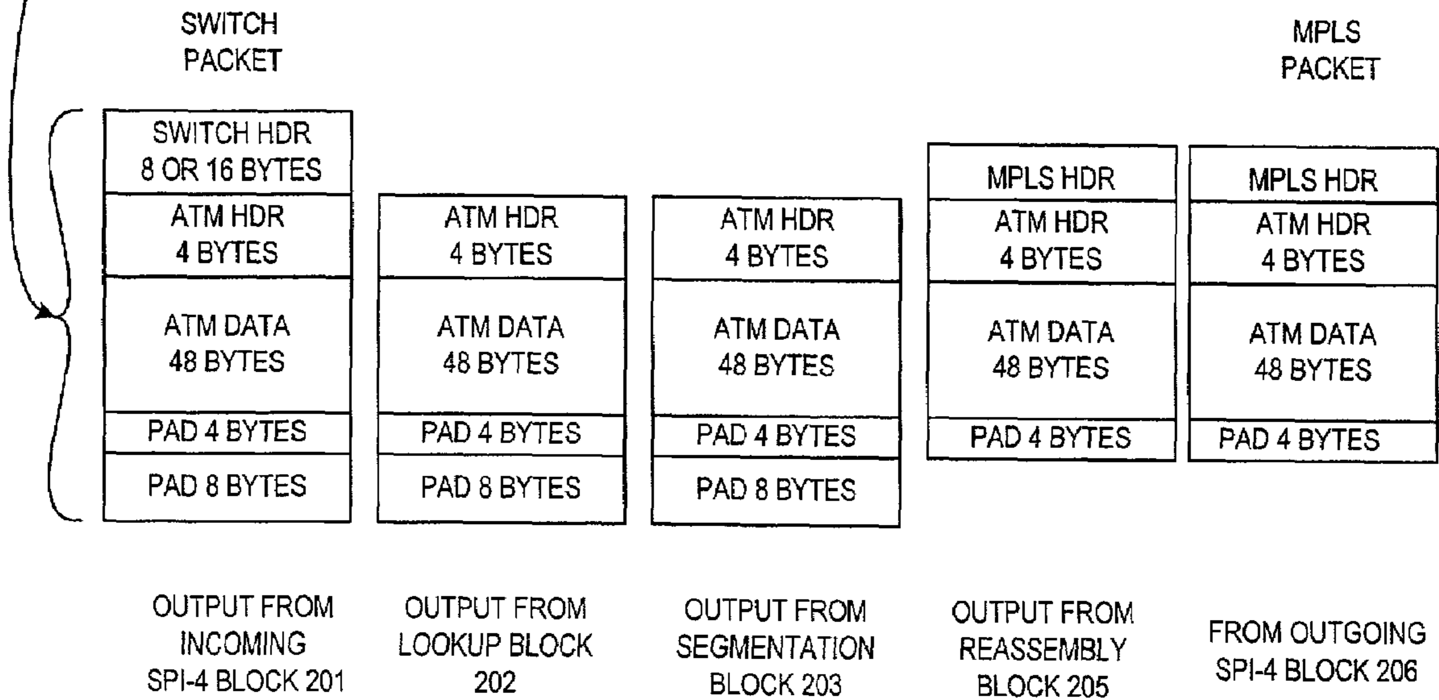
EGRESS APPLICATION TYPE 14
