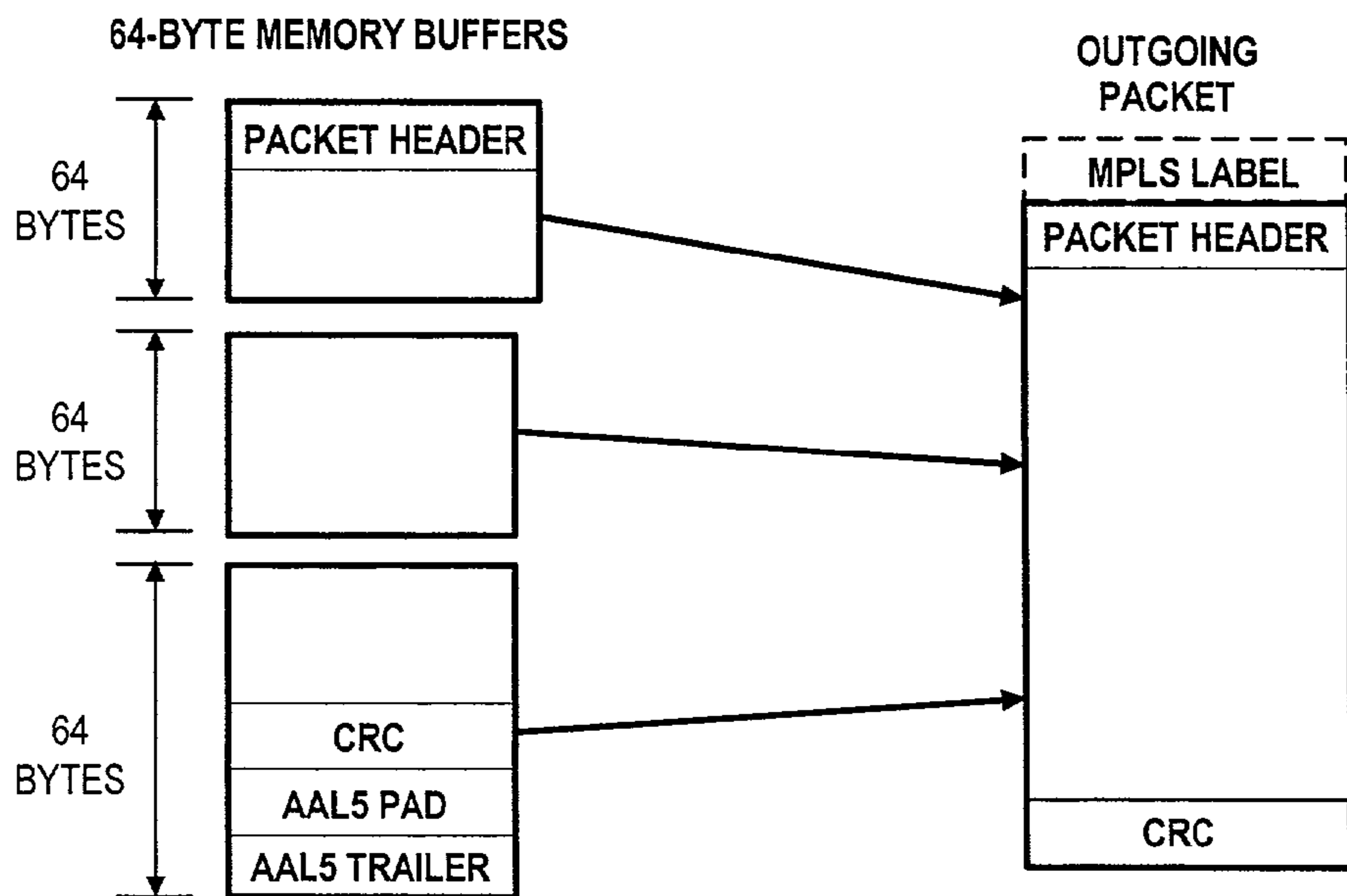
REASSEMBLY TYPE 8 (INGRESS APPLICATION TYPES 11 AND 14)
