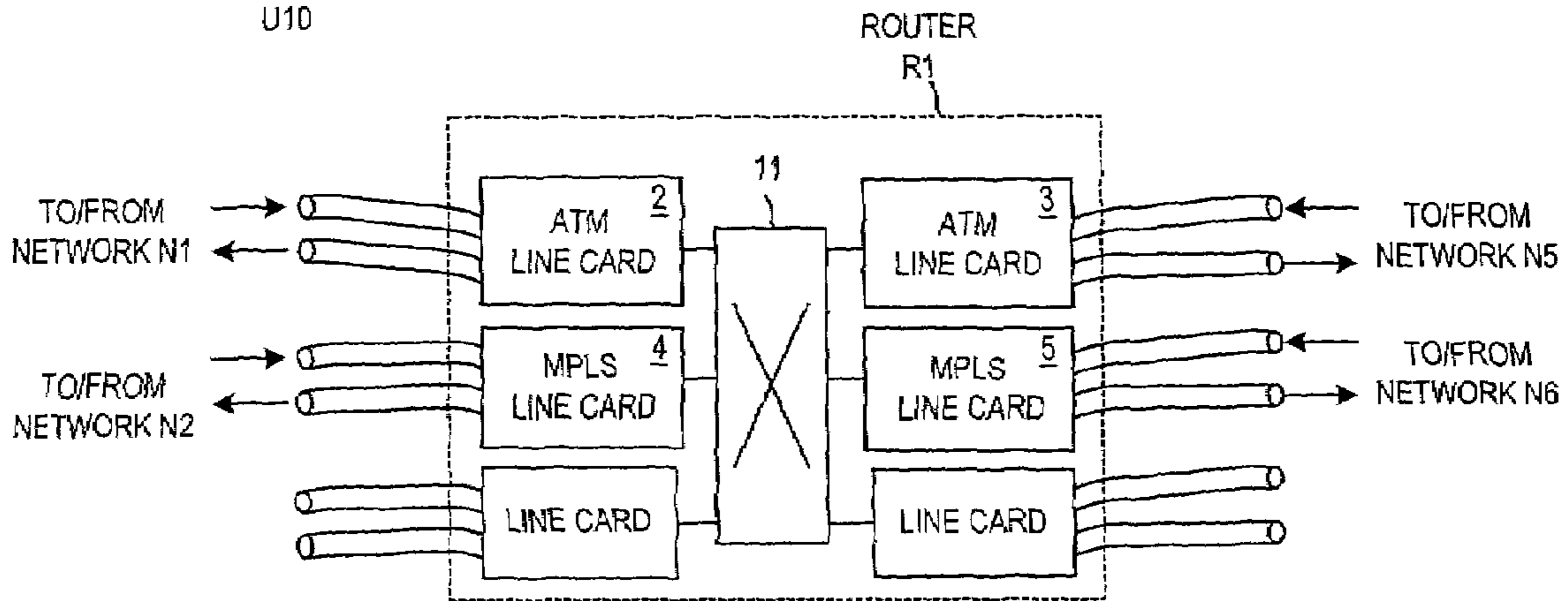
FIG. 2 (PRIOR ART)
