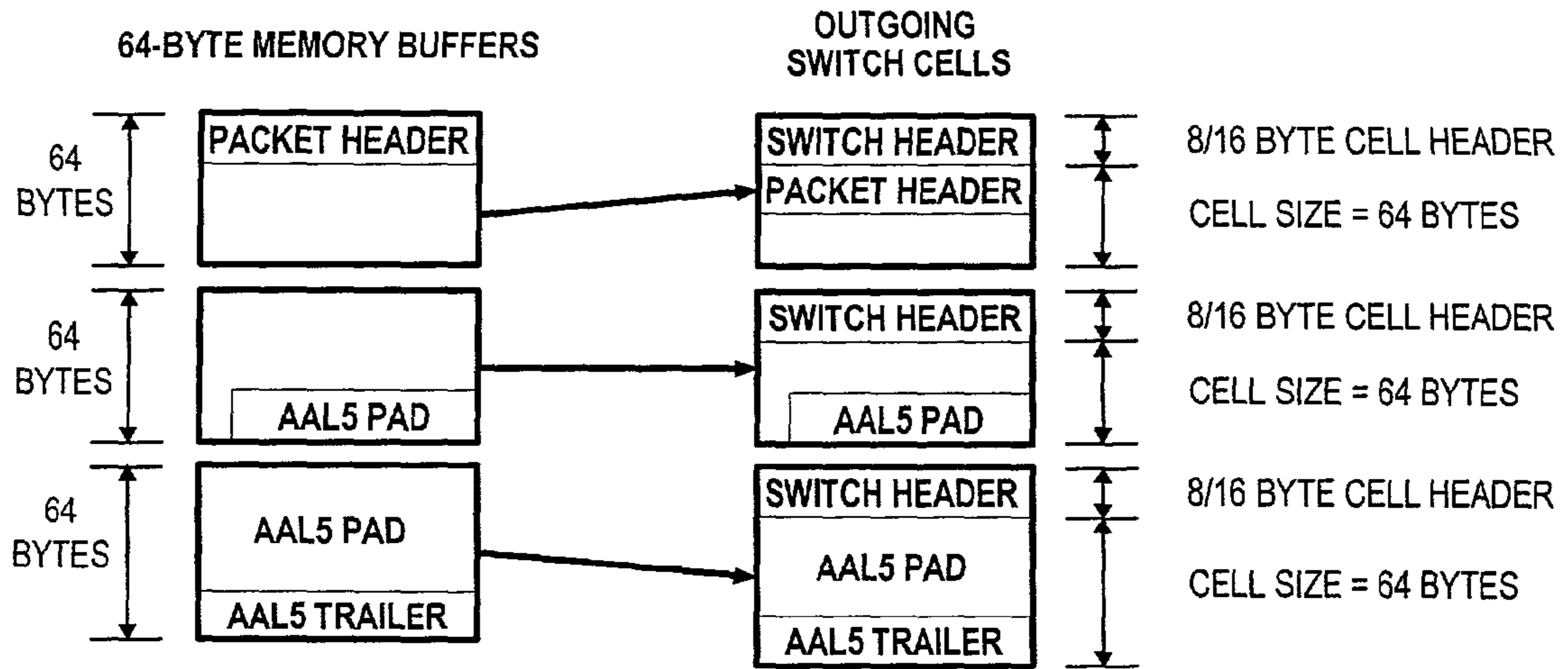
REASSEMBLY TYPE 1 (INGRESS APPLICATION TYPE 3)
