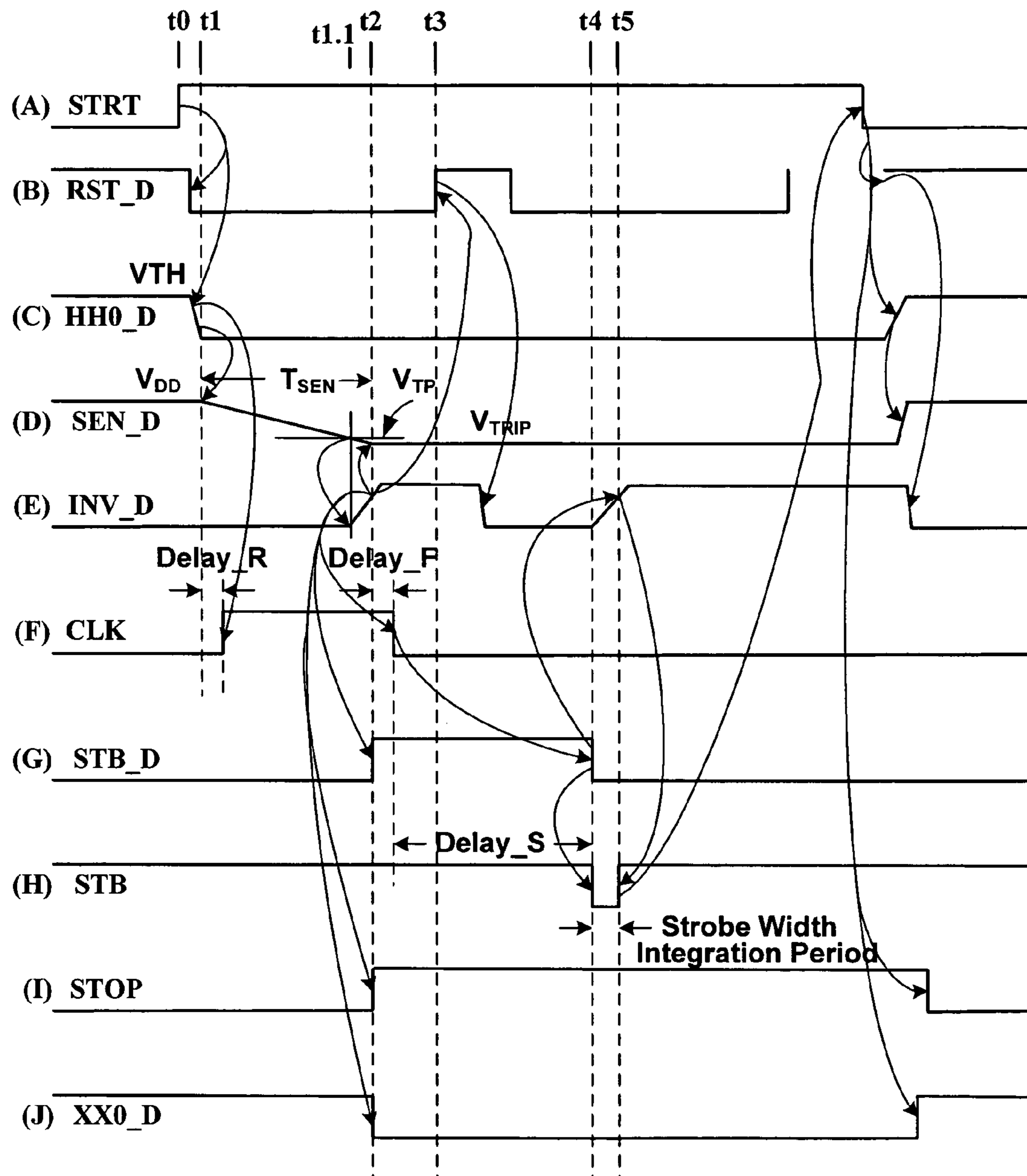
Reference Sense Amplifier's Timing Diagrams
