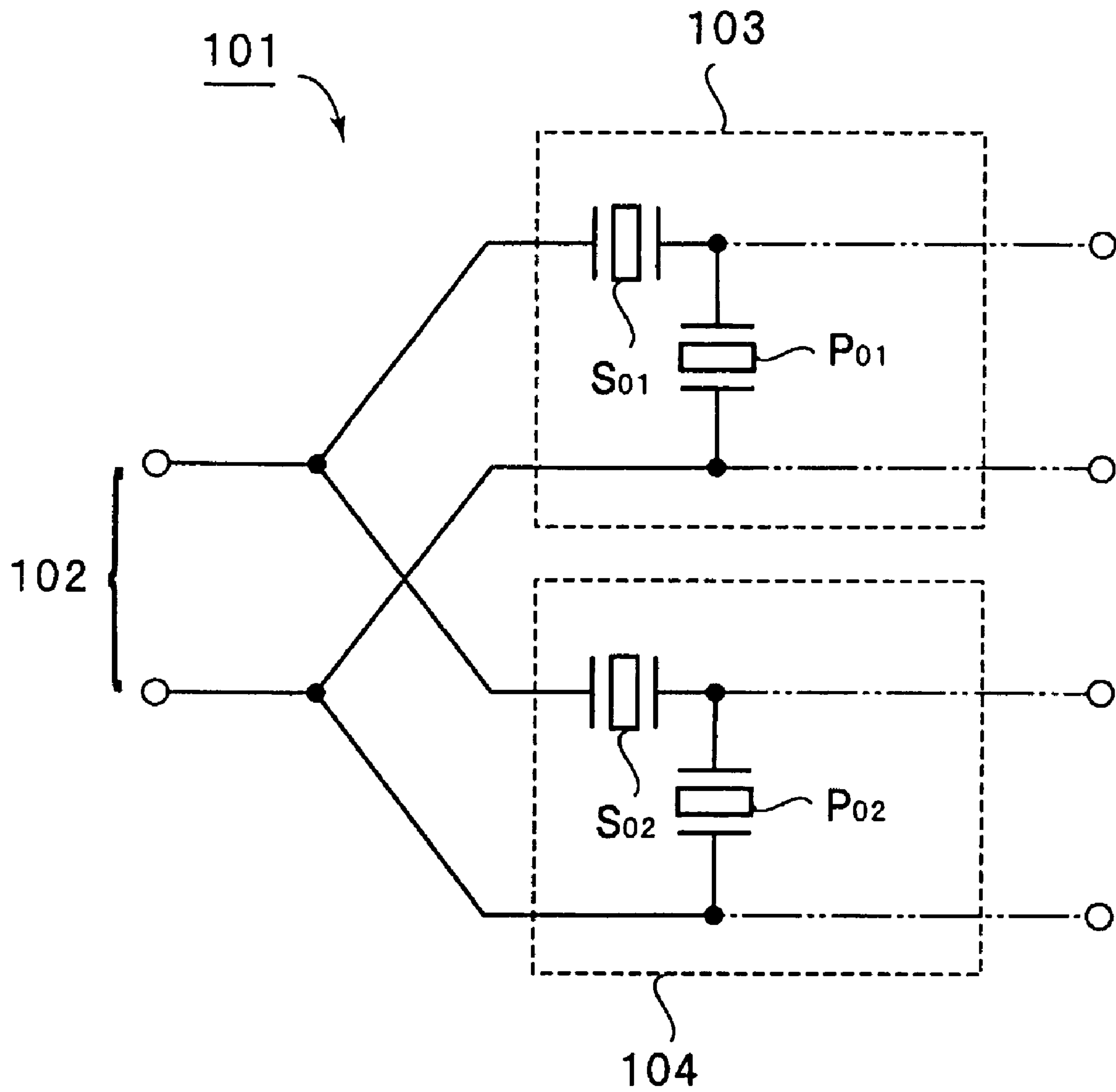
FIG. 17 PRIOR ART
