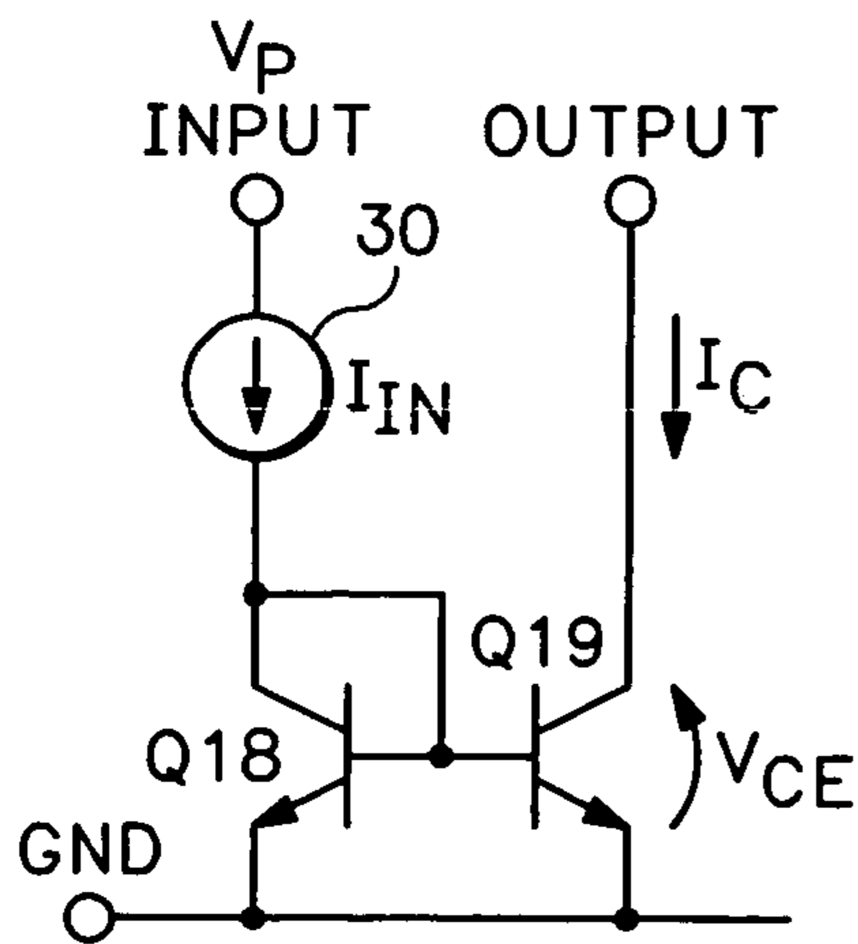
FIG. 16 (PRIOR ART)
