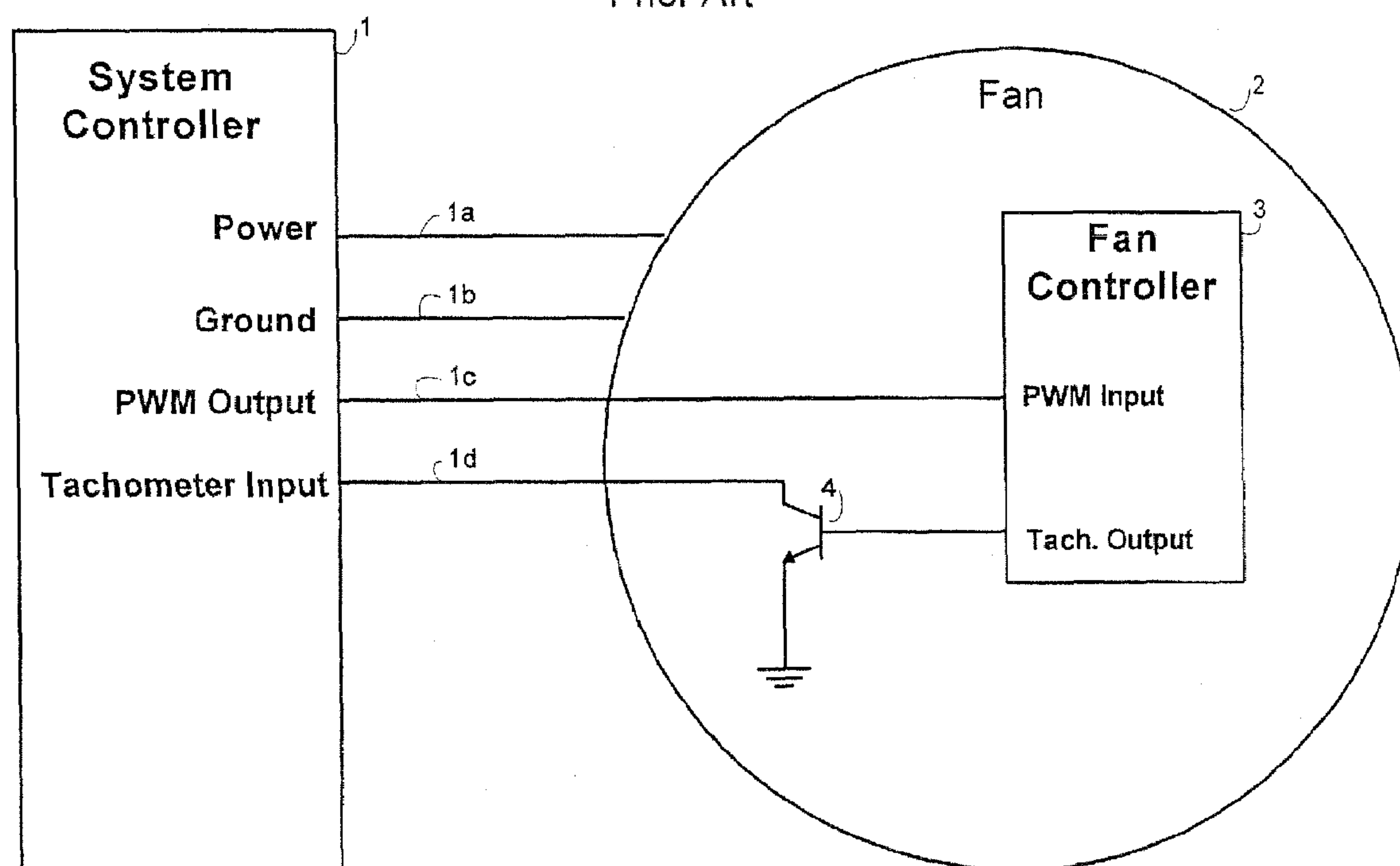
Figure 1 Prior Art
