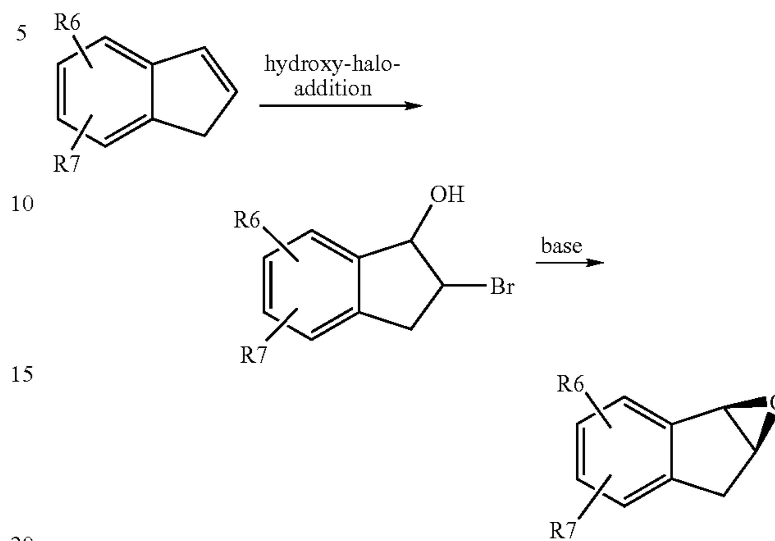
Scheme 1: Preparation of substituted epoxyindanes
