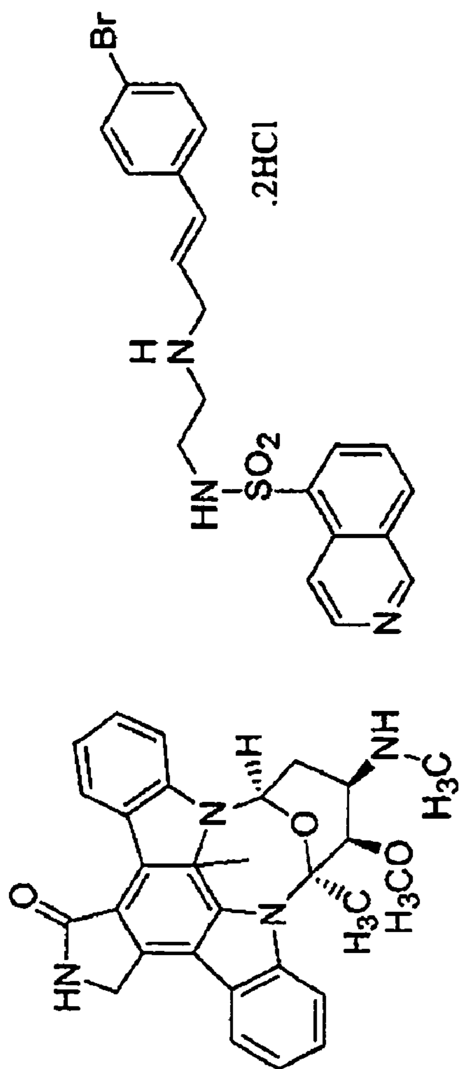
Staurosporine H-89
