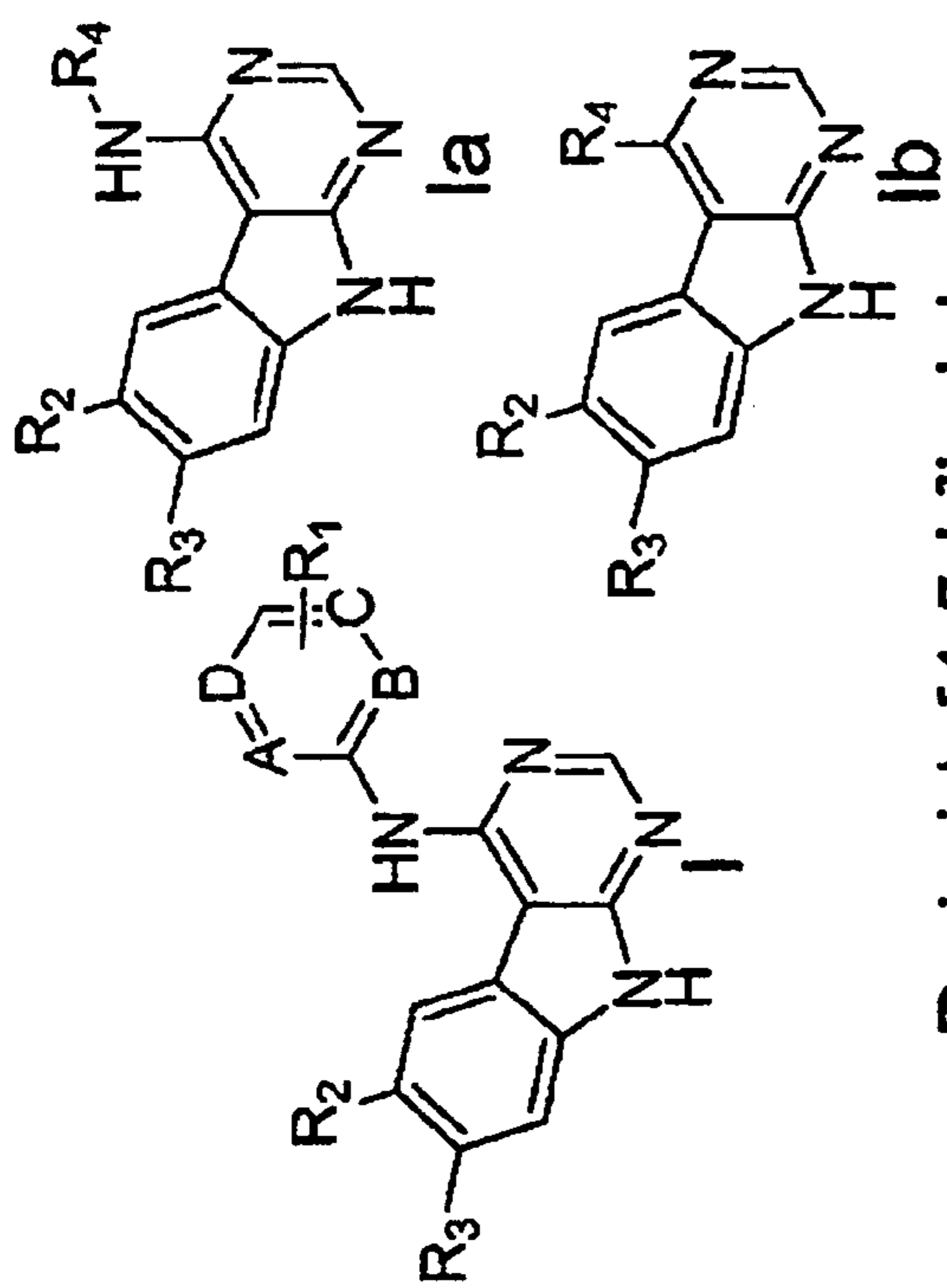
Benzothieno[3,2-d]pyrimidones
