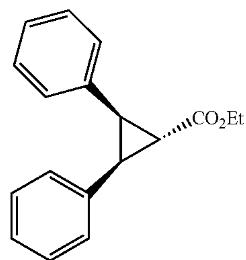
Ethyl 2,3-cis-diphenylcyclopropane carboxylate
