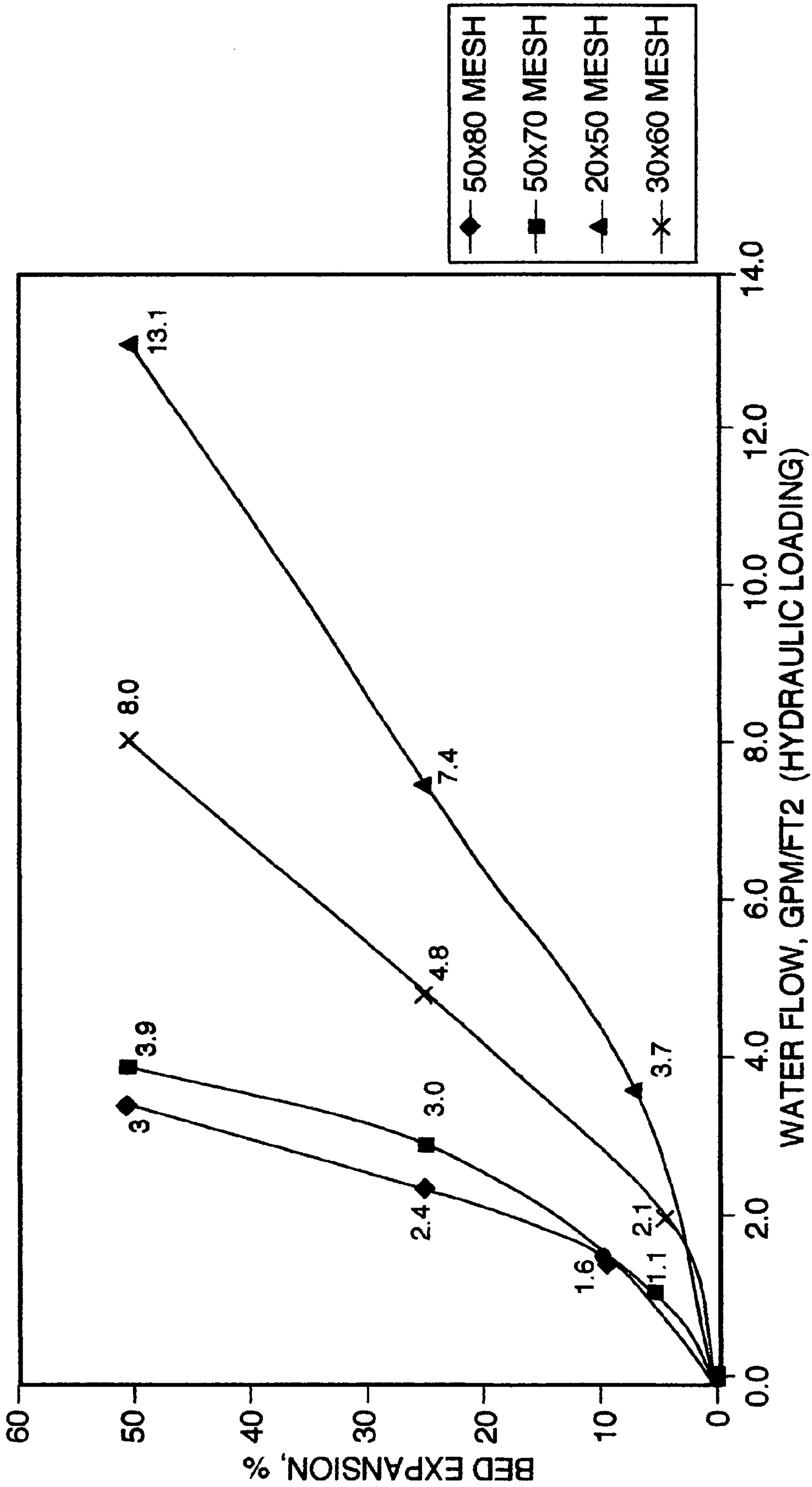
BED EXPANSION DATA ON ROTAP SIZE COMPOSITES
