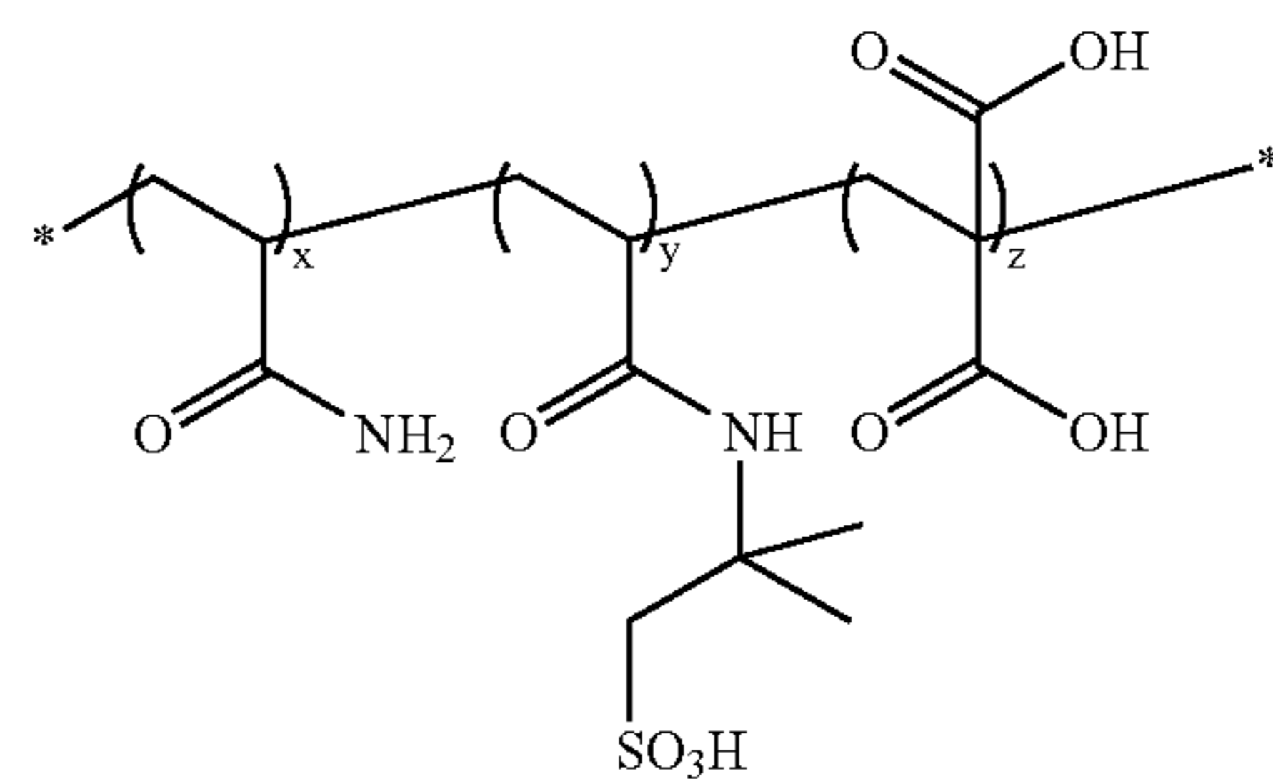
Poly(acrylamide-co-AMPS-co-maleic acid)
