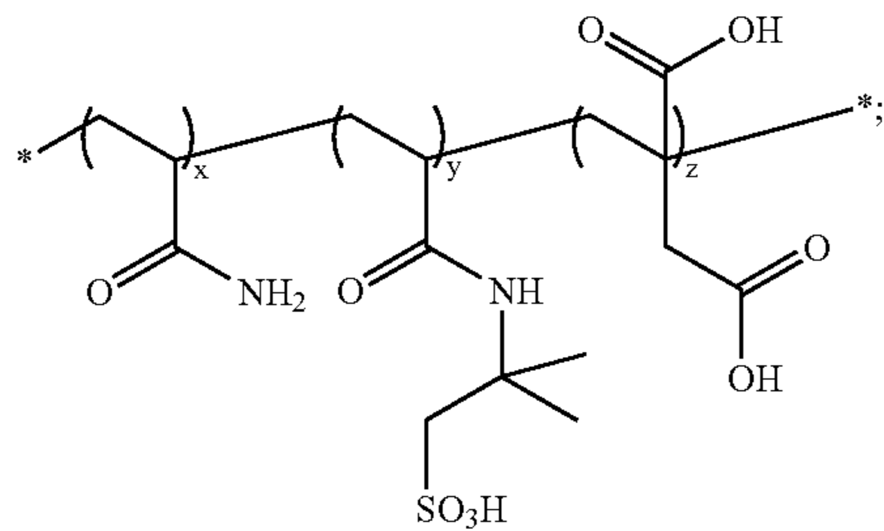
Poly(acrylamide-co-AMPS-co-itaconic acid)
