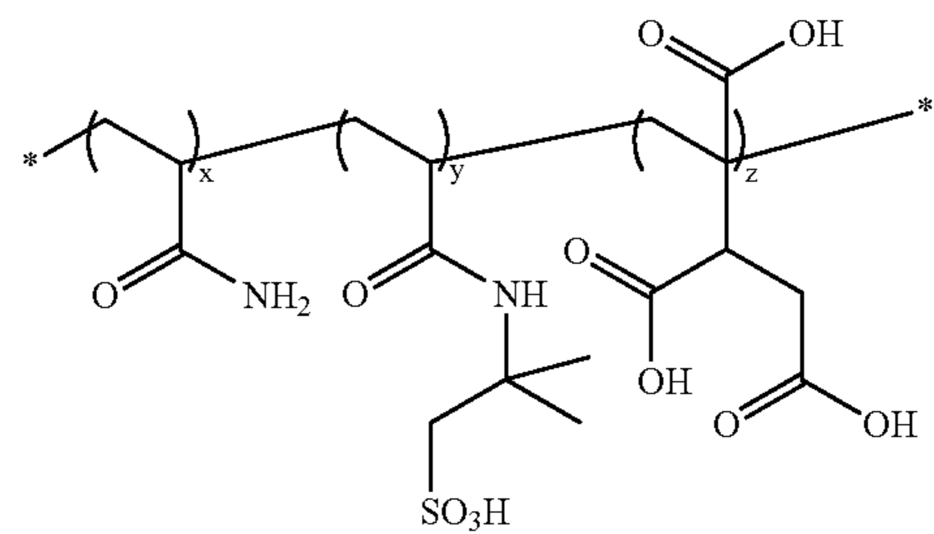
Poly(acrylamide-co-AMPS-co-butenetricarboxylic acid)
