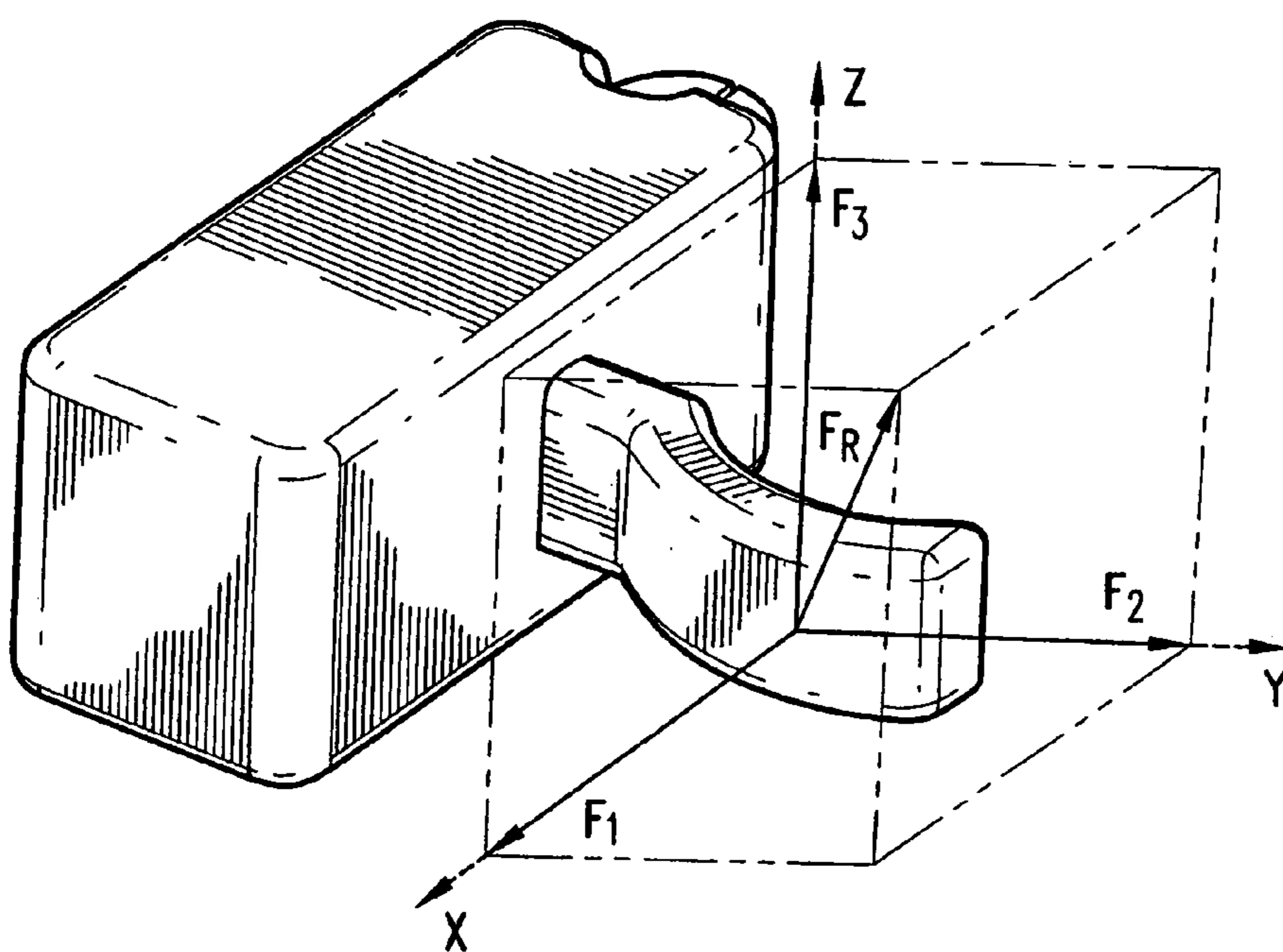
FIG. 1 PRIOR ART
