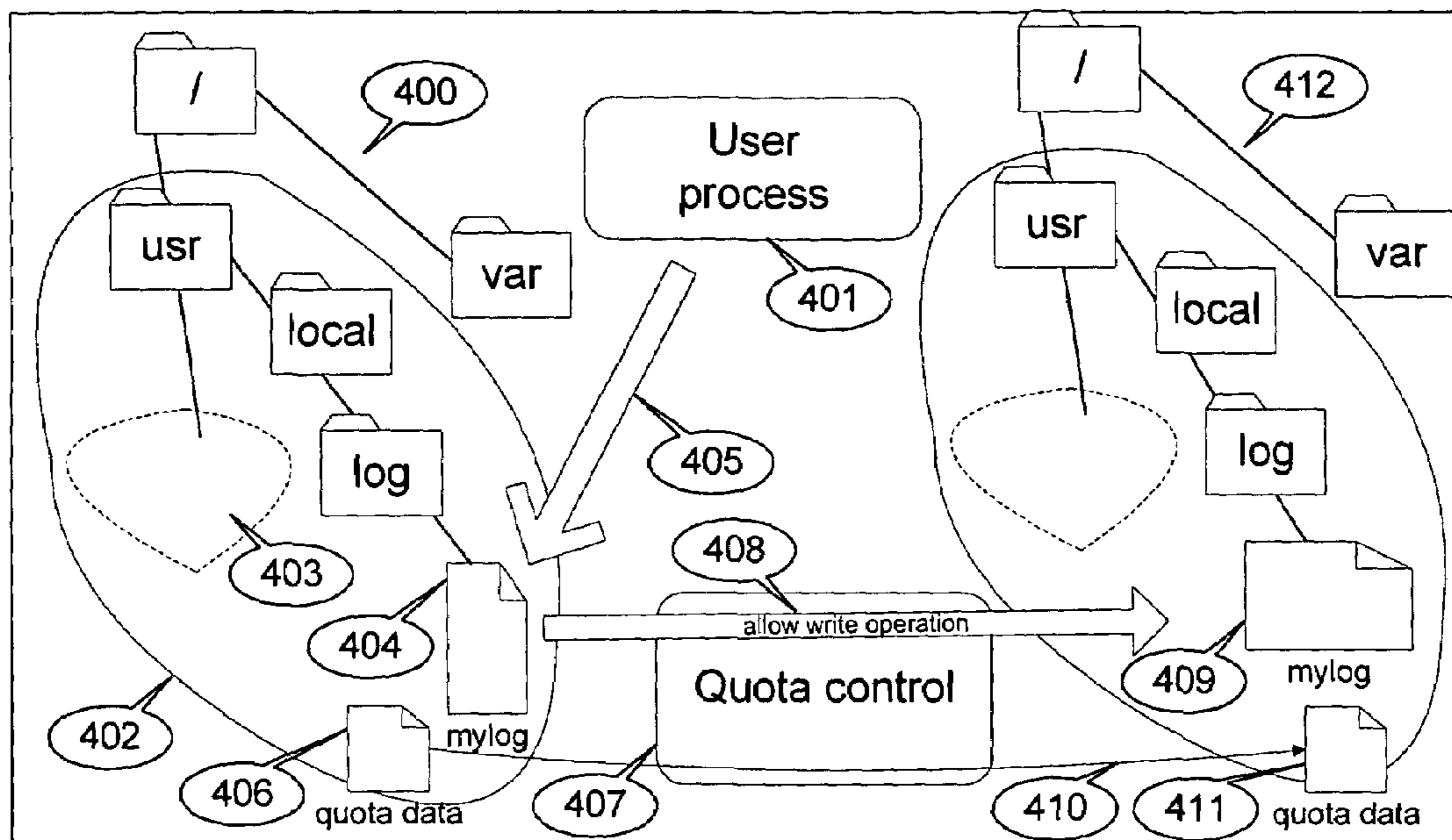
Process of alteration of space size occupied by the file taking into account a quota on the reserved resources
