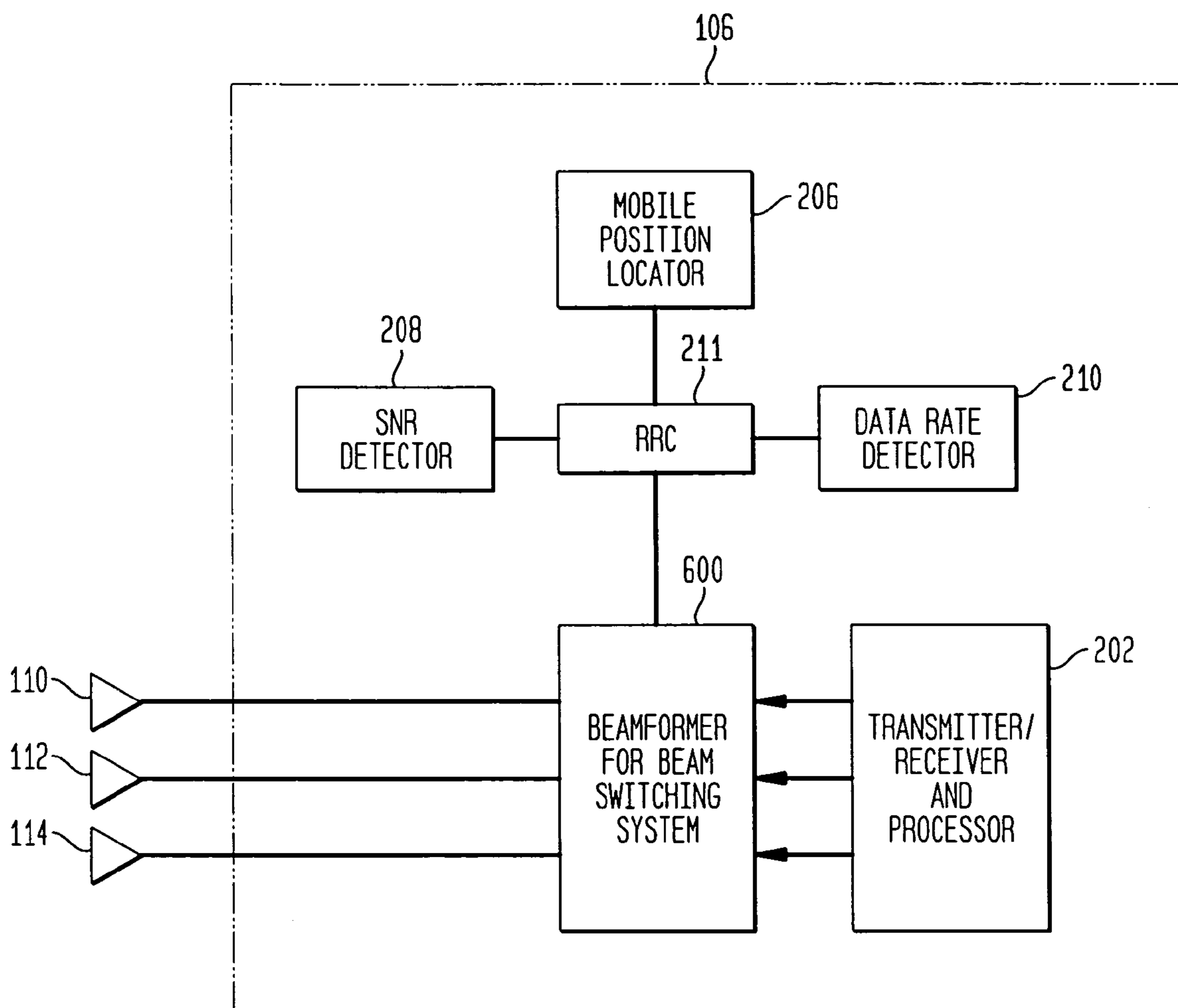
TRANSCEIVER SYSTEM AT A BASE STATION
