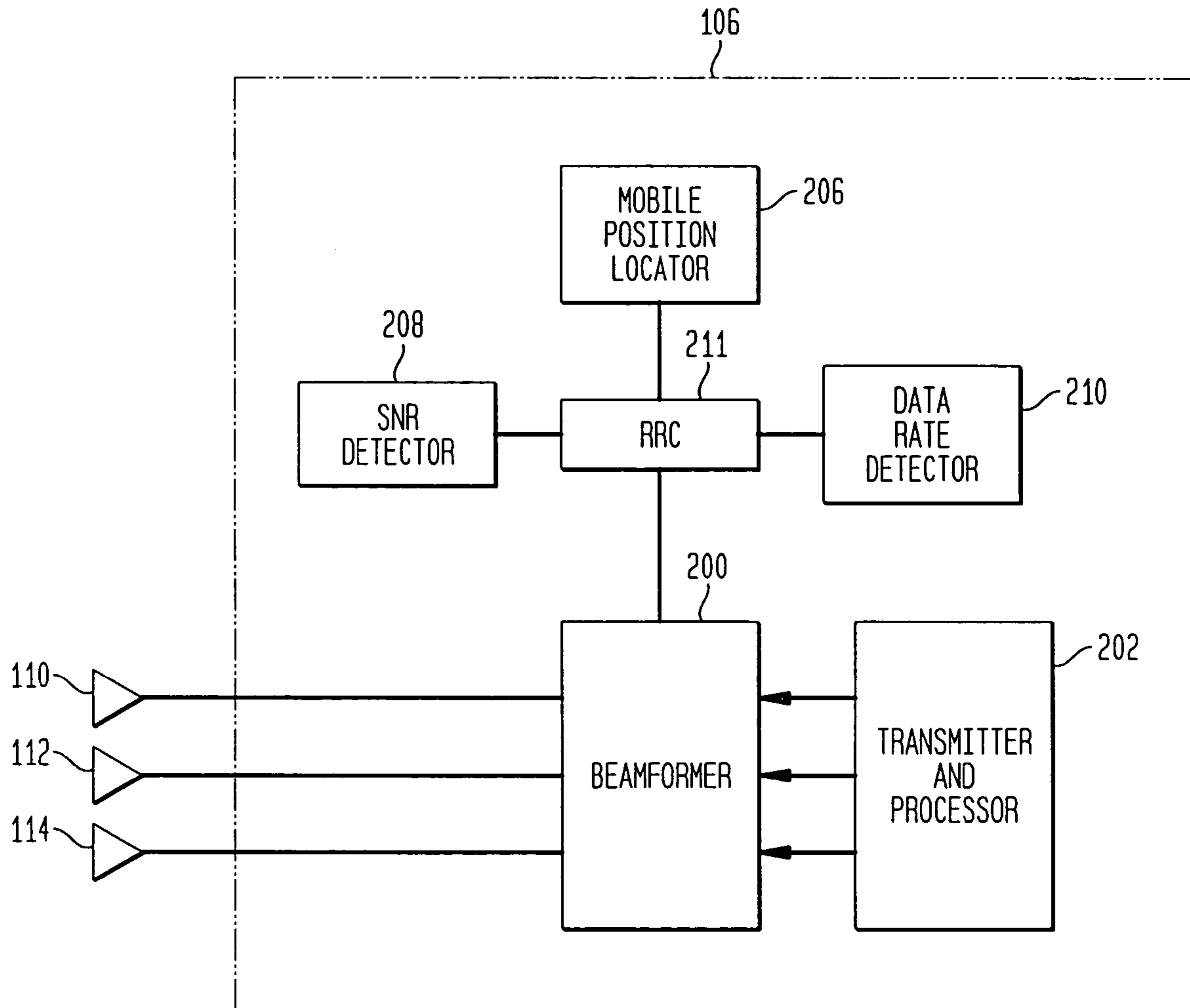
TRANSMIT SYSTEM AT A BASE STATION
