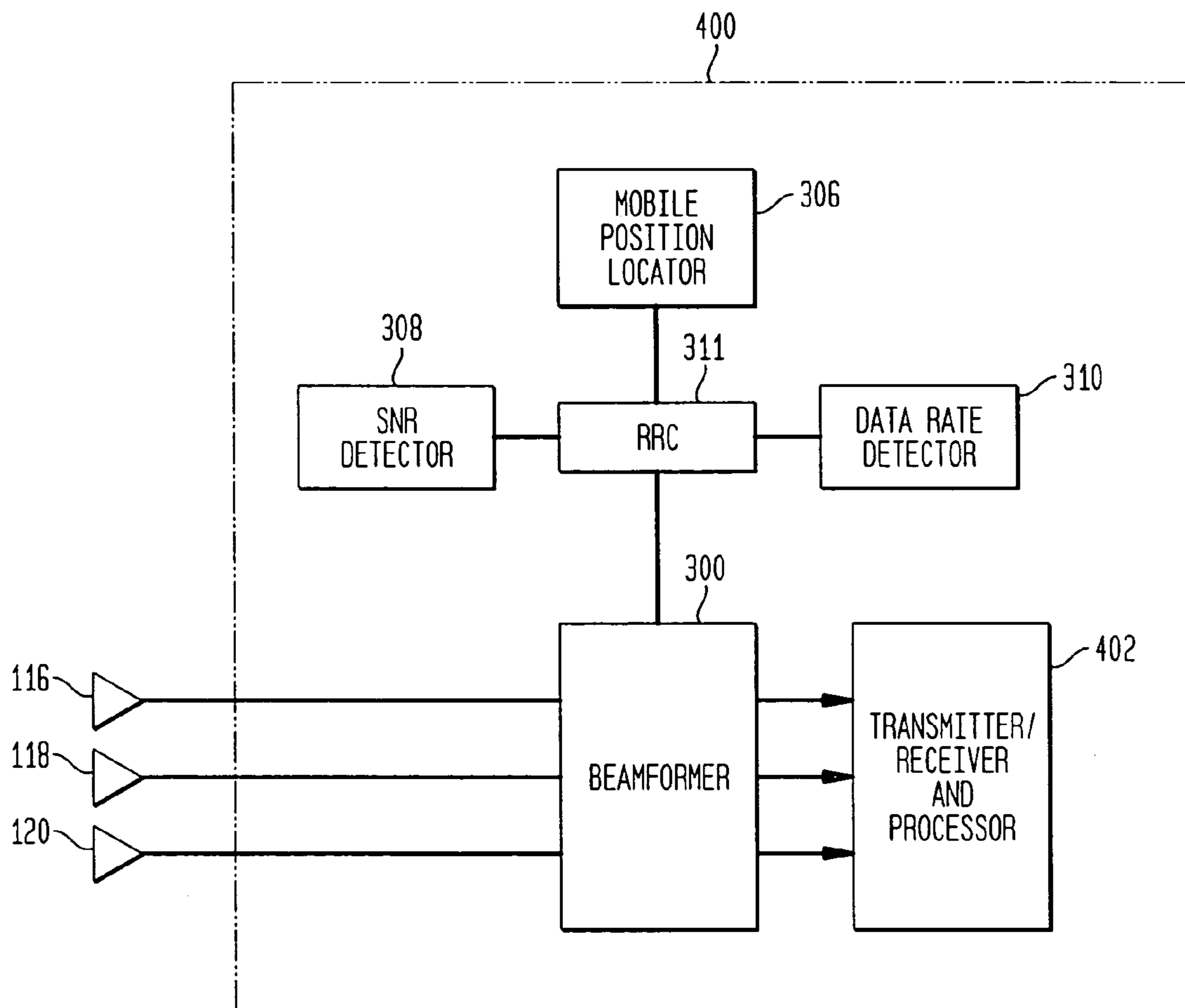
TRANSCEIVER SYSTEM AT A BASE STATION
