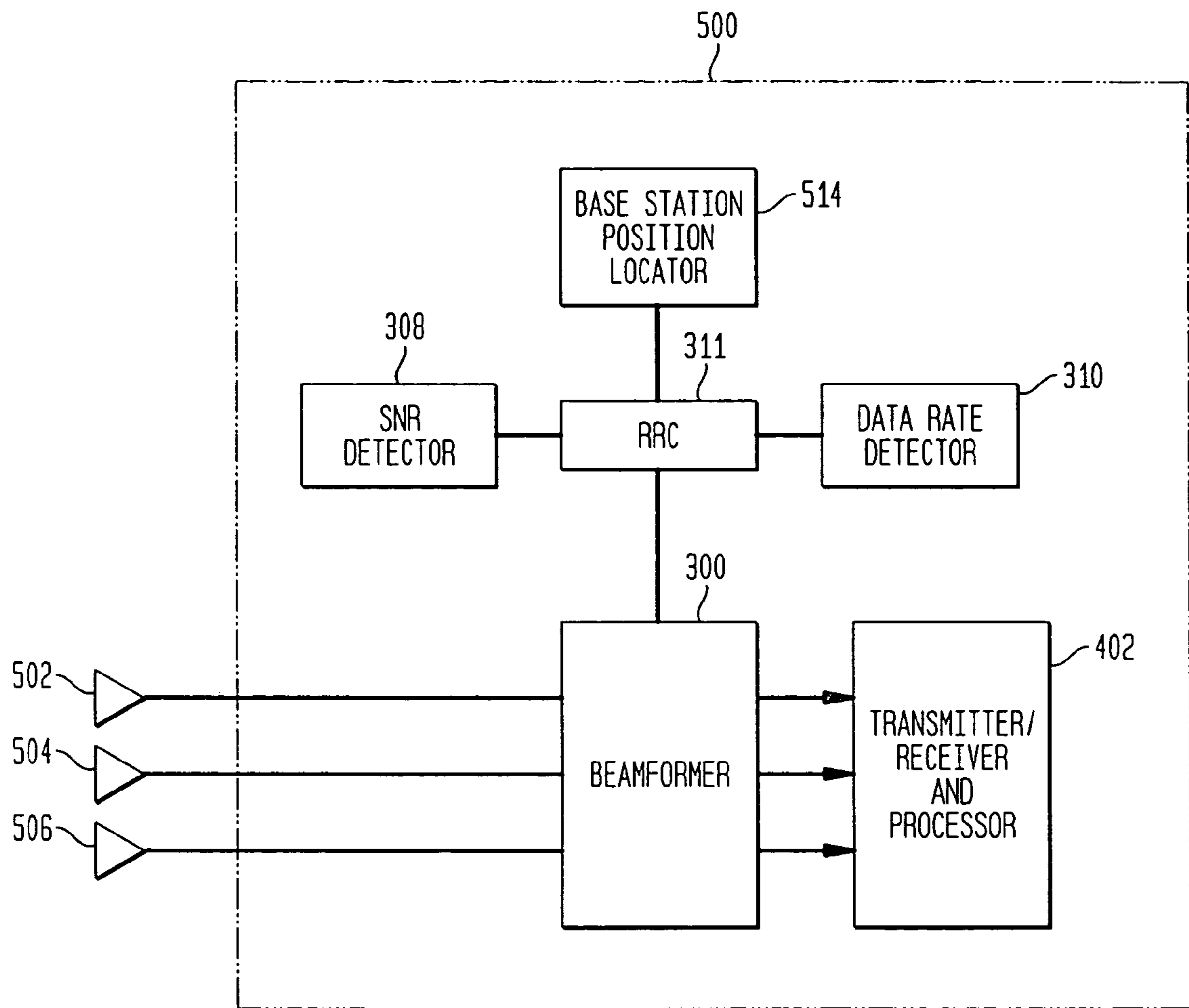
TRANSCIVER SYSTEM AT A MOBILE UNIT
