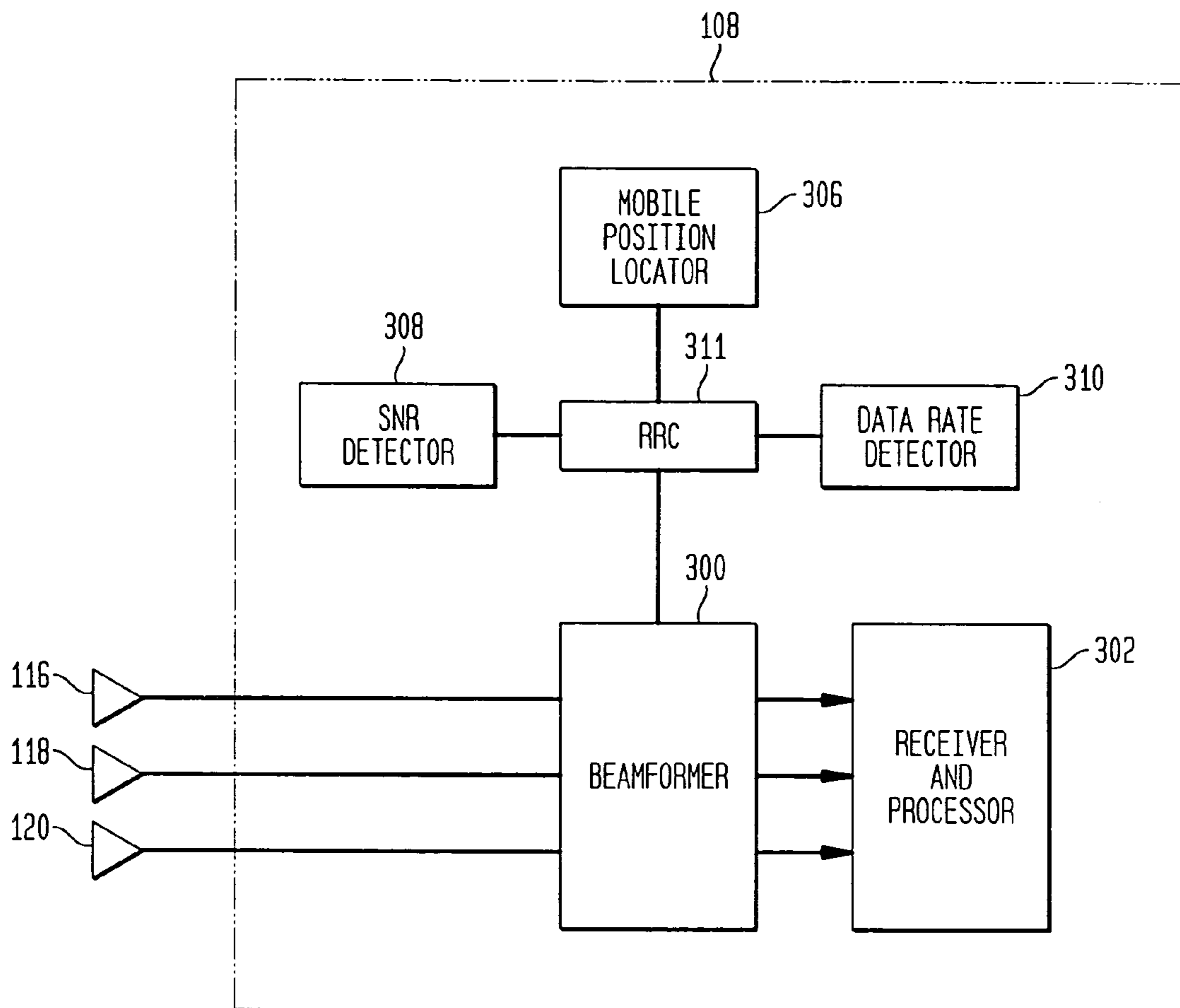
RECEIVE SYSTEM AT A BASE STATION
