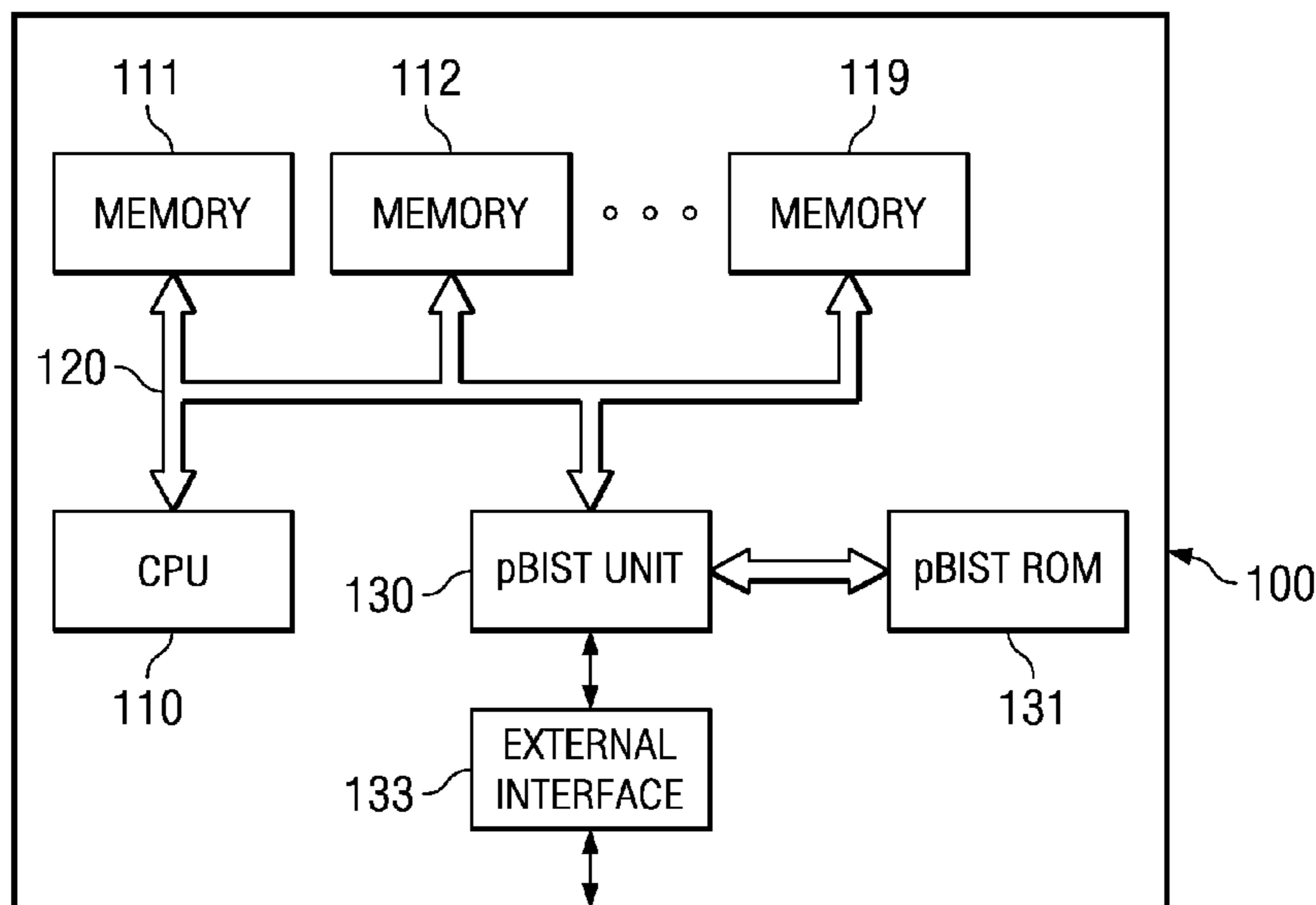
FIG. 1 (PRIOR ART)
