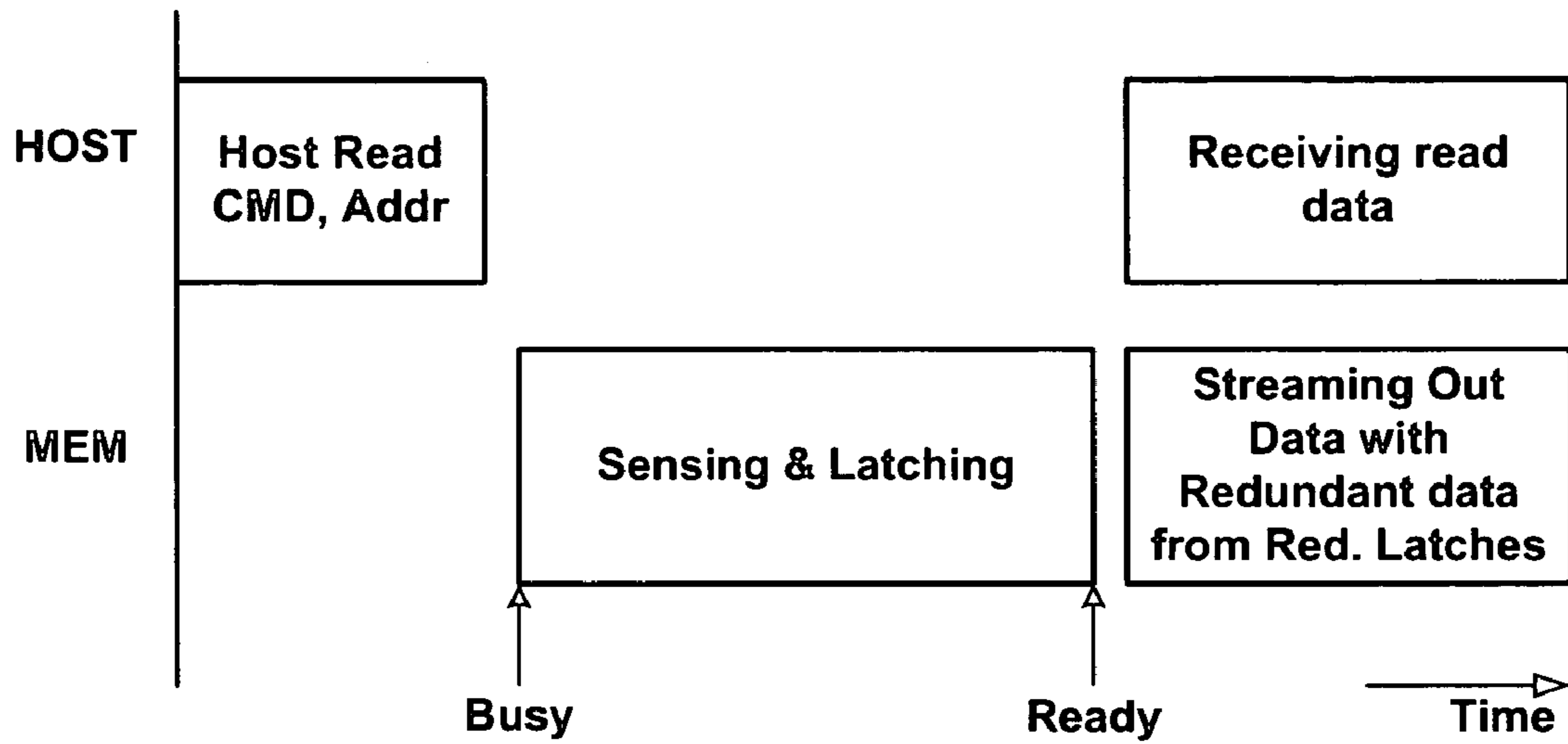
READ TIMING (Prior Art)
