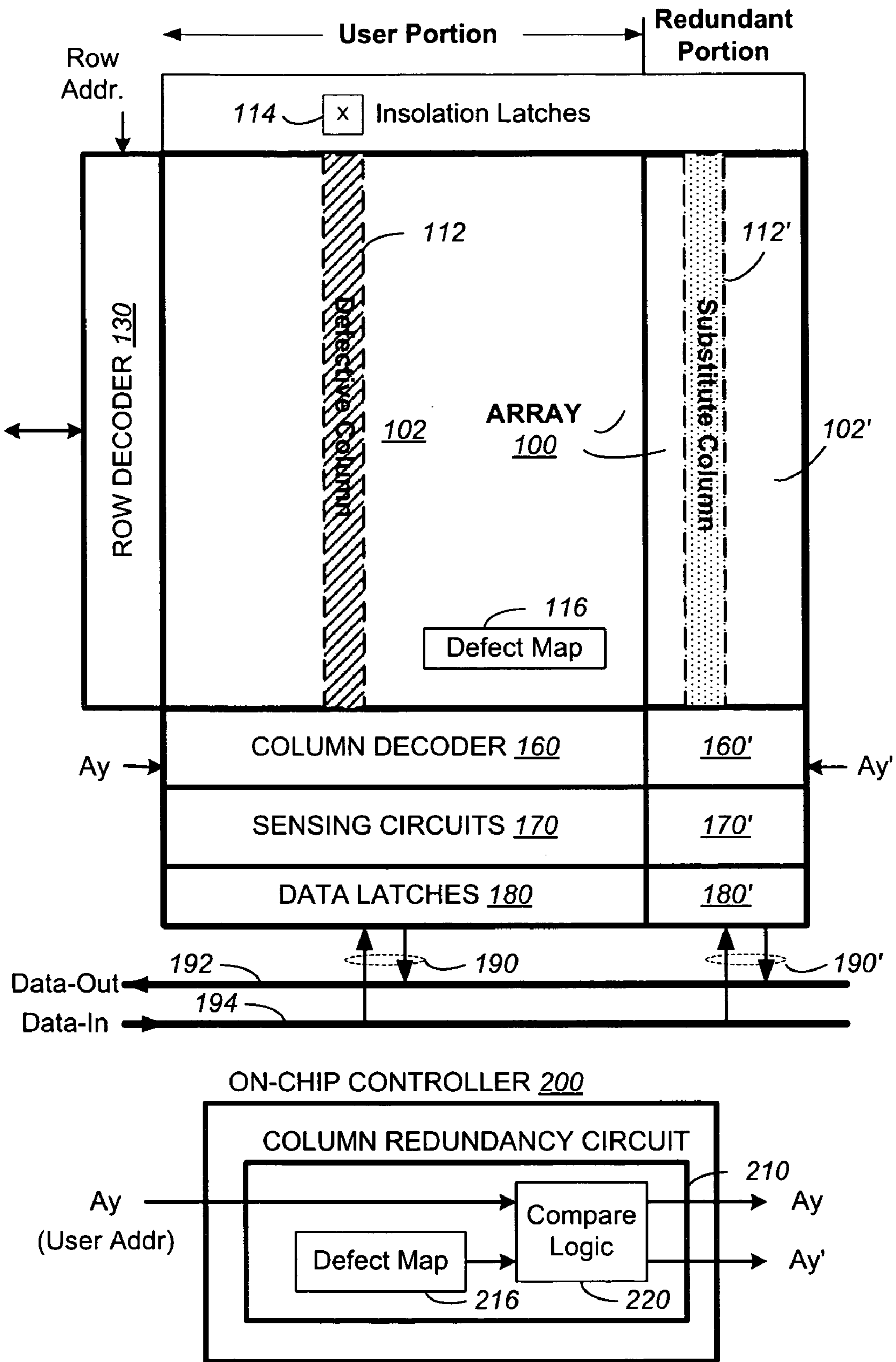
FIG. 1 (Prior Art)
