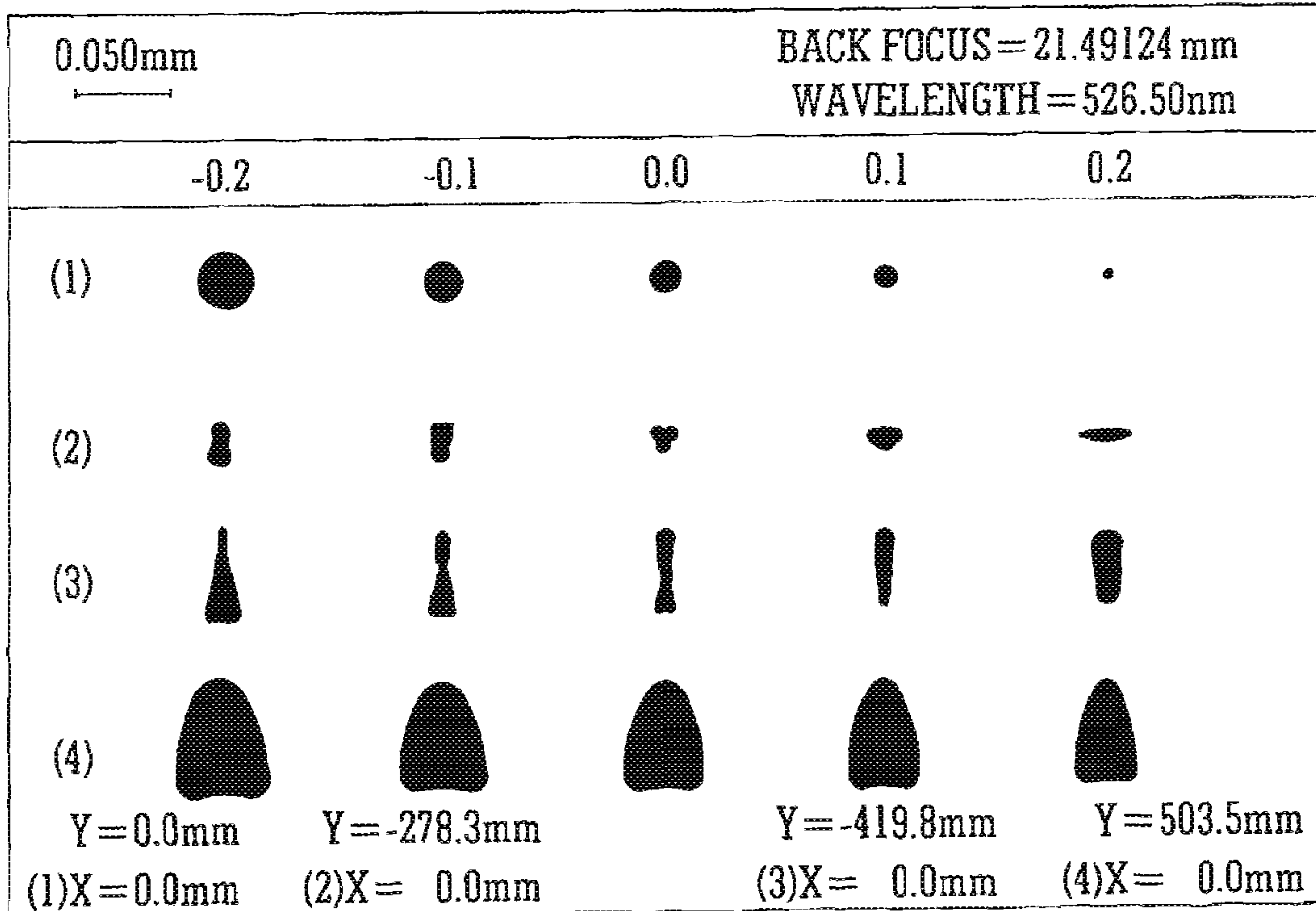
ZOOM CONFIGURATION 4
