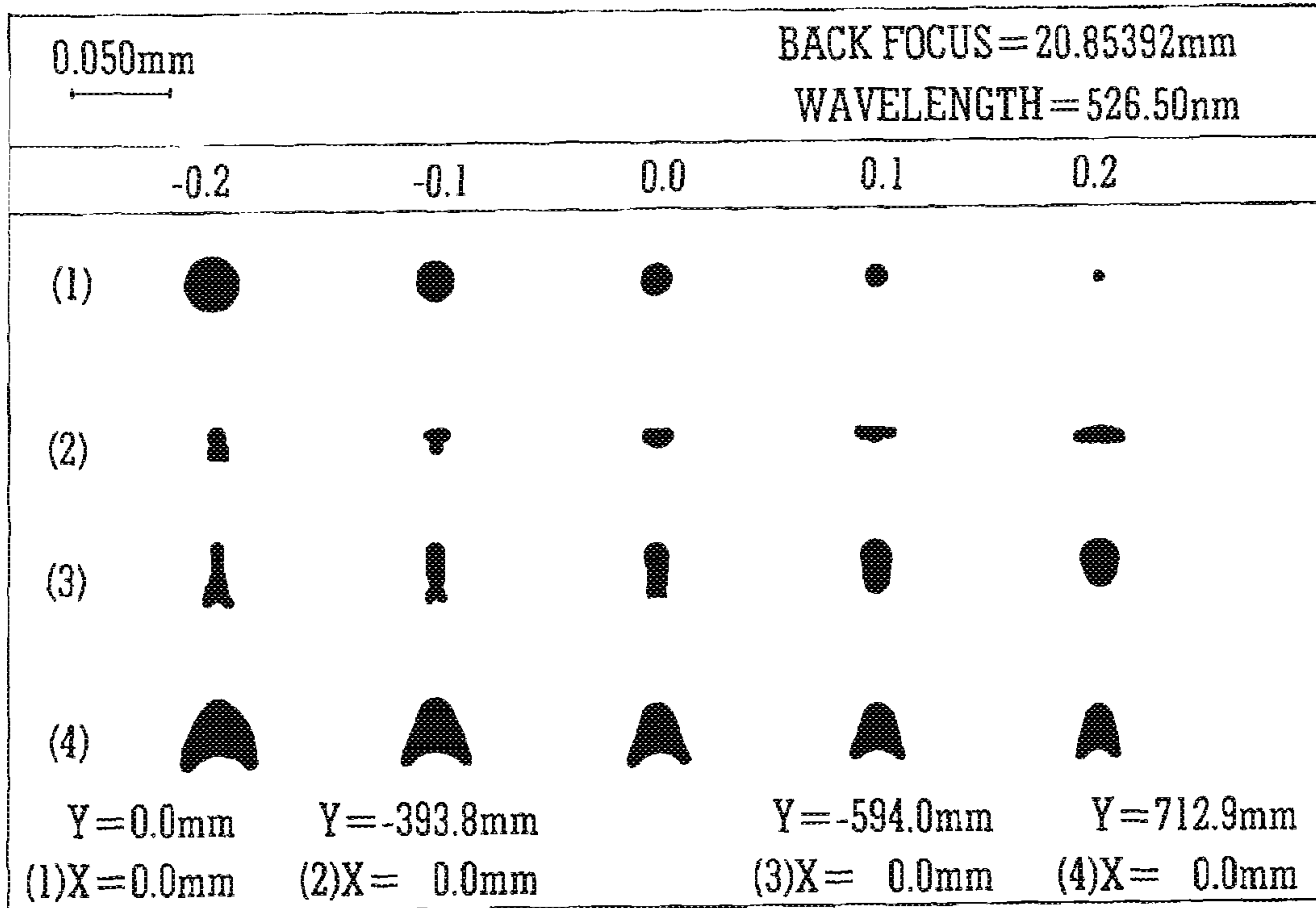
ZOOM CONFIGURATION 3
