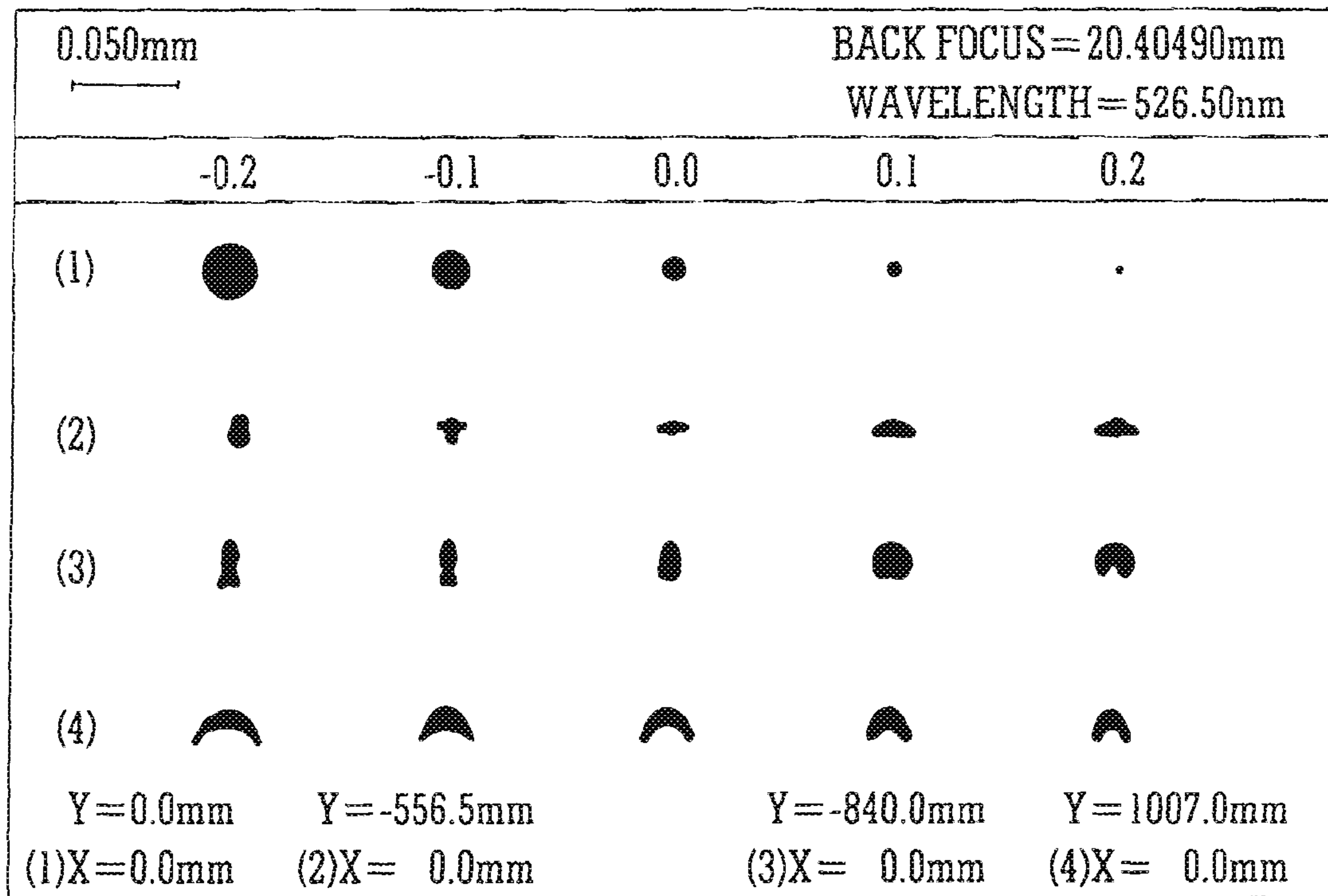
ZOOM CONFIGURATION 2
