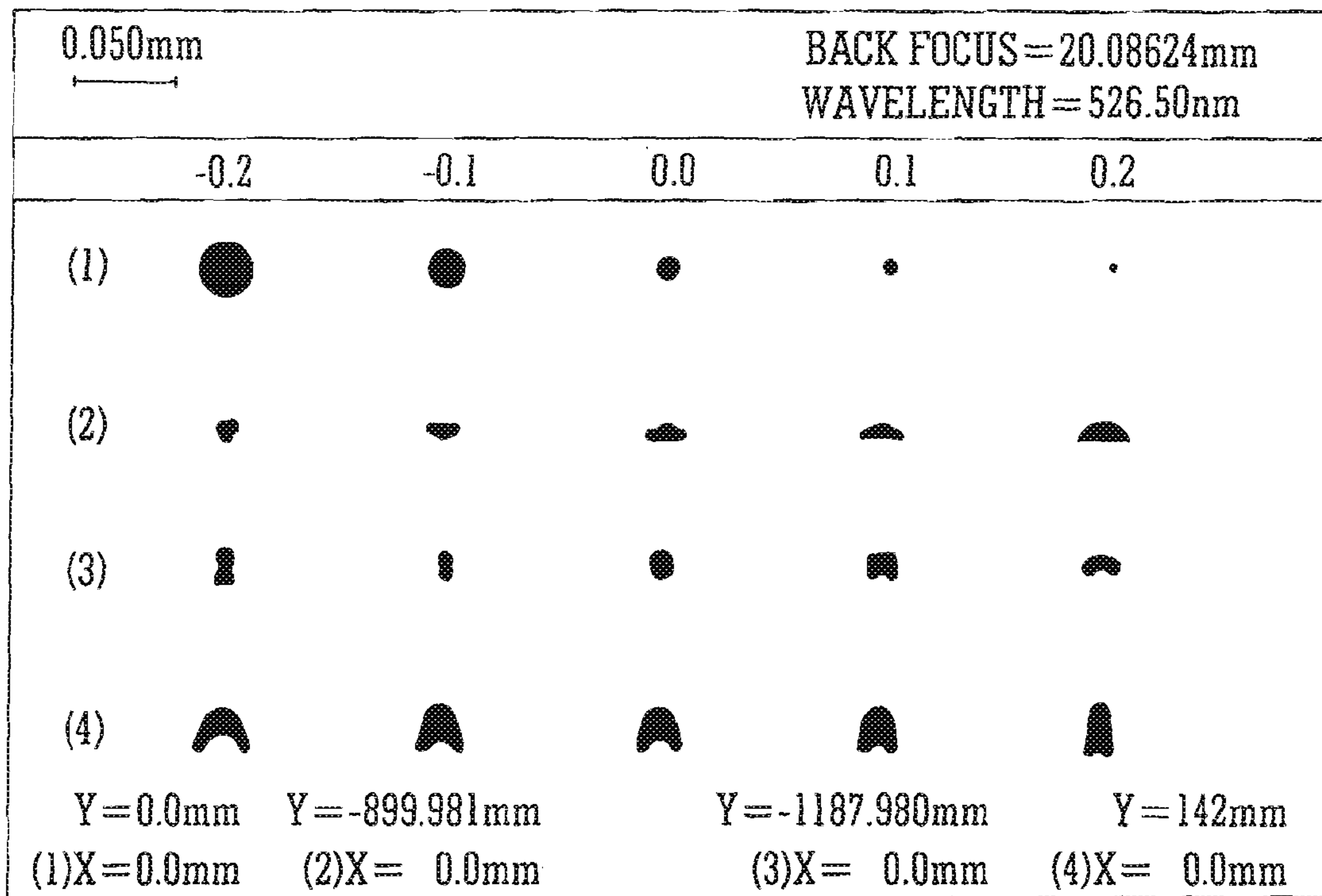
ZOOM CONFIGURATION 1
