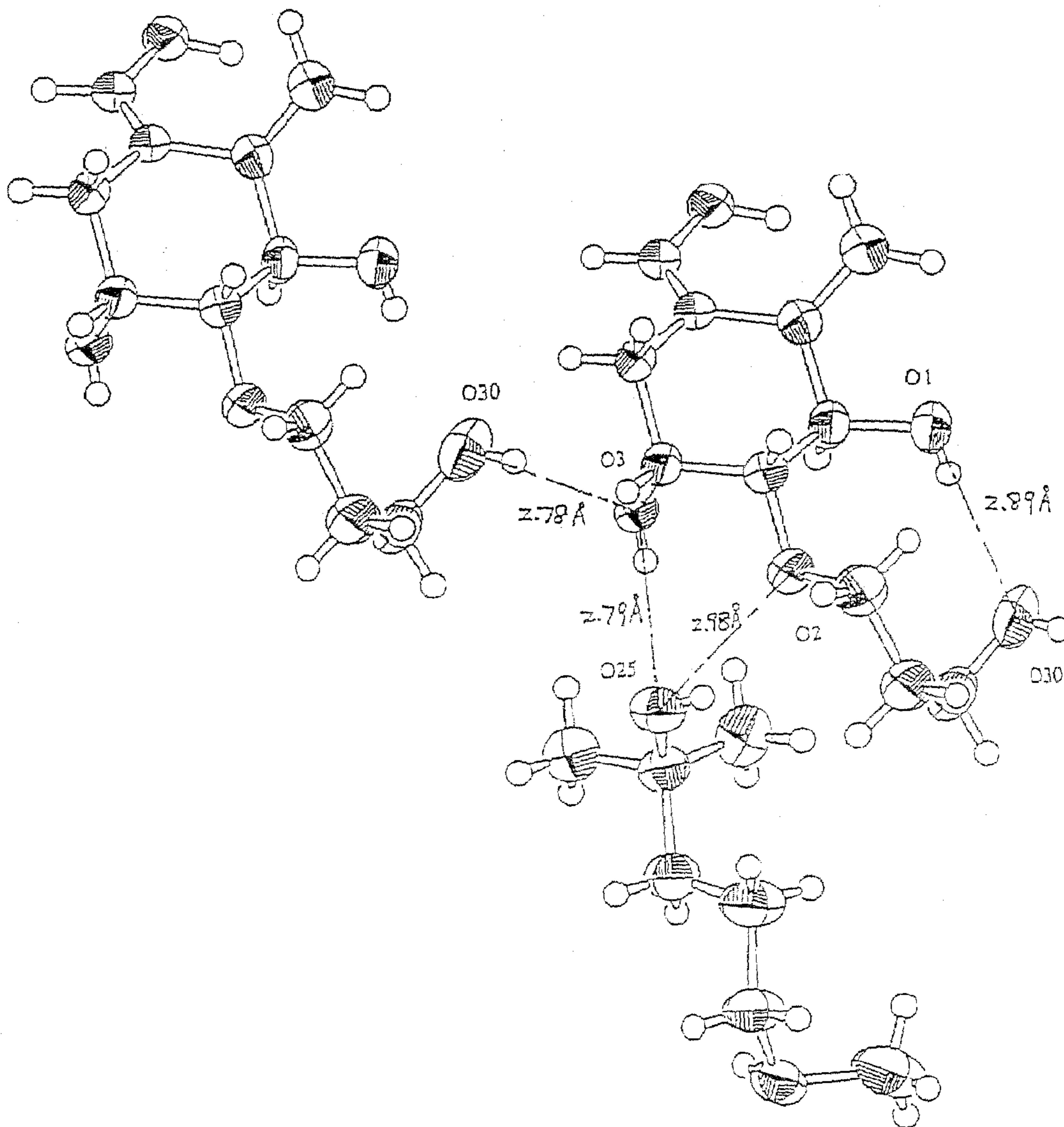
Structure of ED-71 where hydrogen bonds are focused (1)
