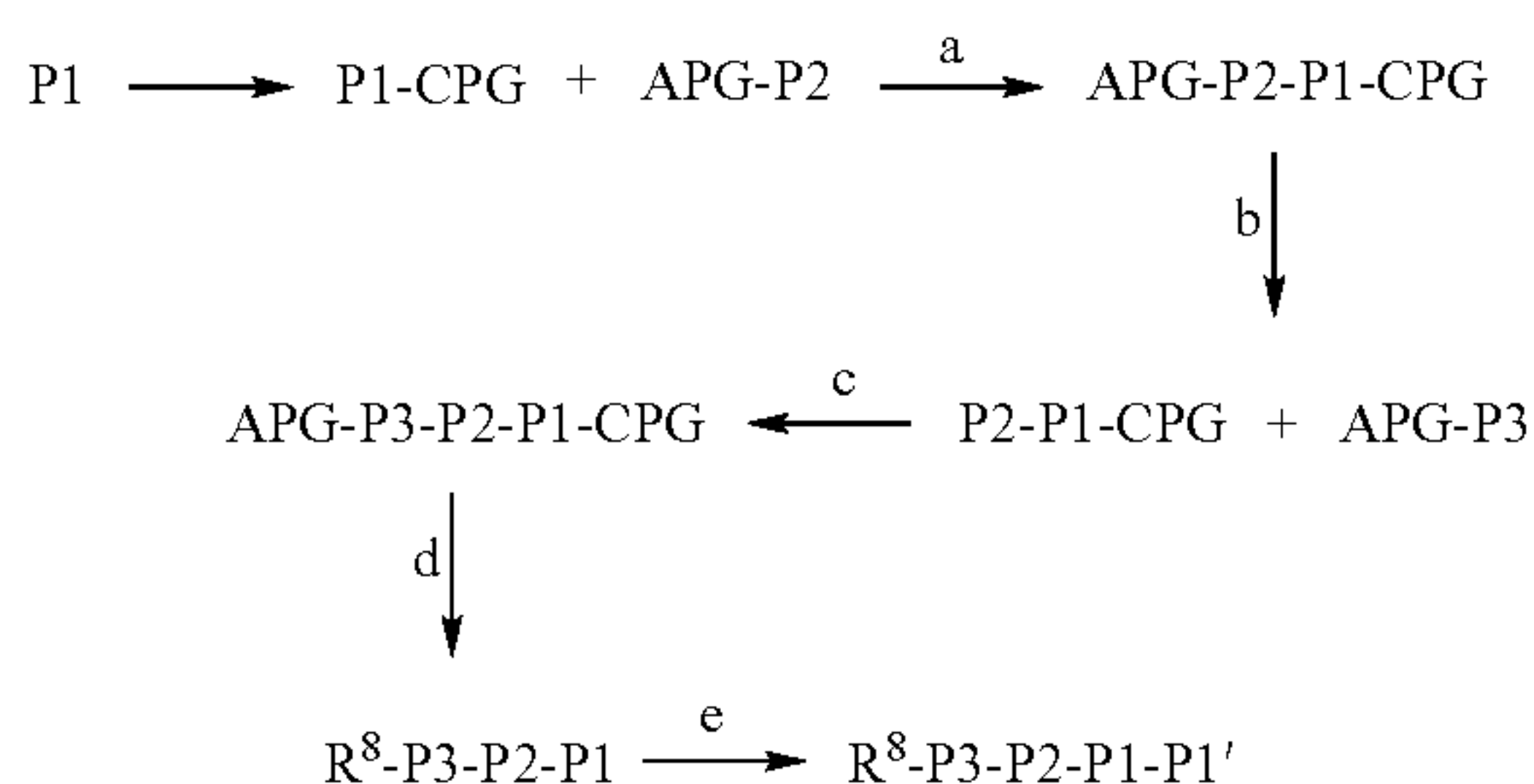
Scheme I
