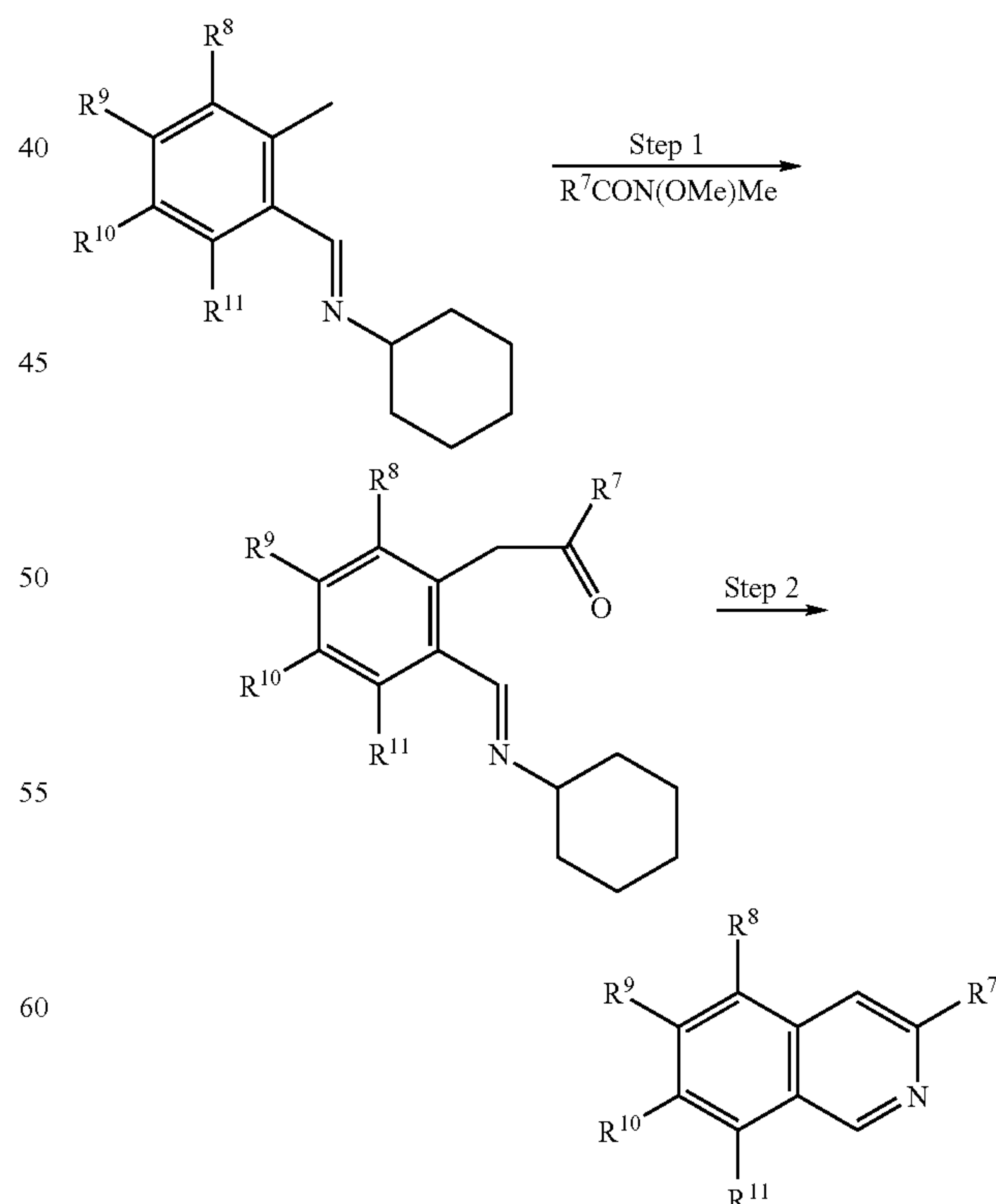
Scheme XV
