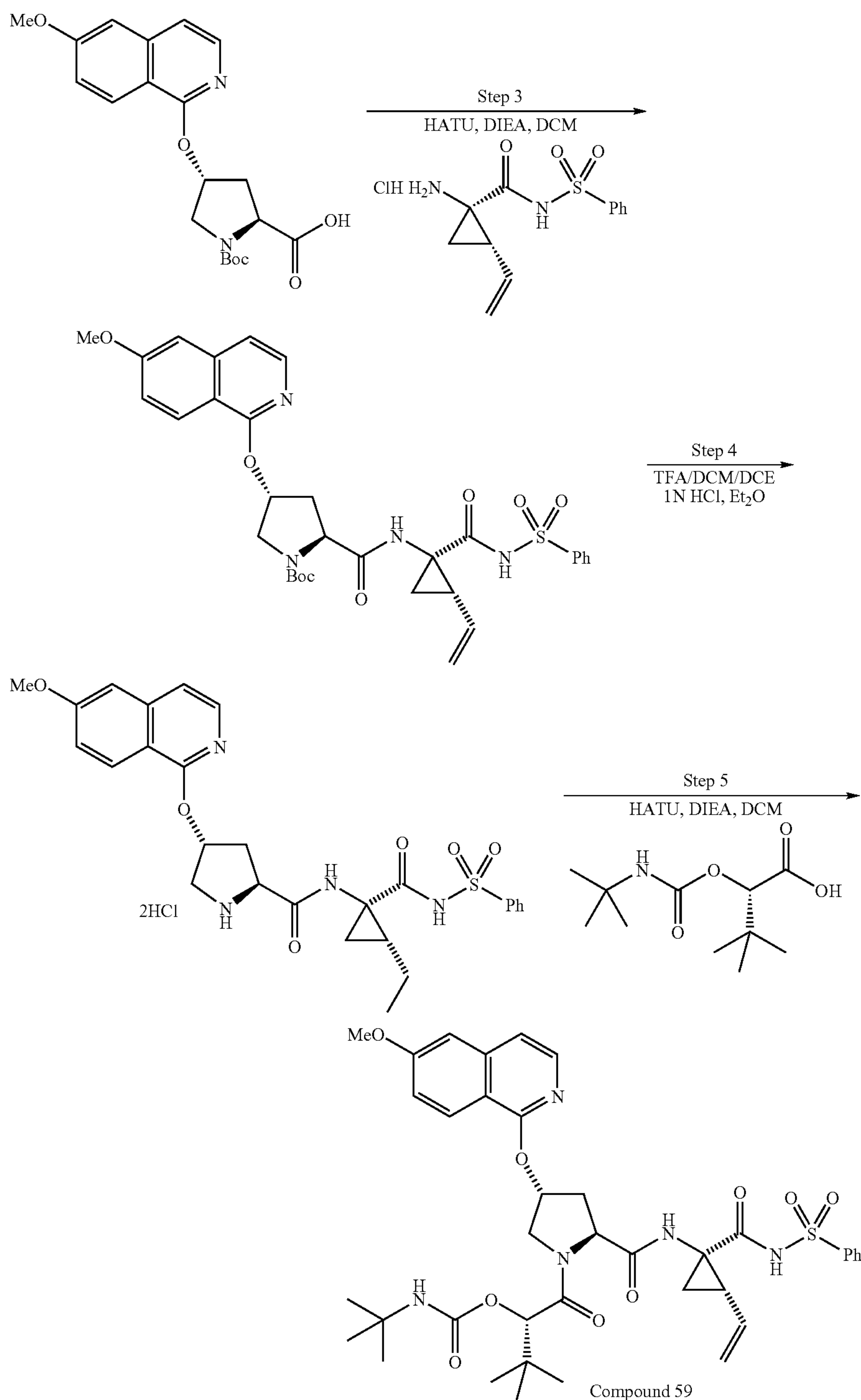
Scheme 2.
