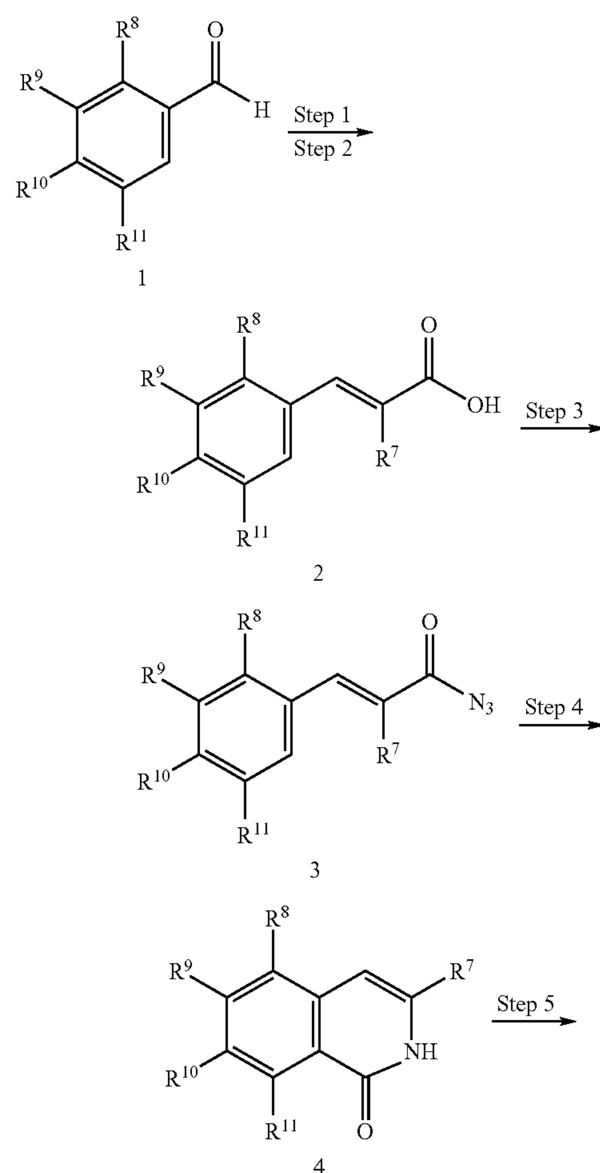
Scheme XI
