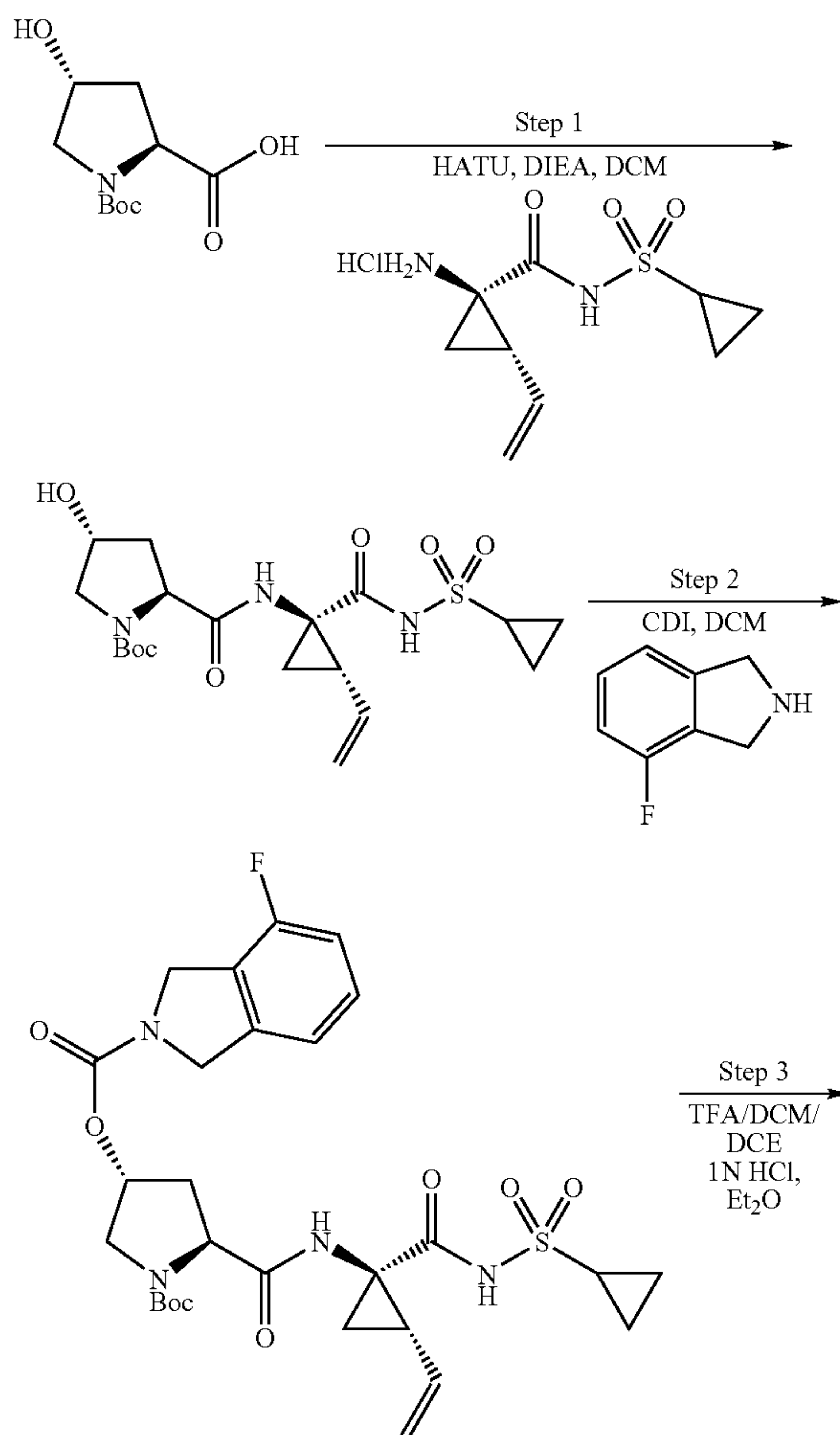
Scheme 2
