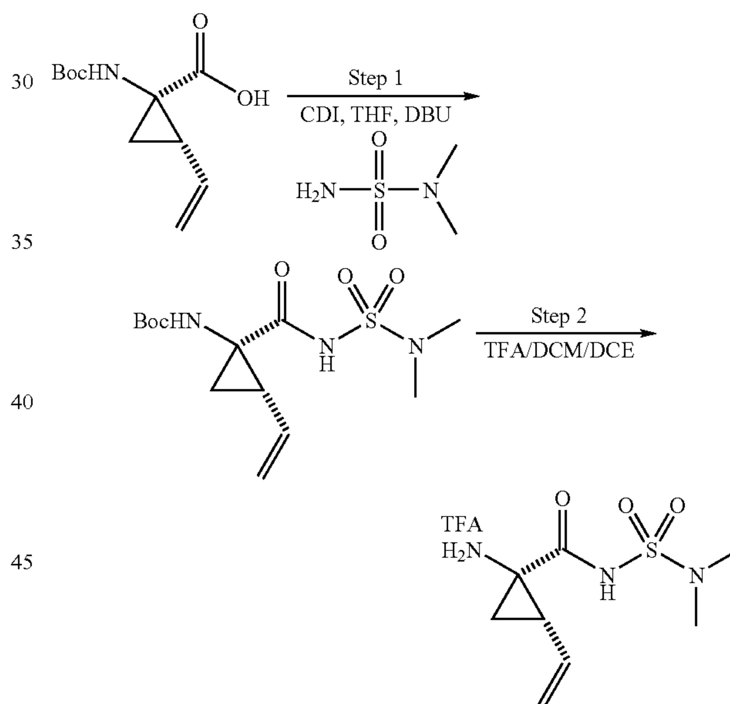
Scheme 1.
