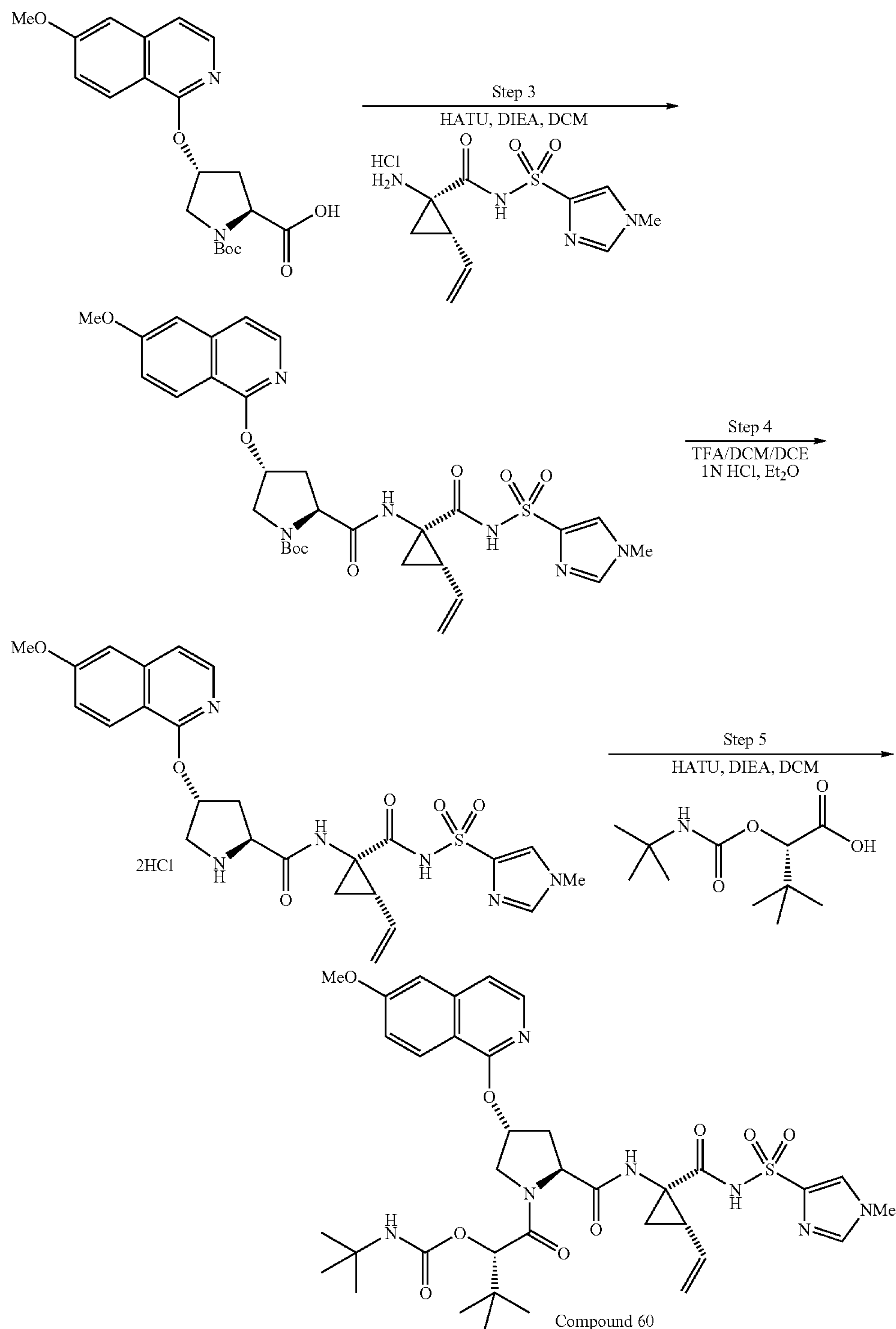
Scheme 2.
