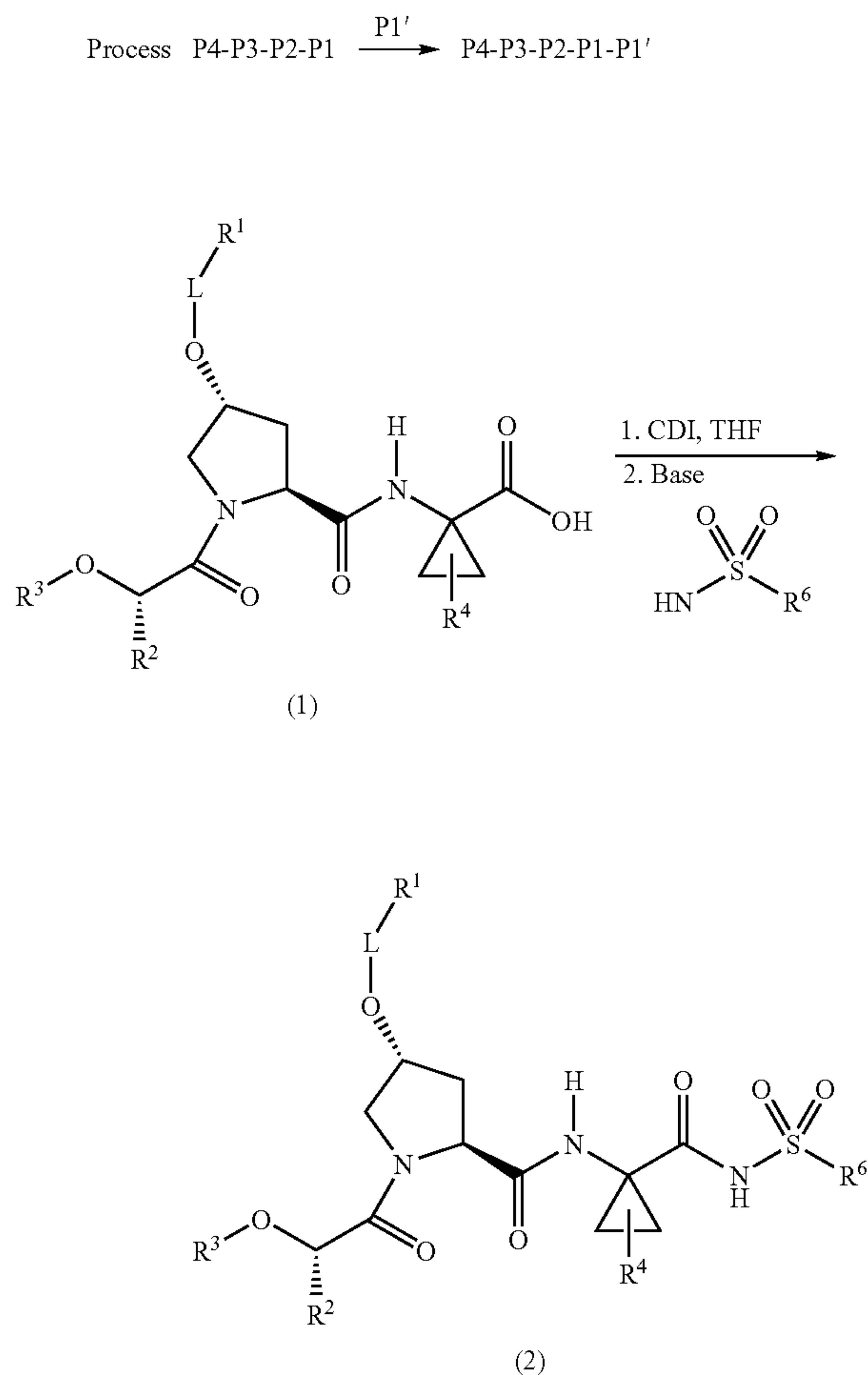
Scheme II
