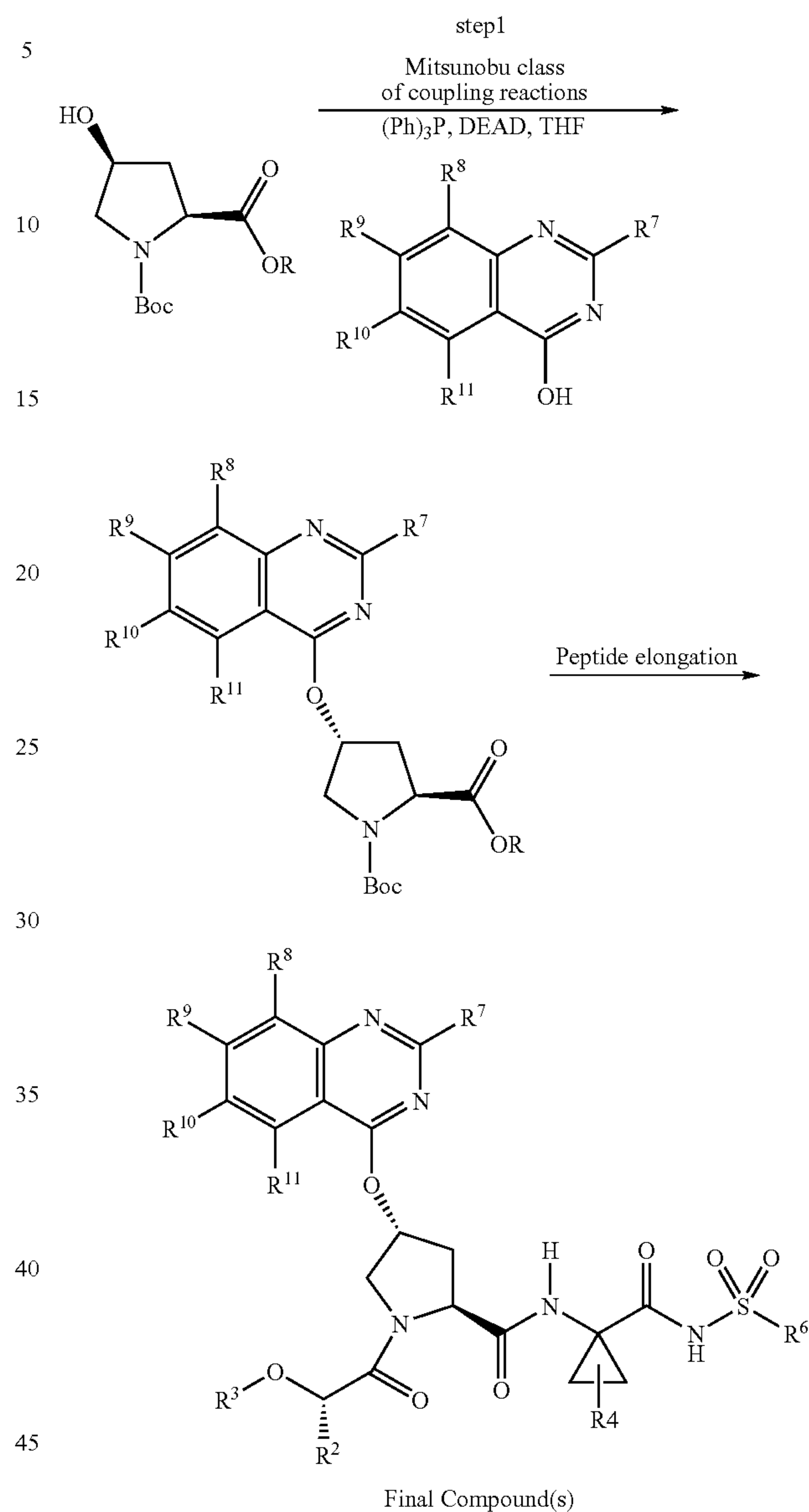
Scheme X
