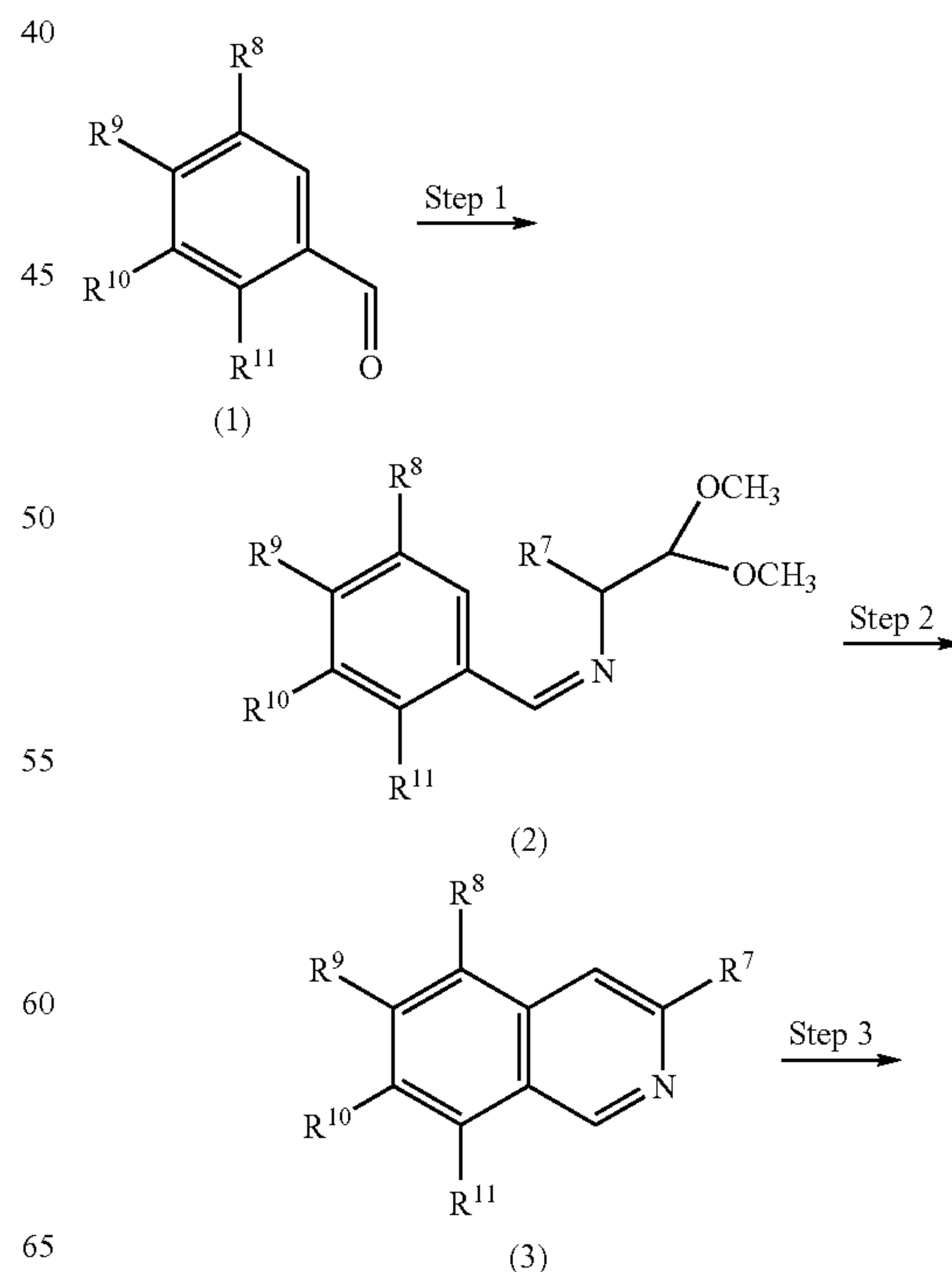
Scheme XII
