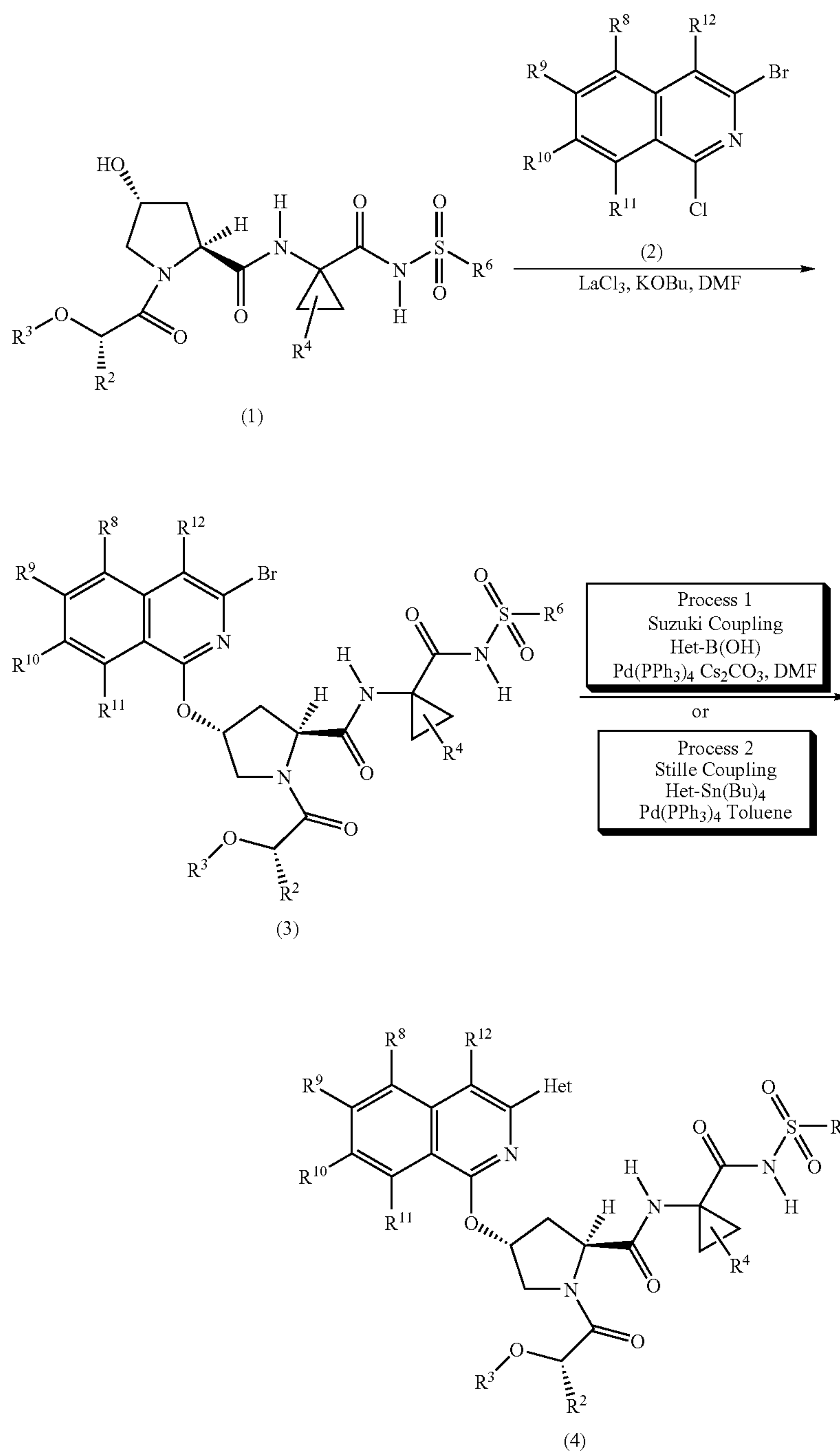
Scheme XVIII
