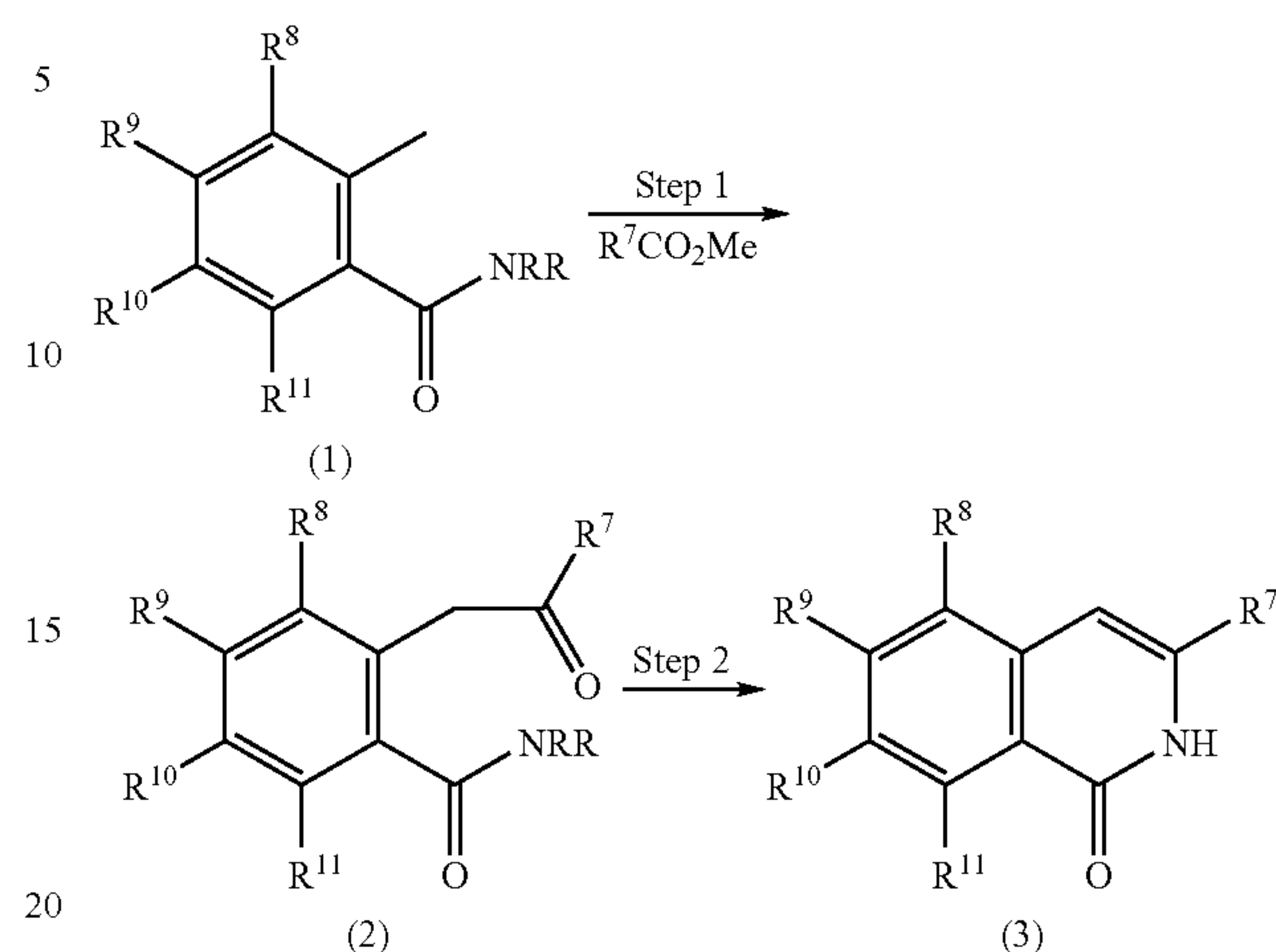
Scheme XIV
