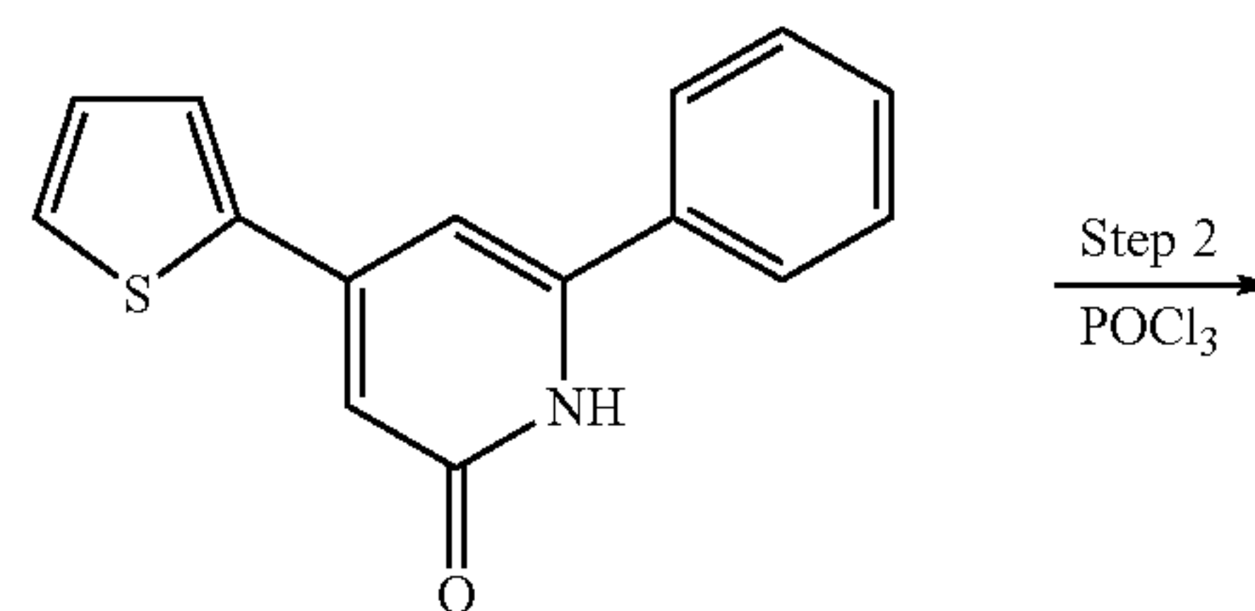
Scheme 2
