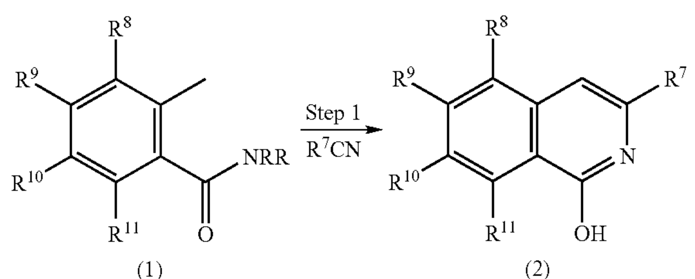
Scheme XIII
