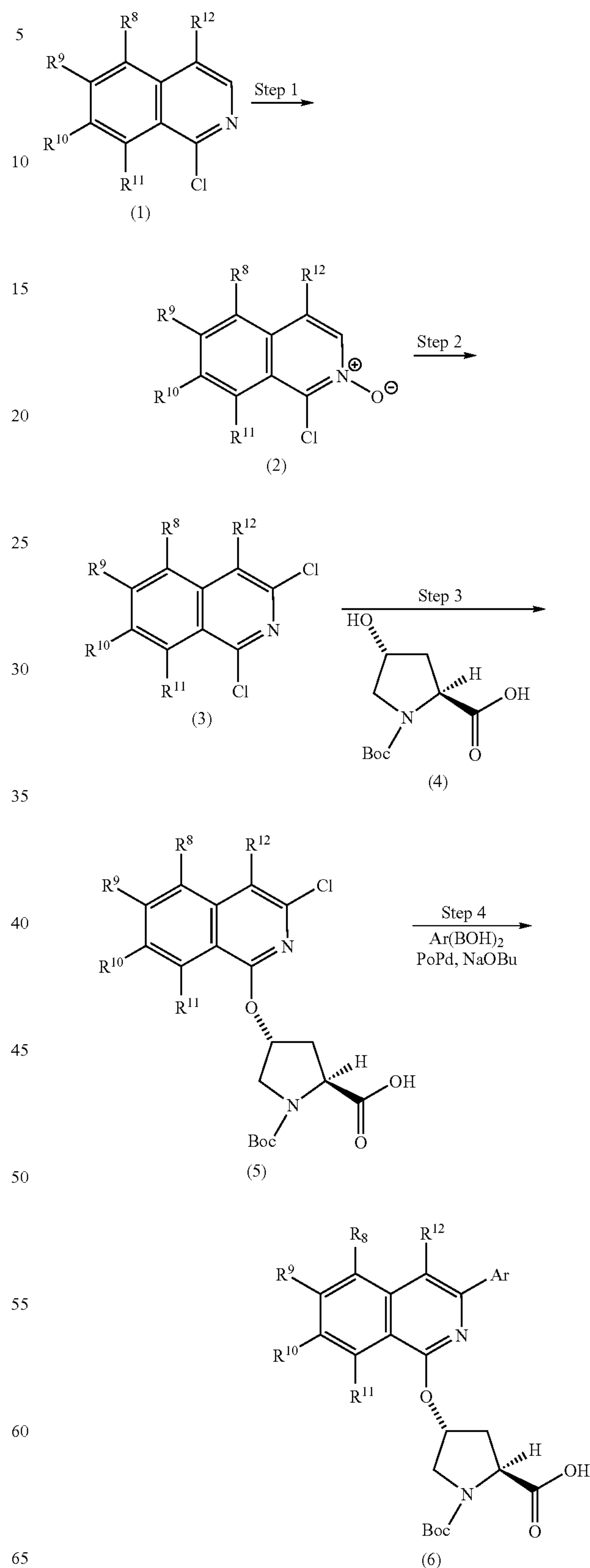
Scheme XVII
