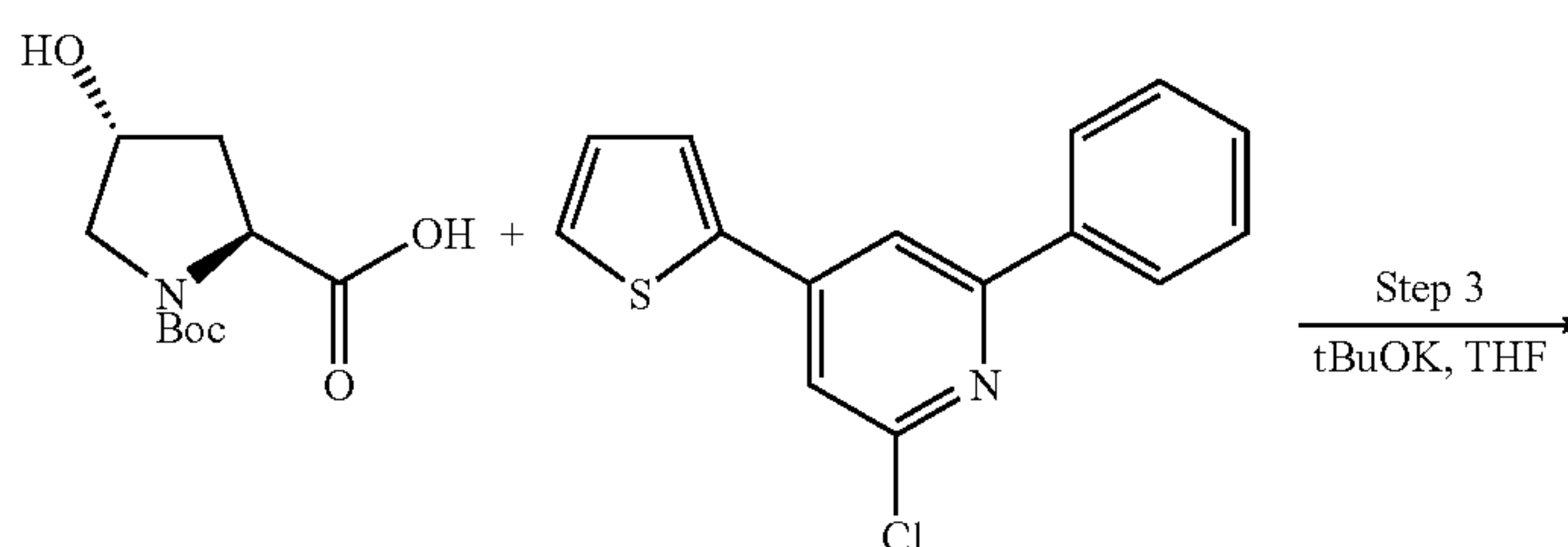
Scheme 3
