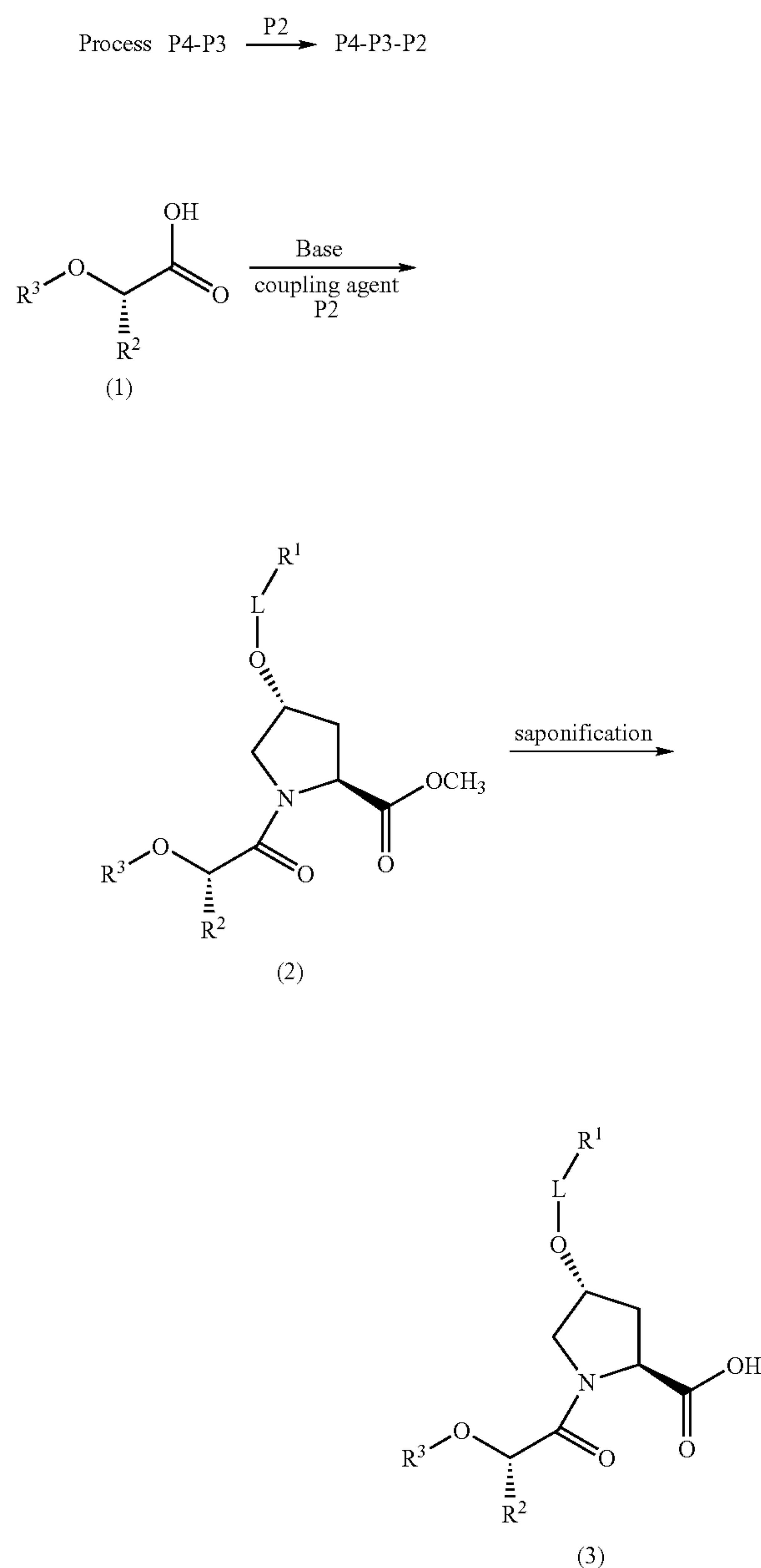
Scheme V
