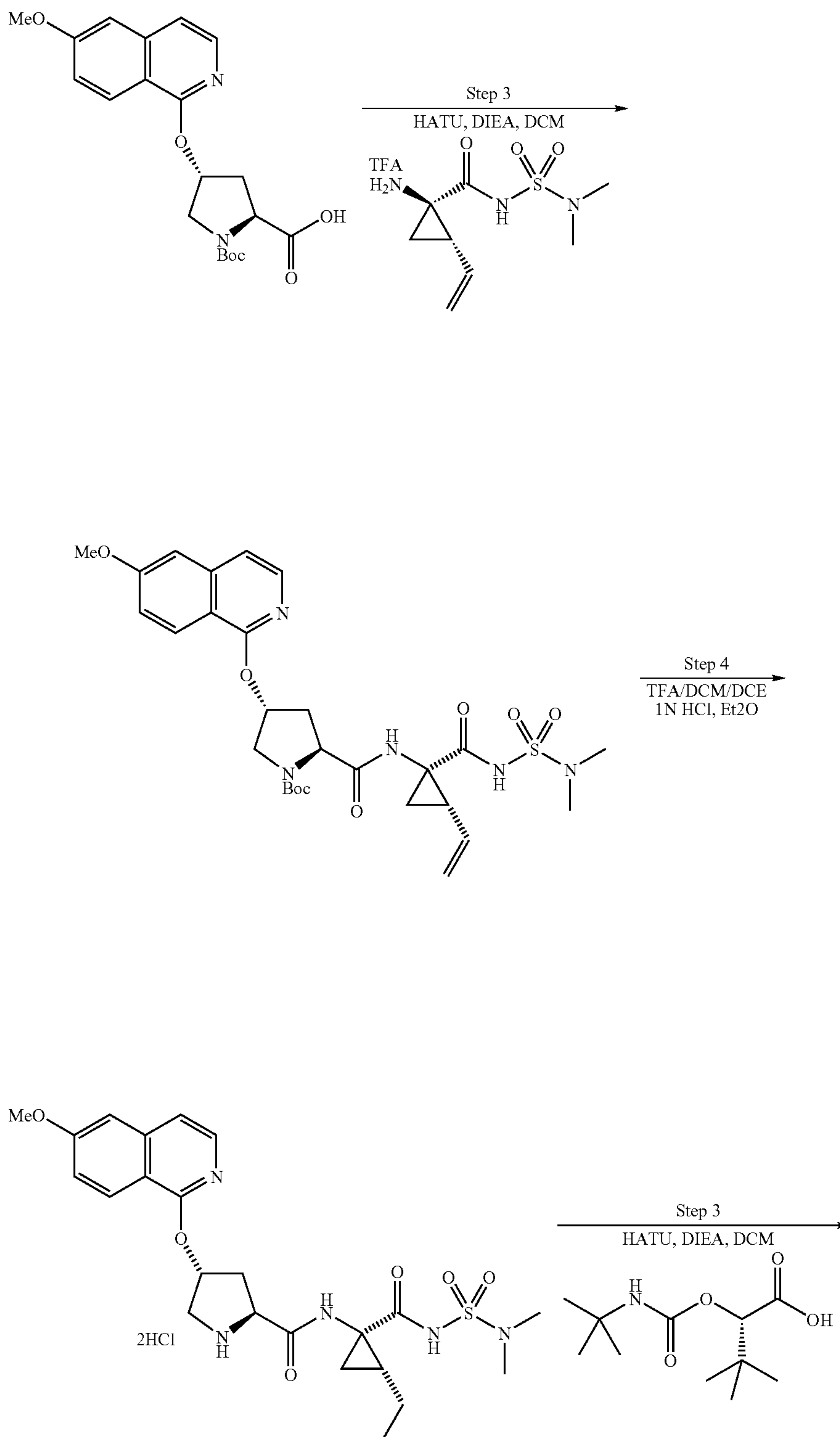
Scheme 2
