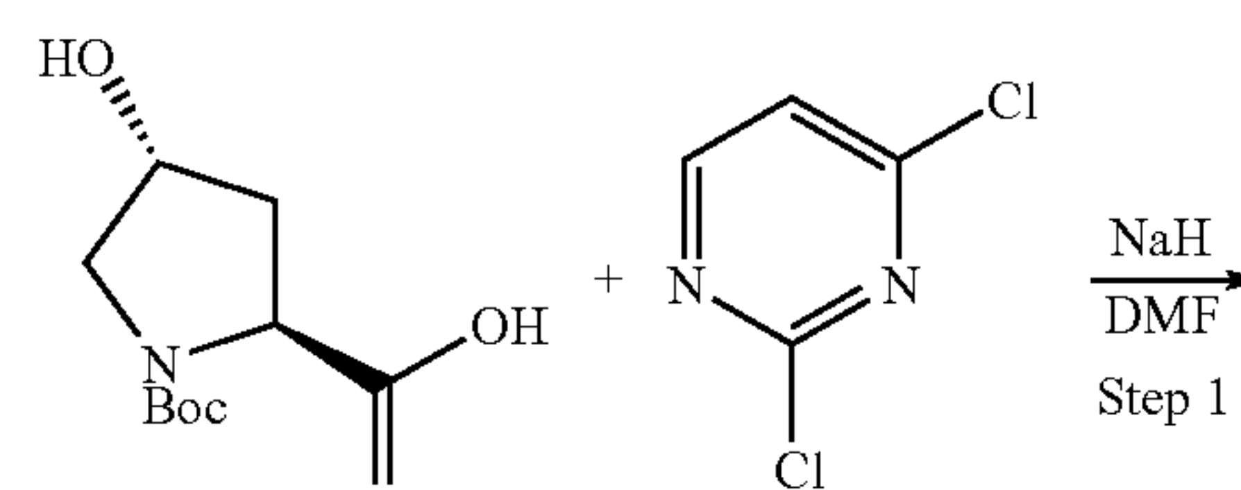
Scheme 1
