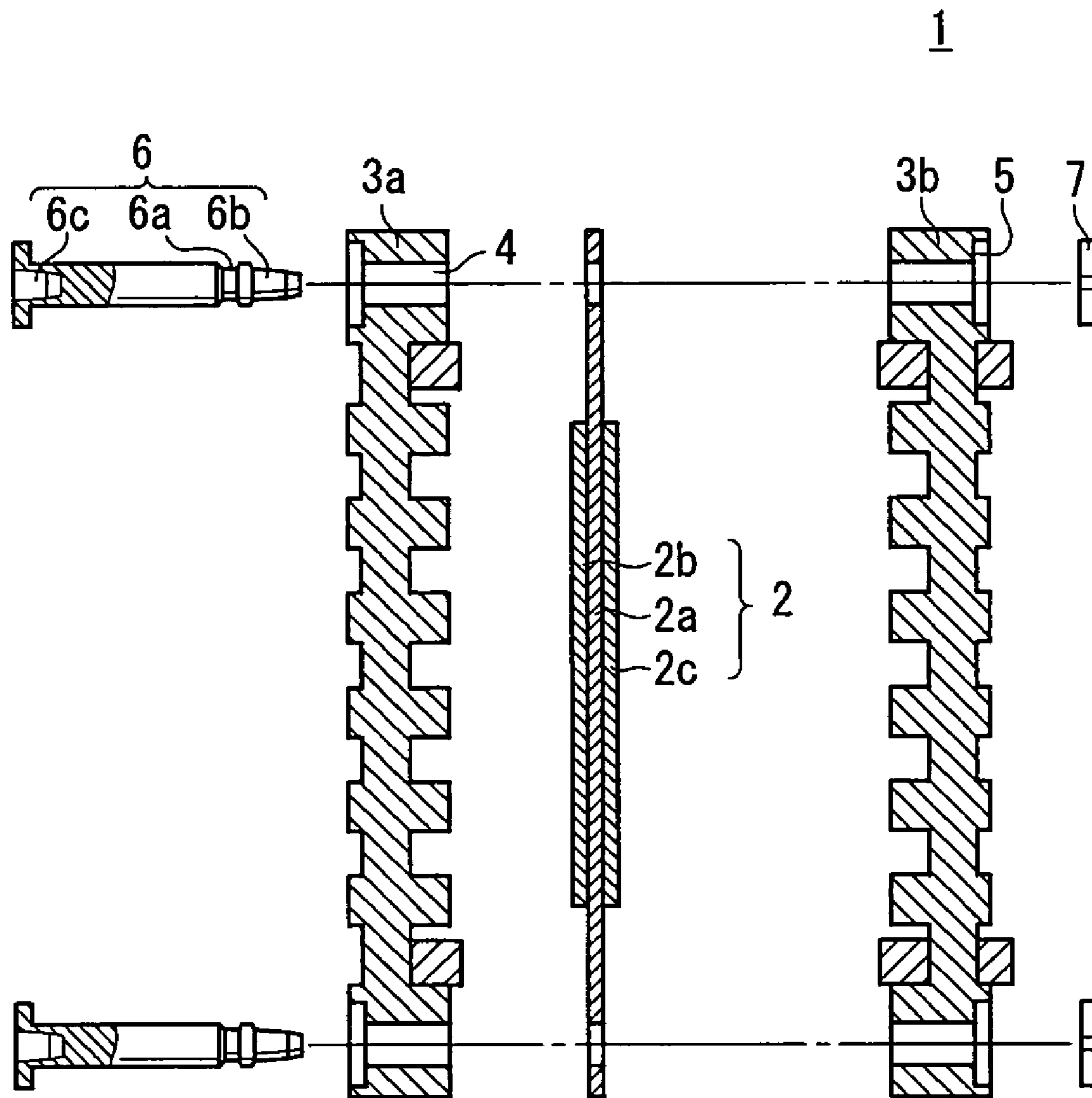
FIG. 9 PRIOR ART
