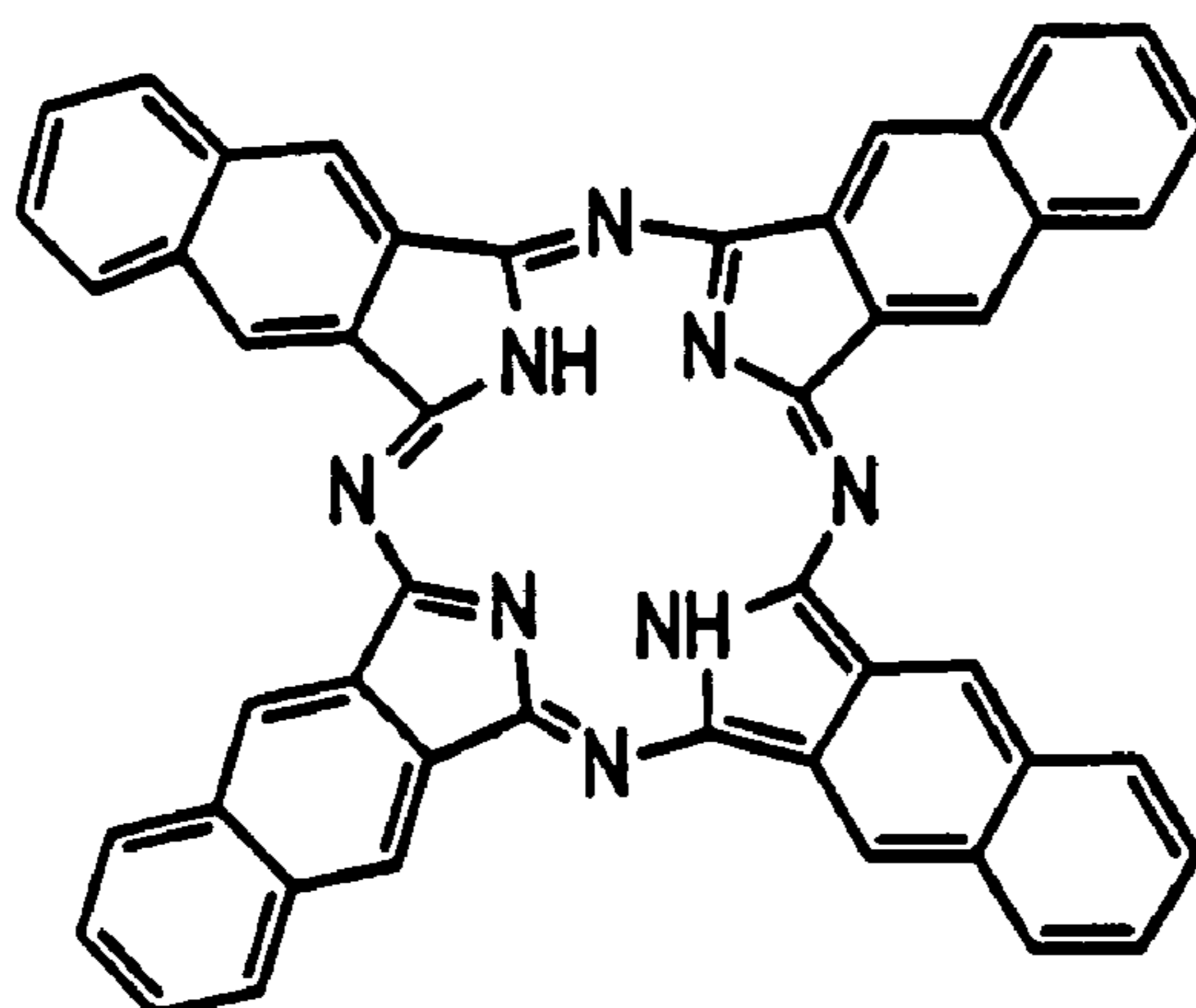
NAPHTHALOCYANINE
