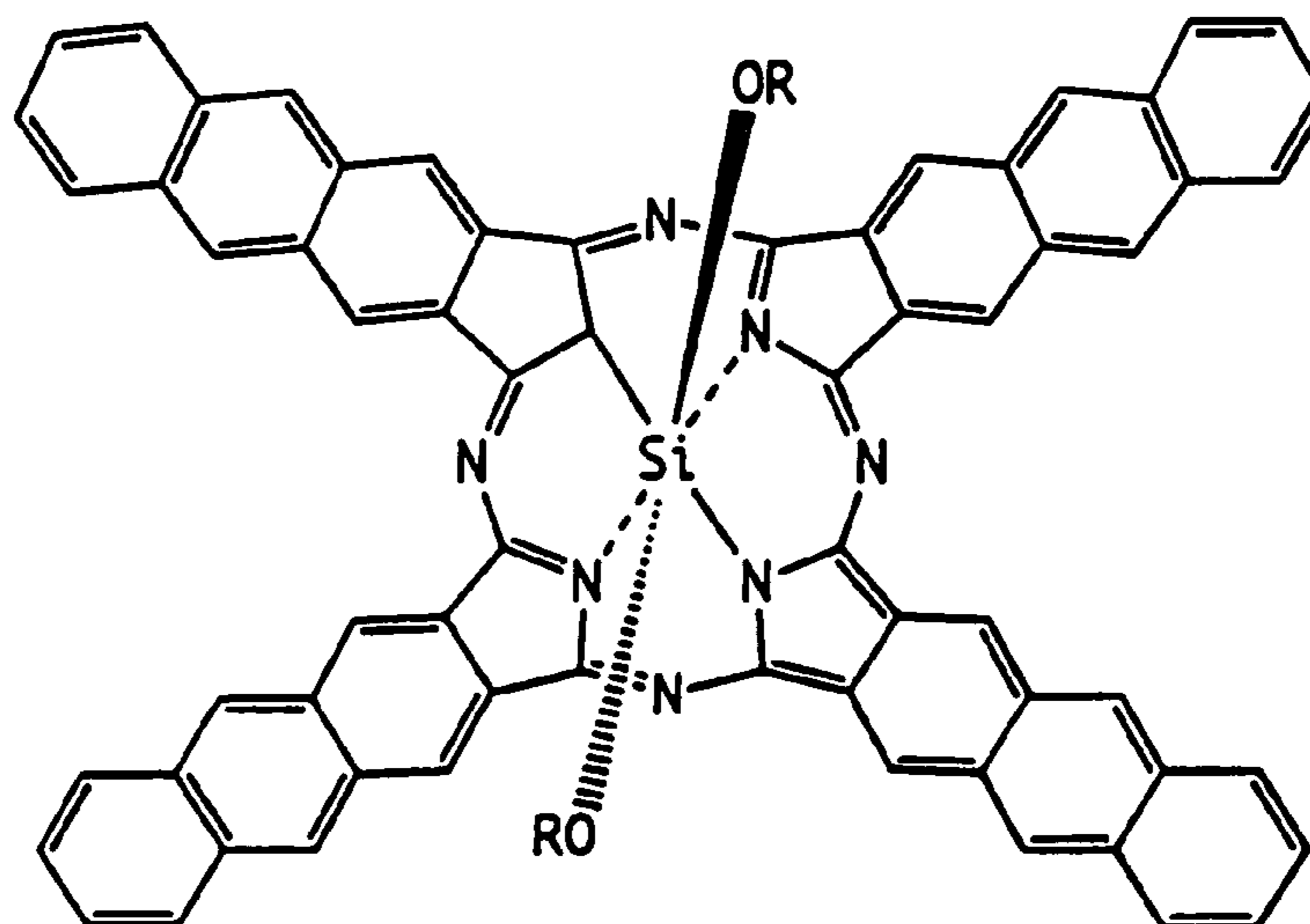
SILICON ANTHRACYANINE
