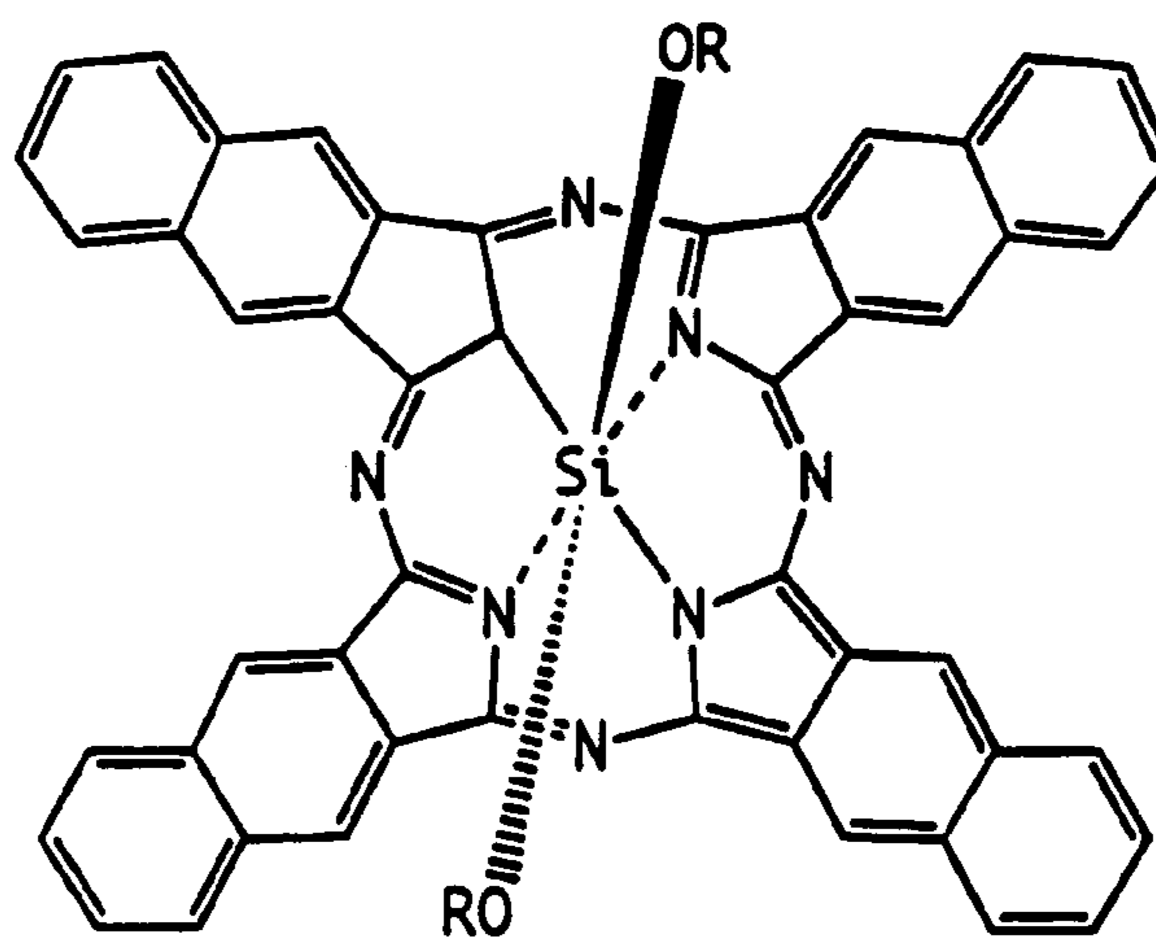
SILICON NAPHTHALOCYANINE
