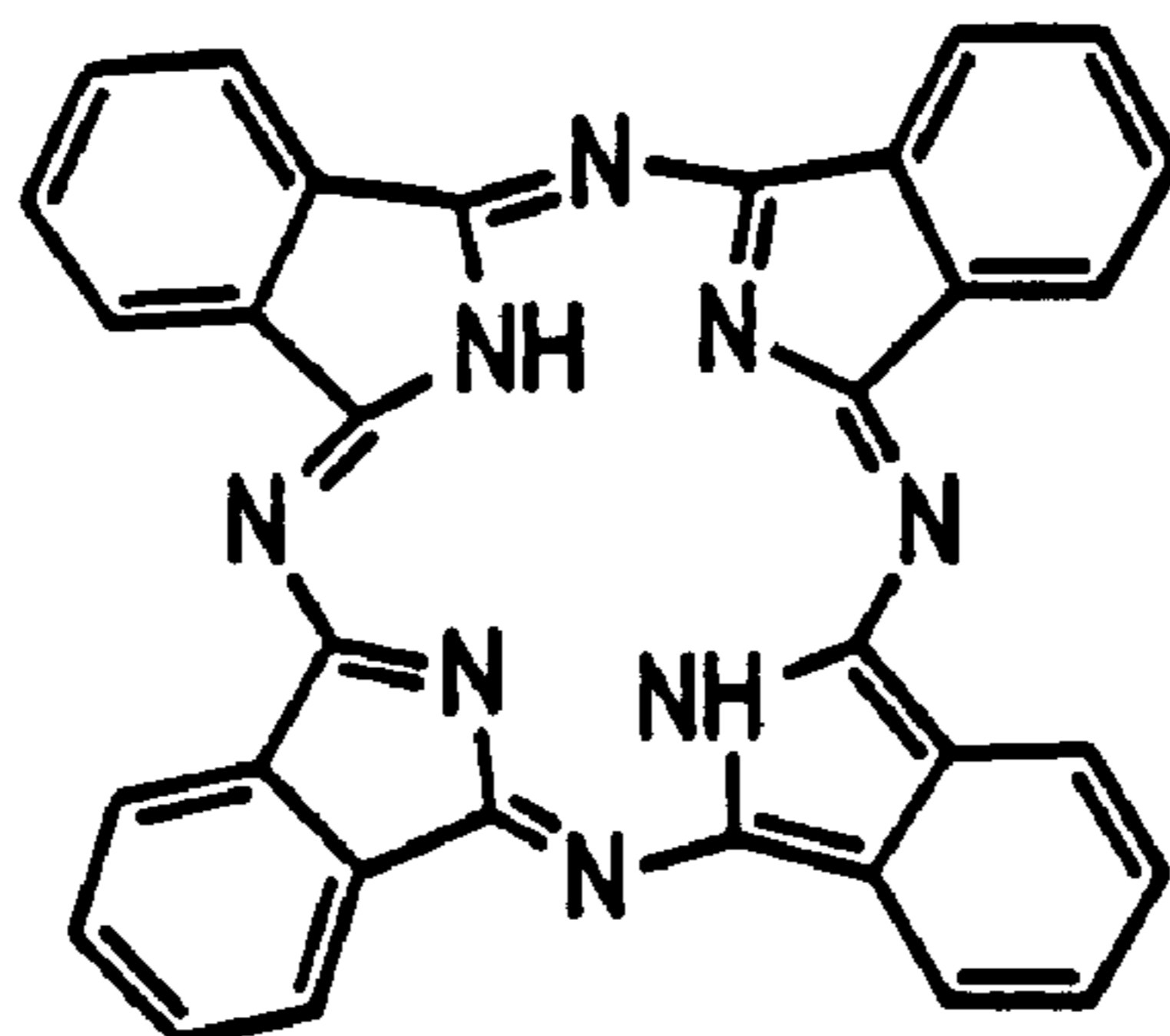
PHTHALOCYANINE
