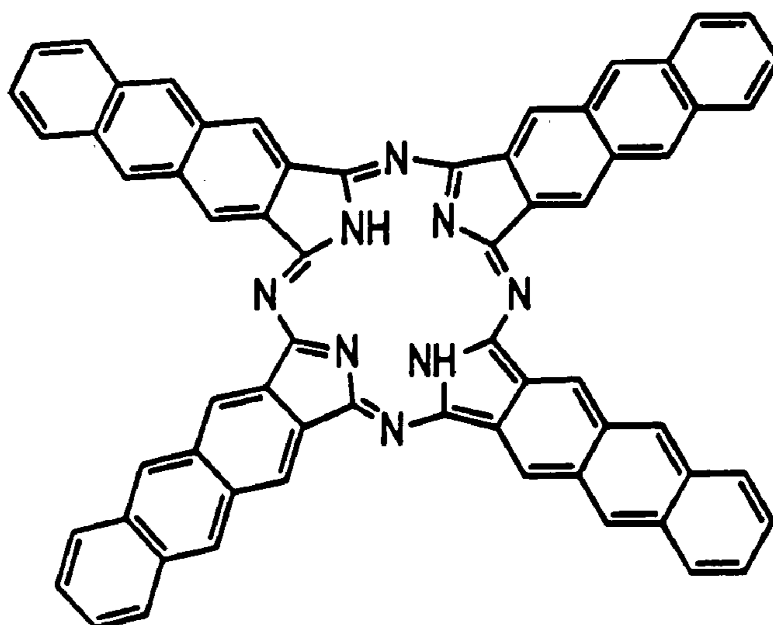
ANTHRANYLOCYANINE
