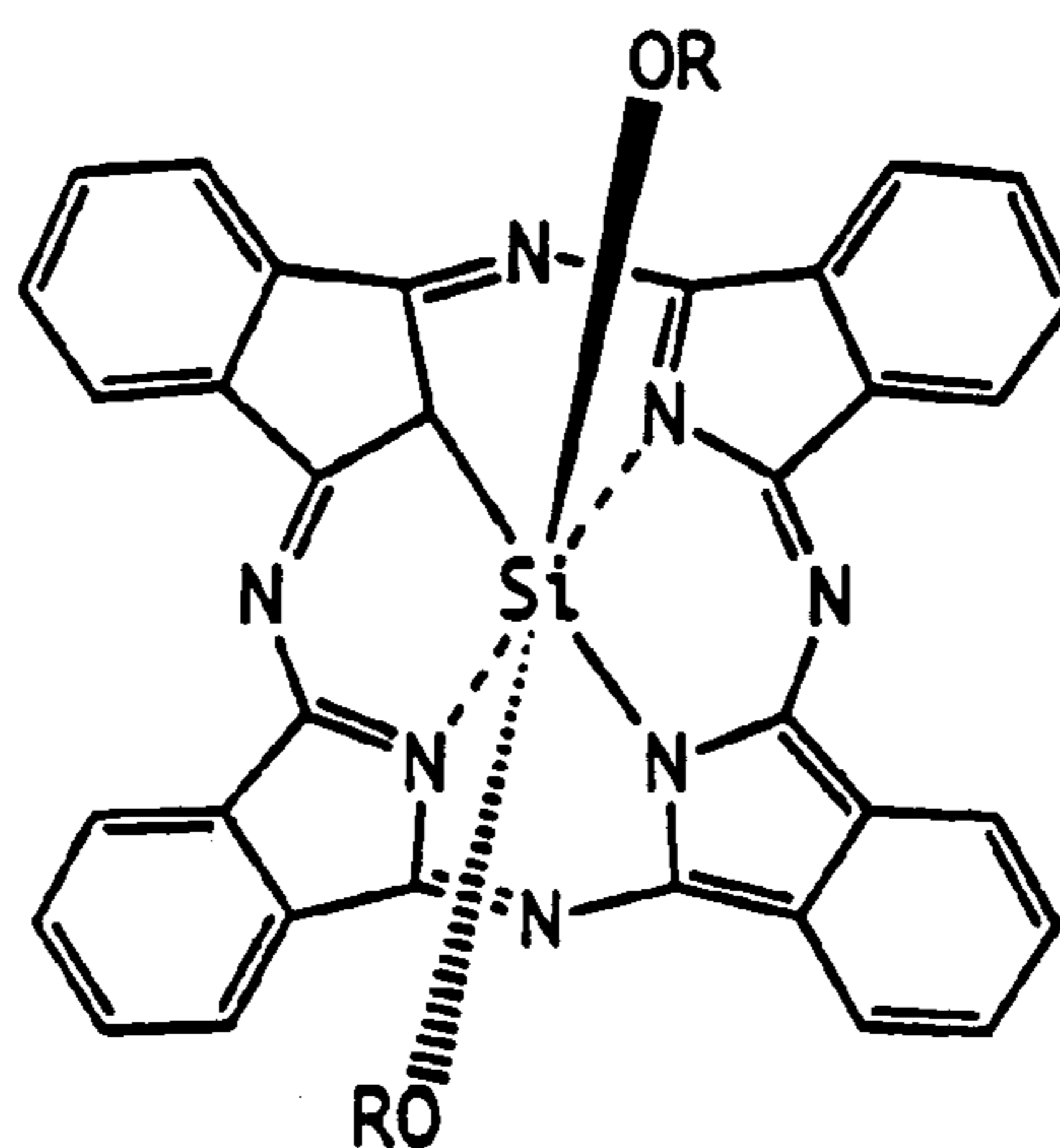
SILICON PHTHALOCYANINE
