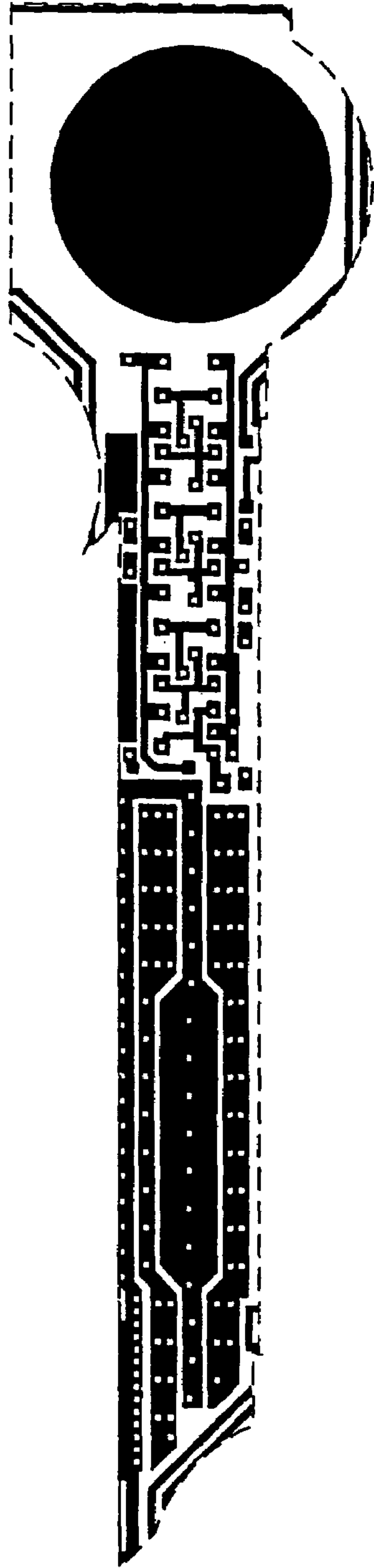
Metal 1 mask
