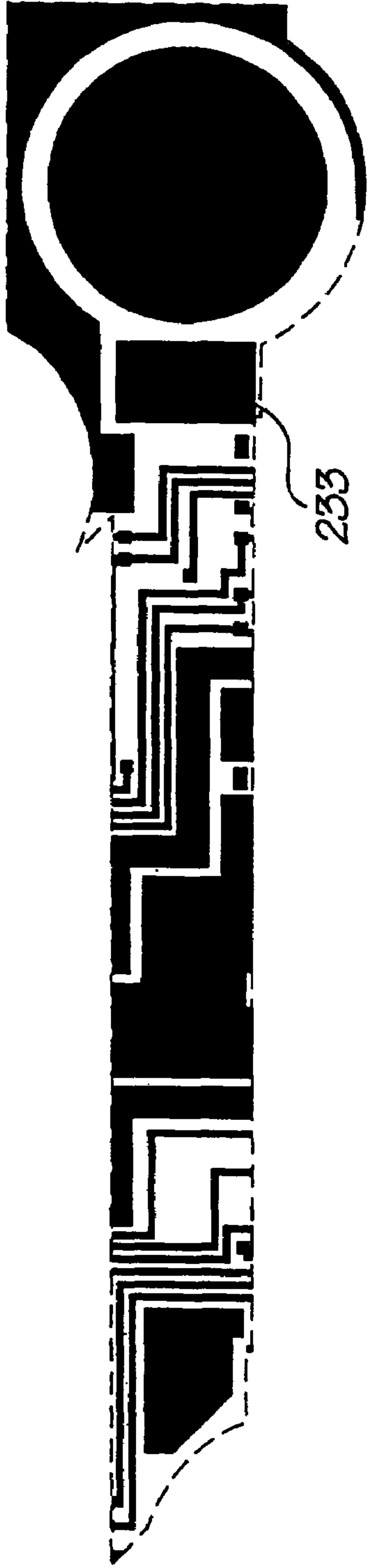
Metal 2 mask
