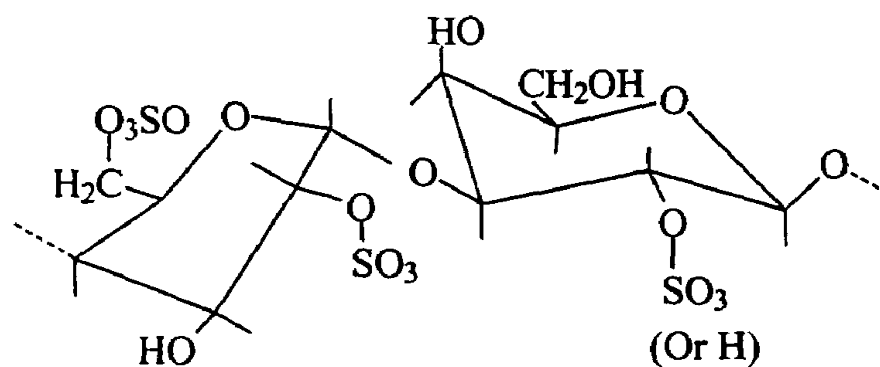
D-galactose-2,6-disulphate D-galactose-2-sulphate
