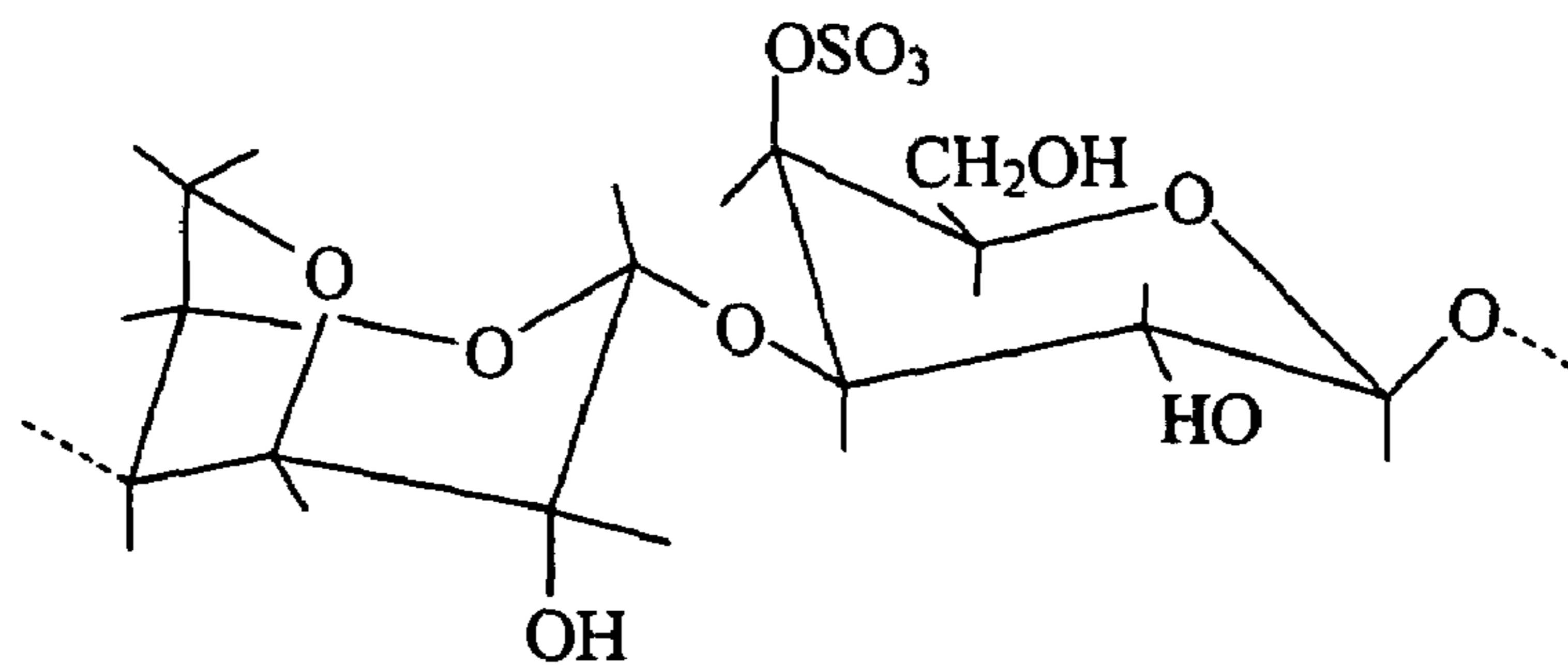
3,6-anhydro-D-galactose D-galactose-4-sulphate
