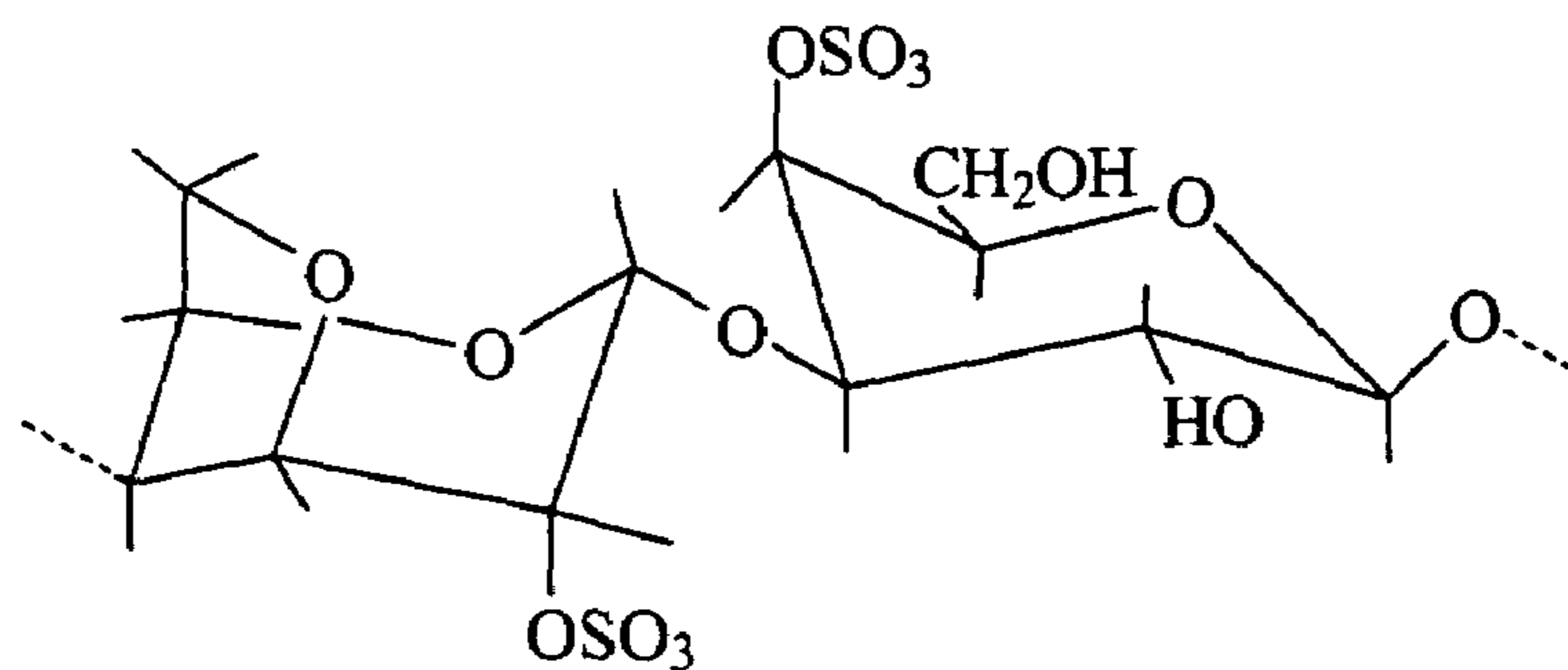
3,6-anhydro-D-galactose-2-Sulphate D-galactose-4-sulphate
