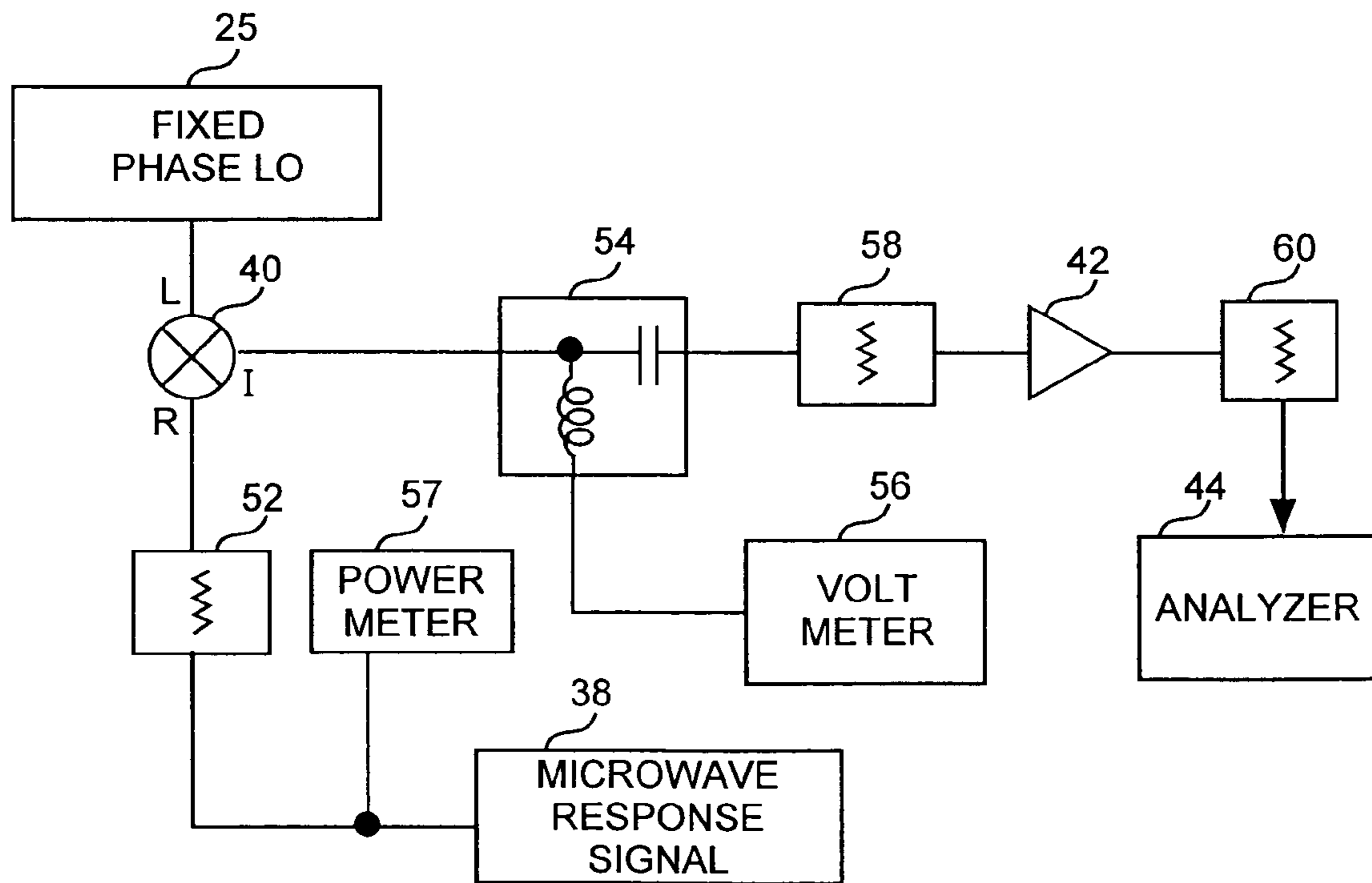
BASEBAND TIME-DOMAIN RECEIVER
