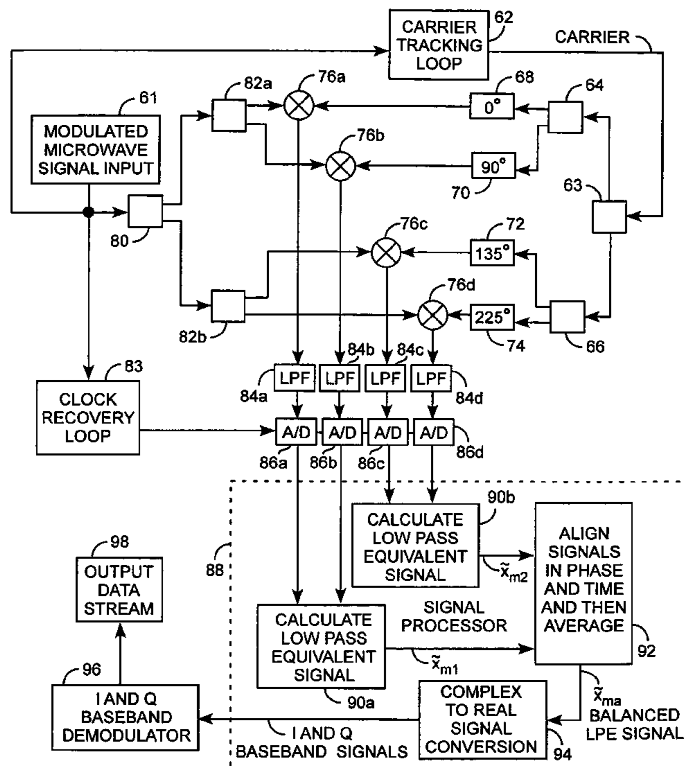
BALANCED BASEBAND RECEIVER SYSTEM
