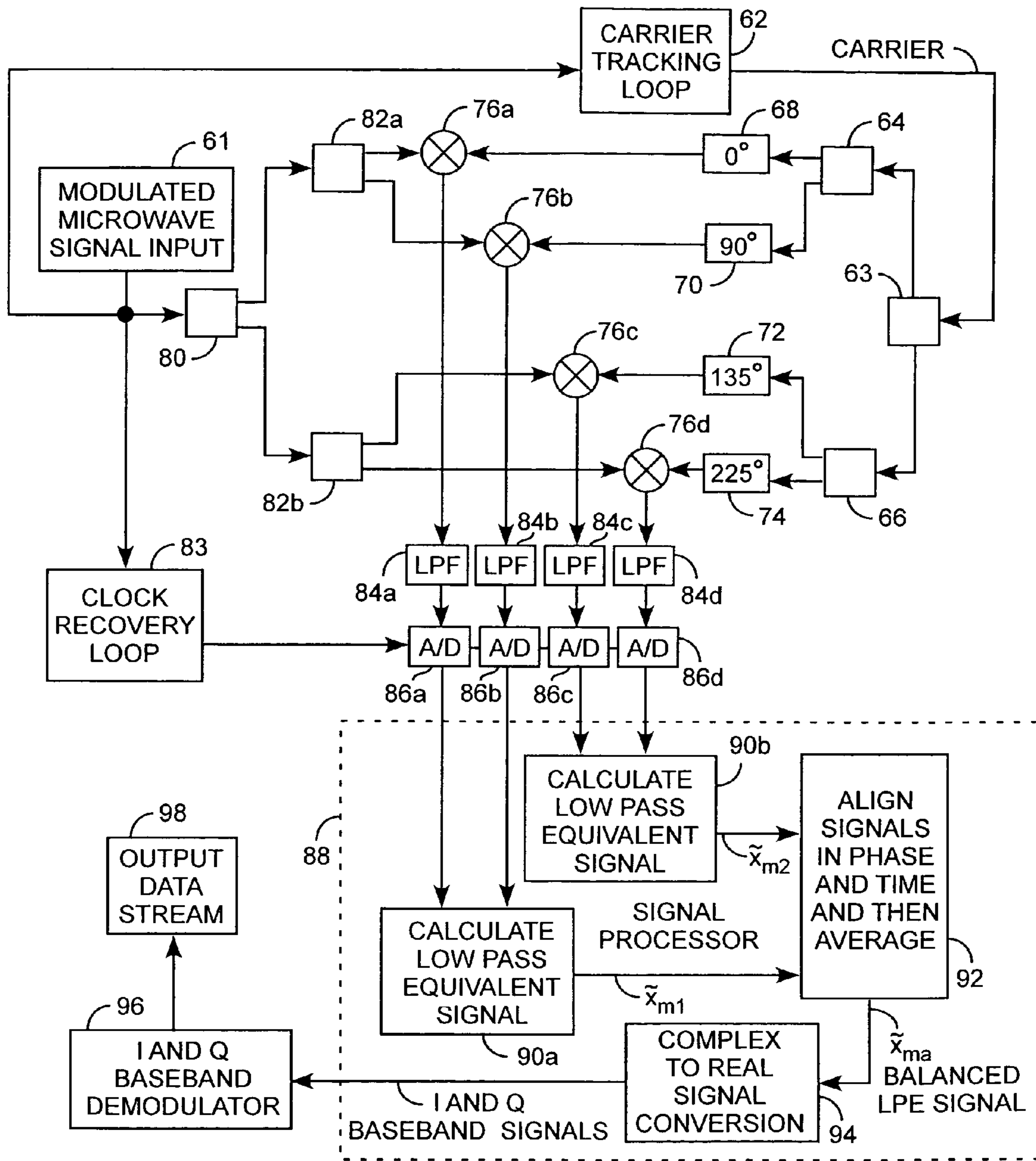
BALANCED BASEBAND RECEIVER SYSTEM
