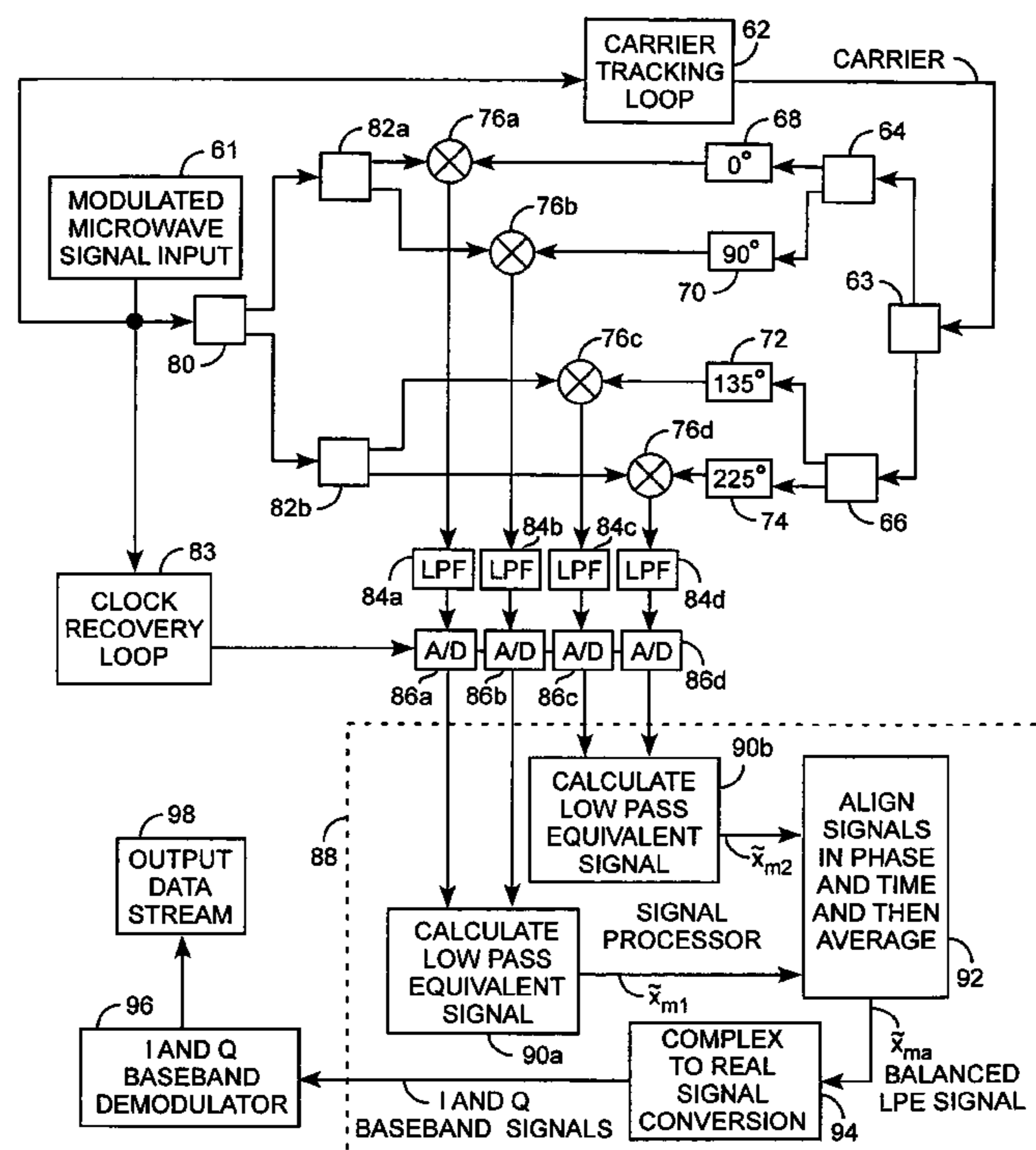
BALANCED BASEBAND RECEIVER SYSTEM
