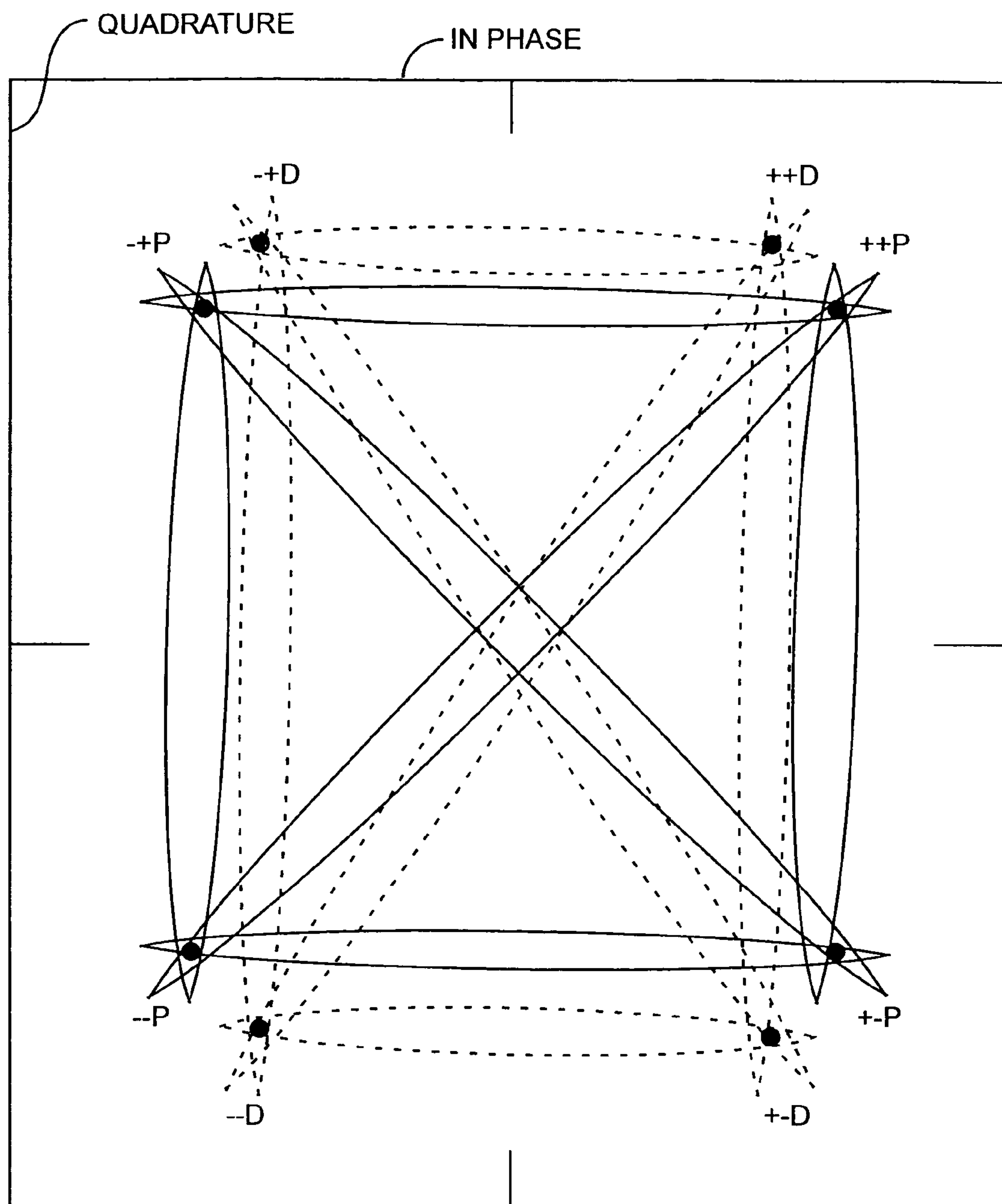
IDEAL &amp; DISTORTED QPSK CONSTELLATION PLOT
