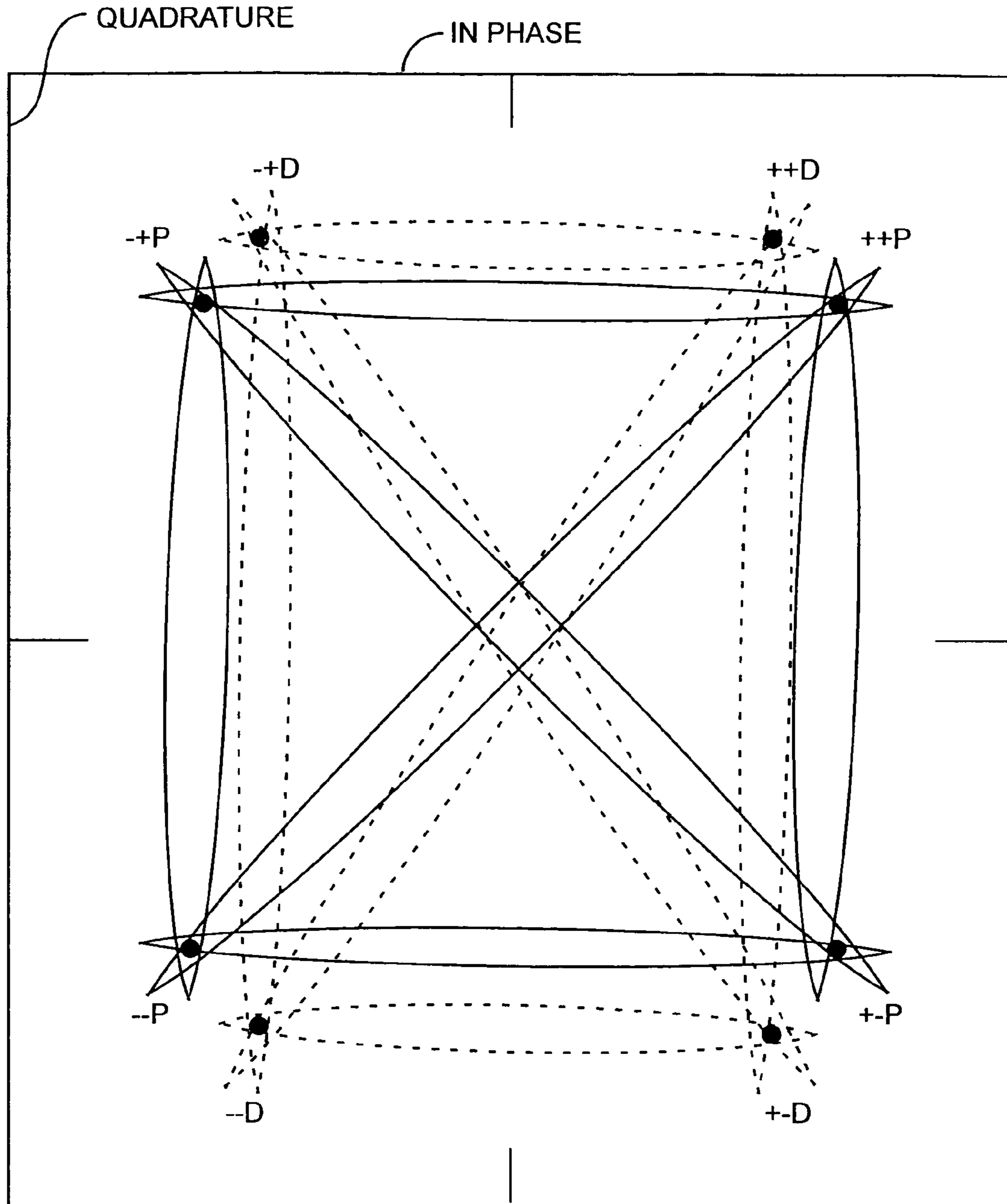
IDEAL & DISTORTED QPSK CONSTELLATION PLOT
