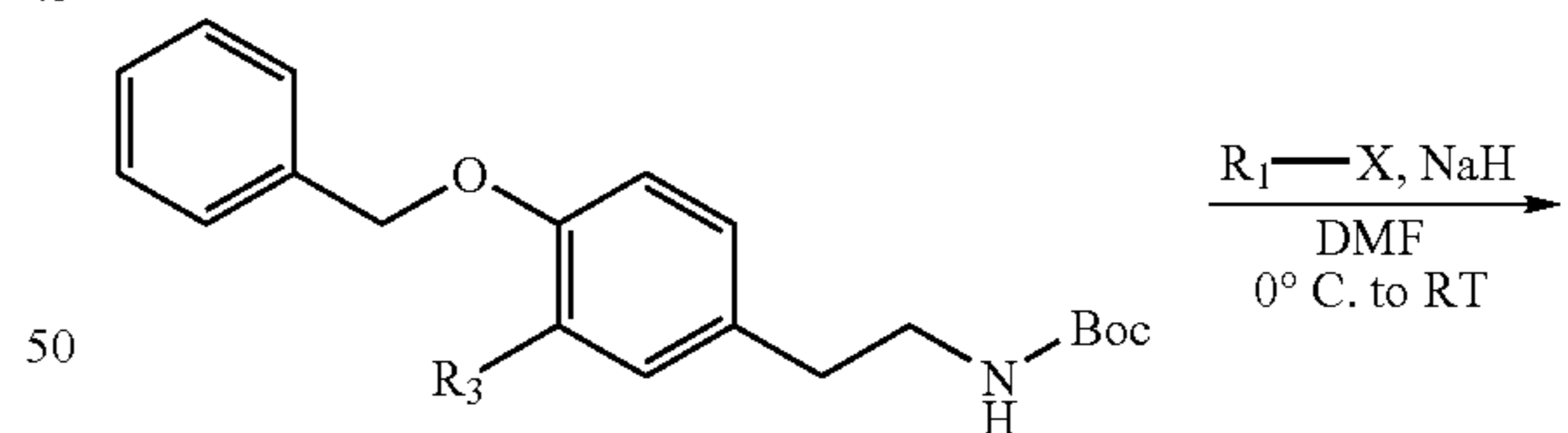
Scheme 6: Synthesis of N-Alkylated Derivatives
