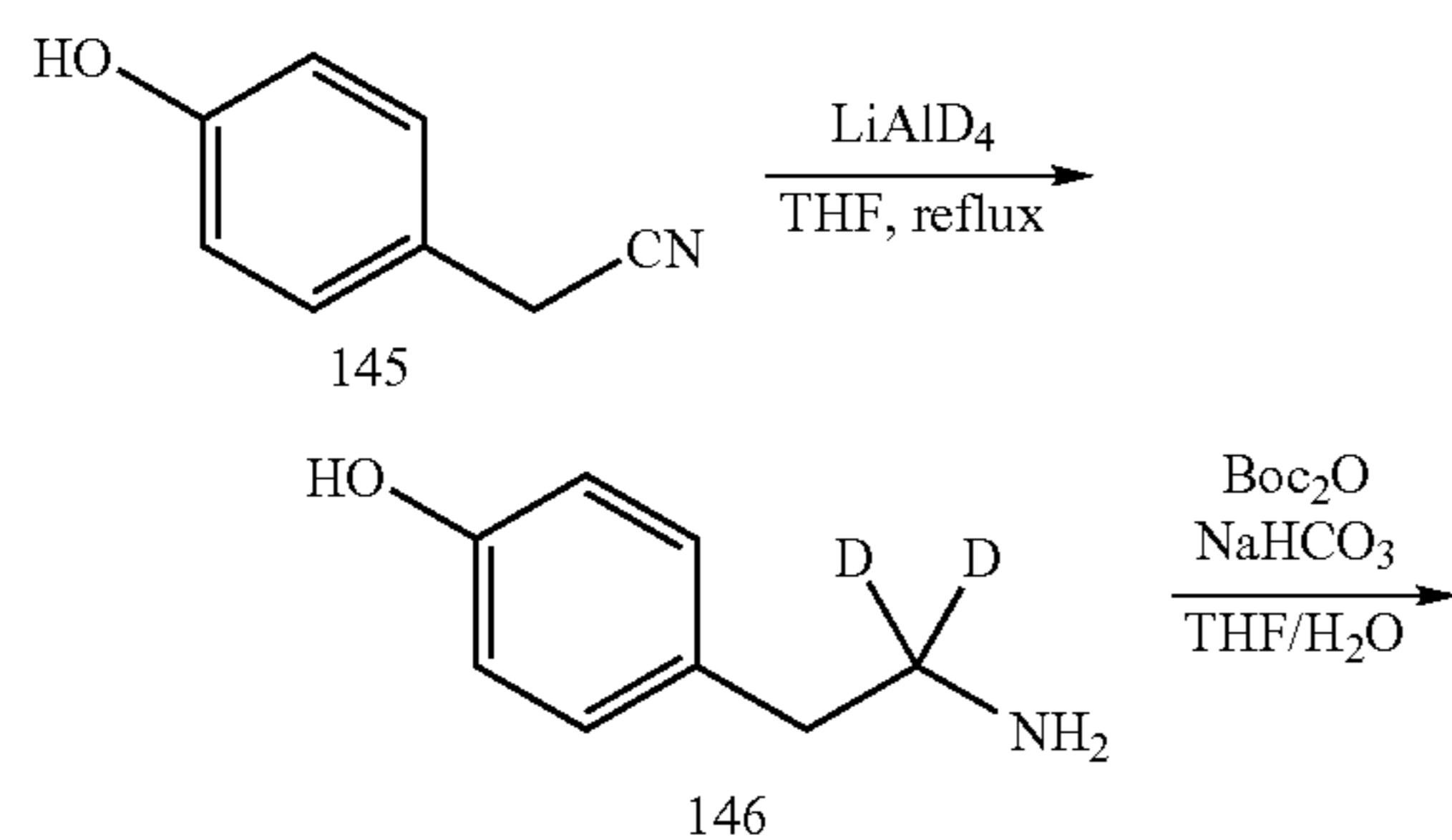
Scheme 17: Synthesis of [ ^2\text{H} , ^2\text{H} ]-N-t-Boc-Tyramine
