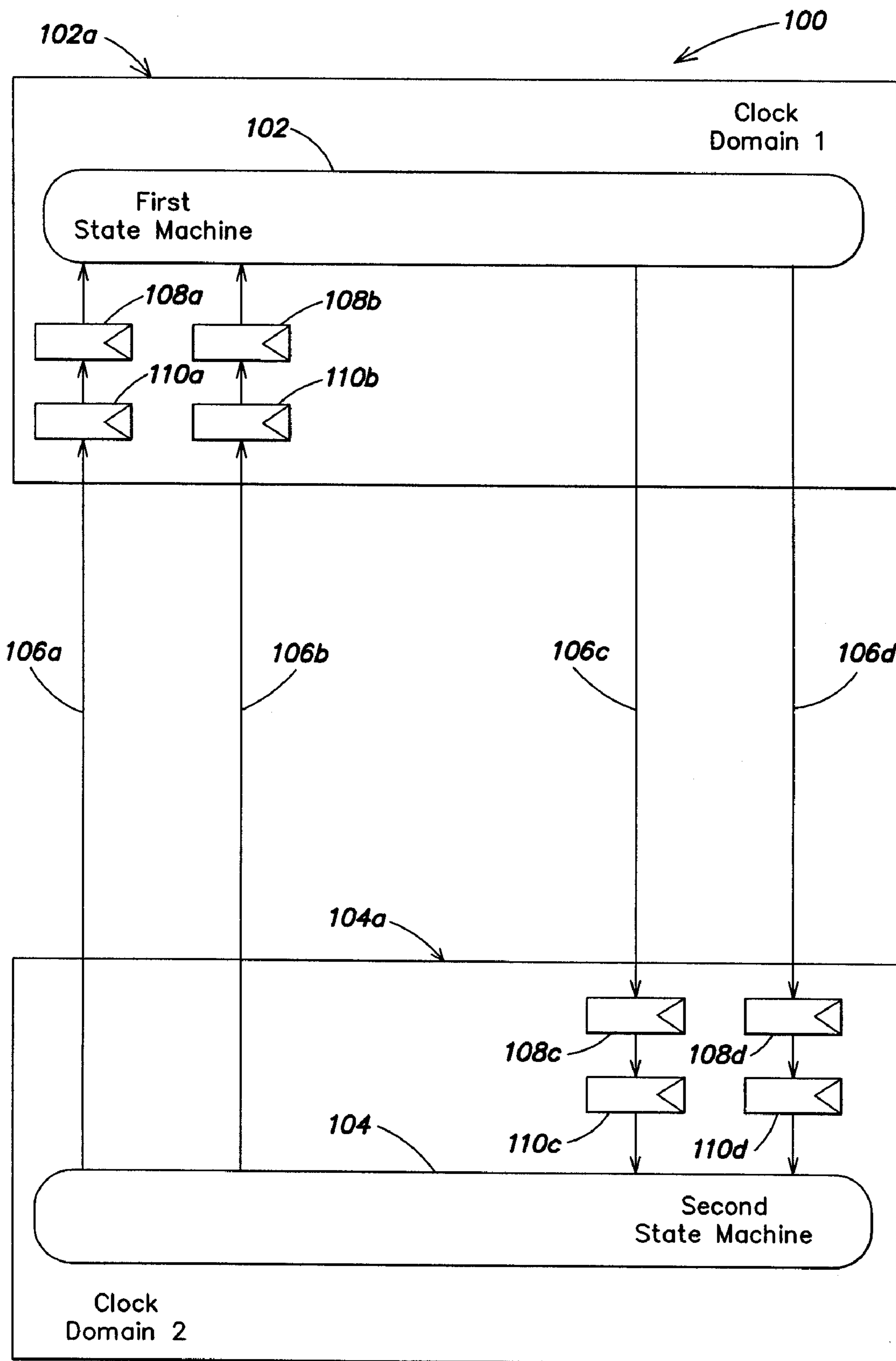
FIG. 1 (PRIOR ART)
