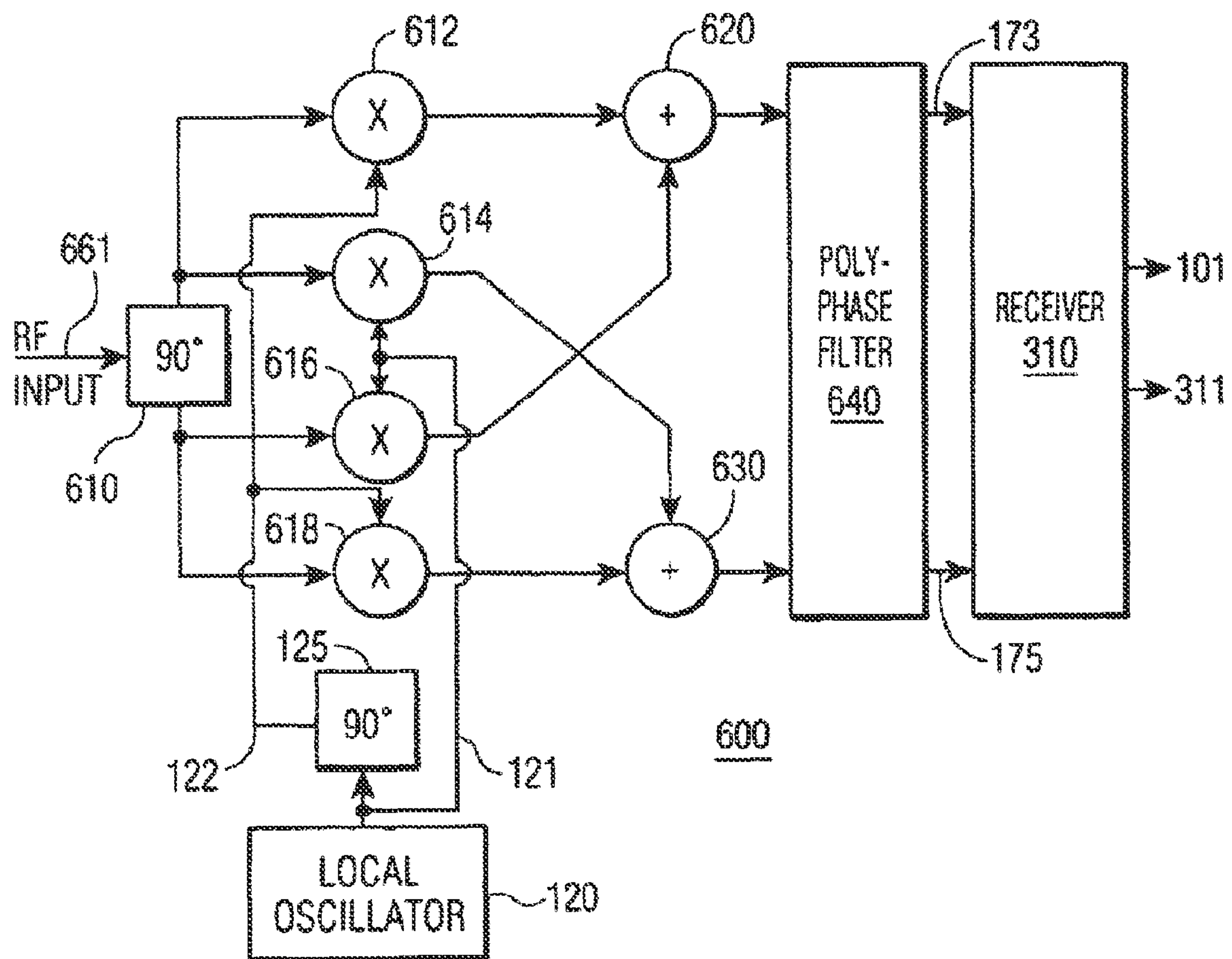
FIG. 6 (Prior Art)
