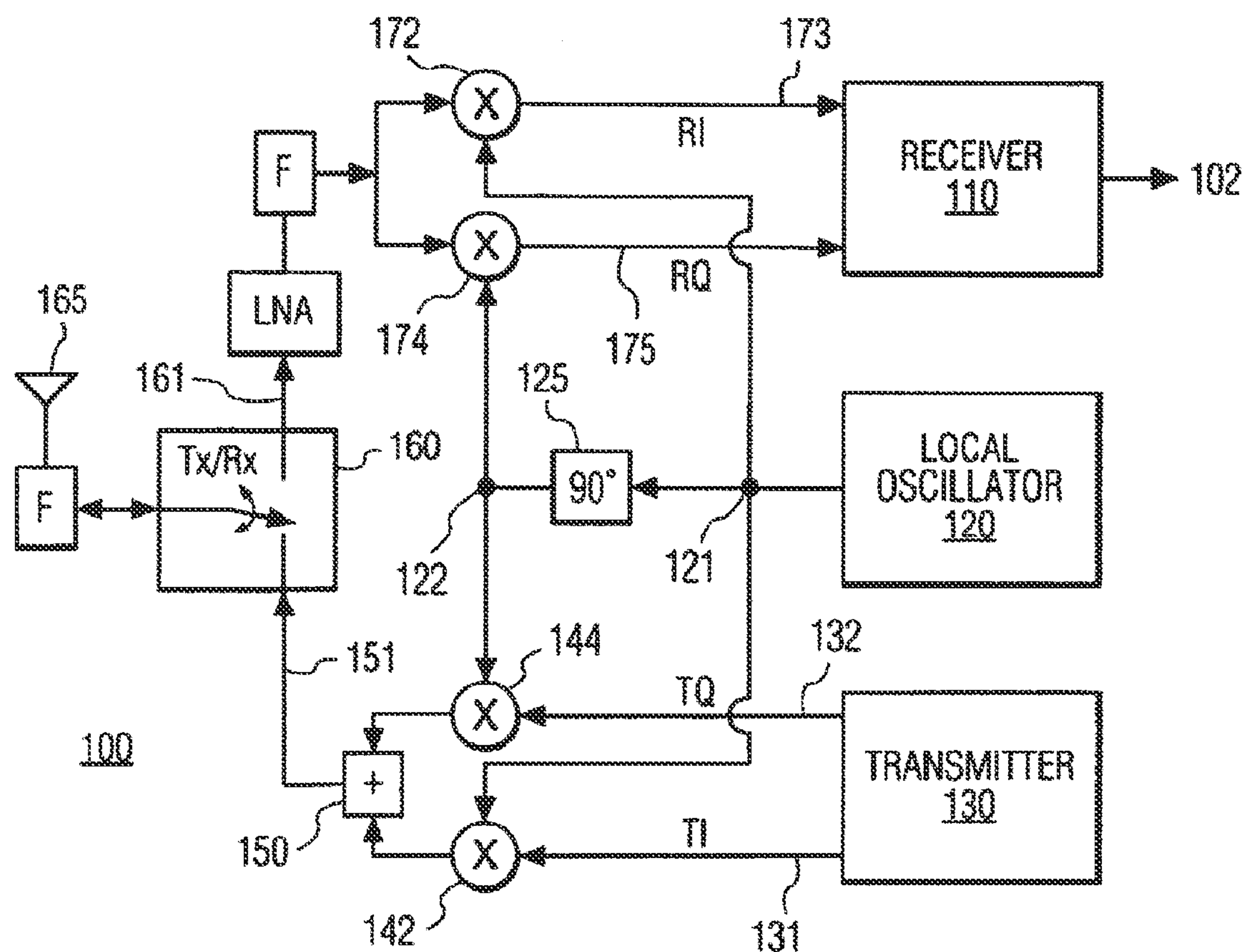
FIG. 1 PRIOR ART
