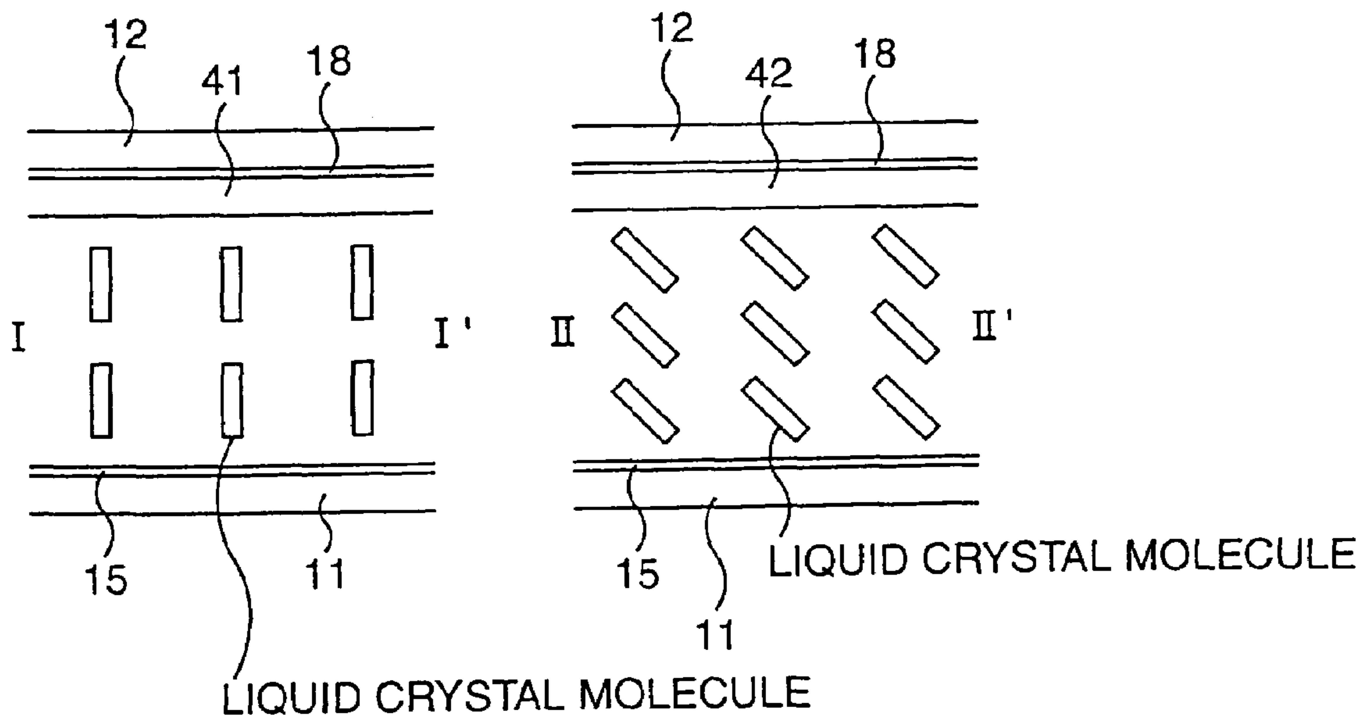
SECTIONAL VIEW
