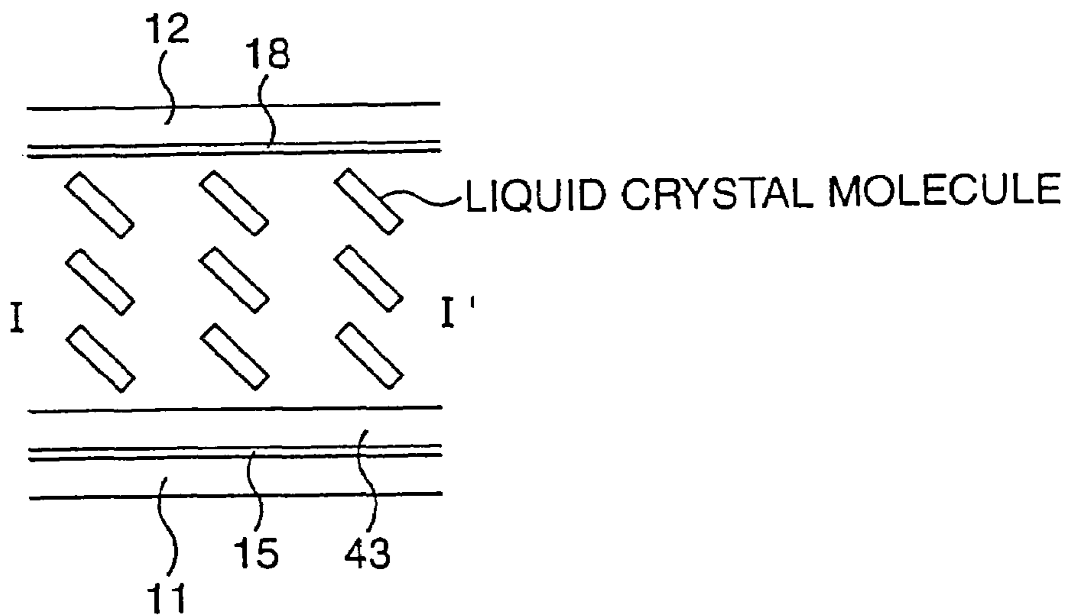
SECTIONAL VIEW
