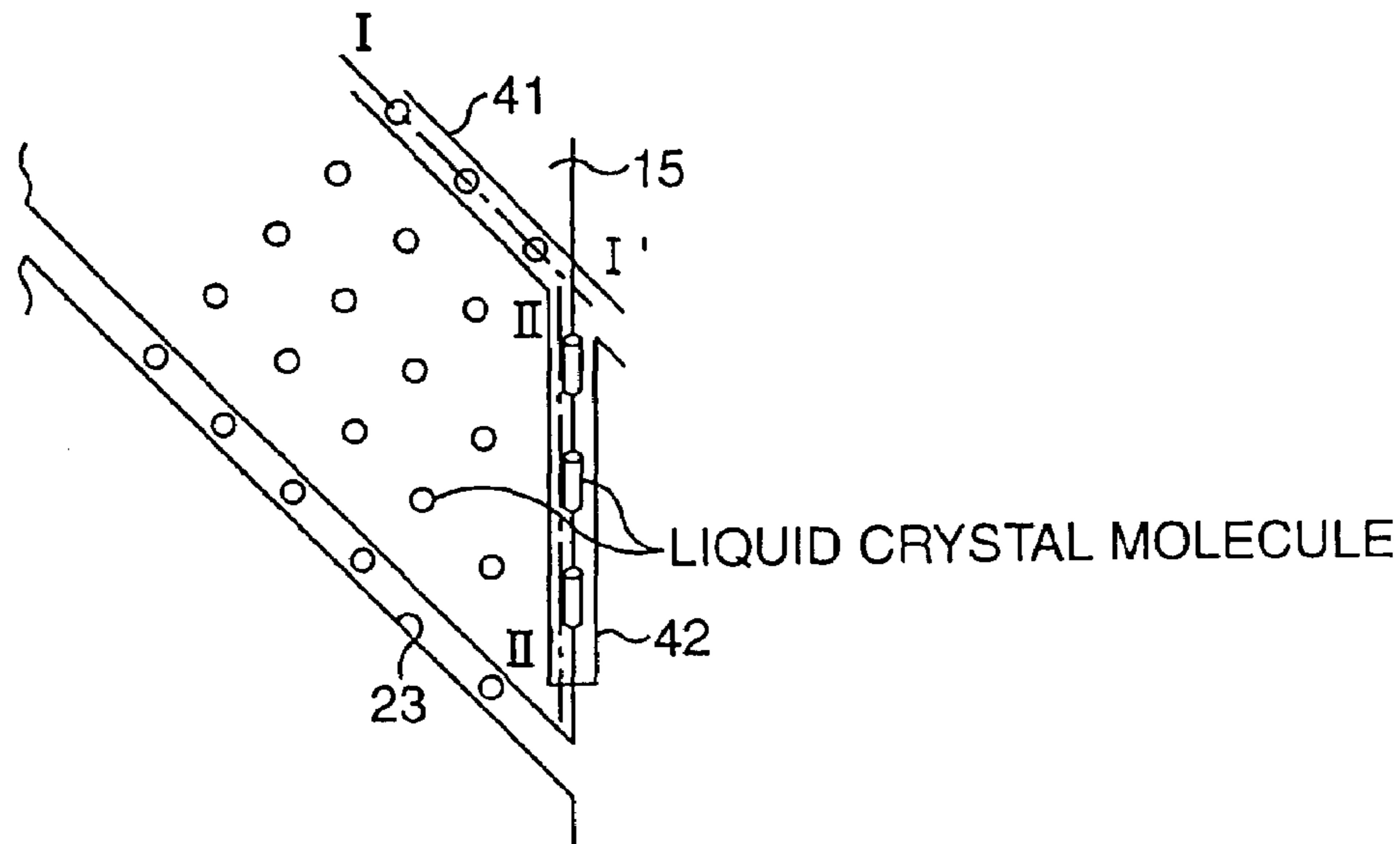
PLANE VIEW
