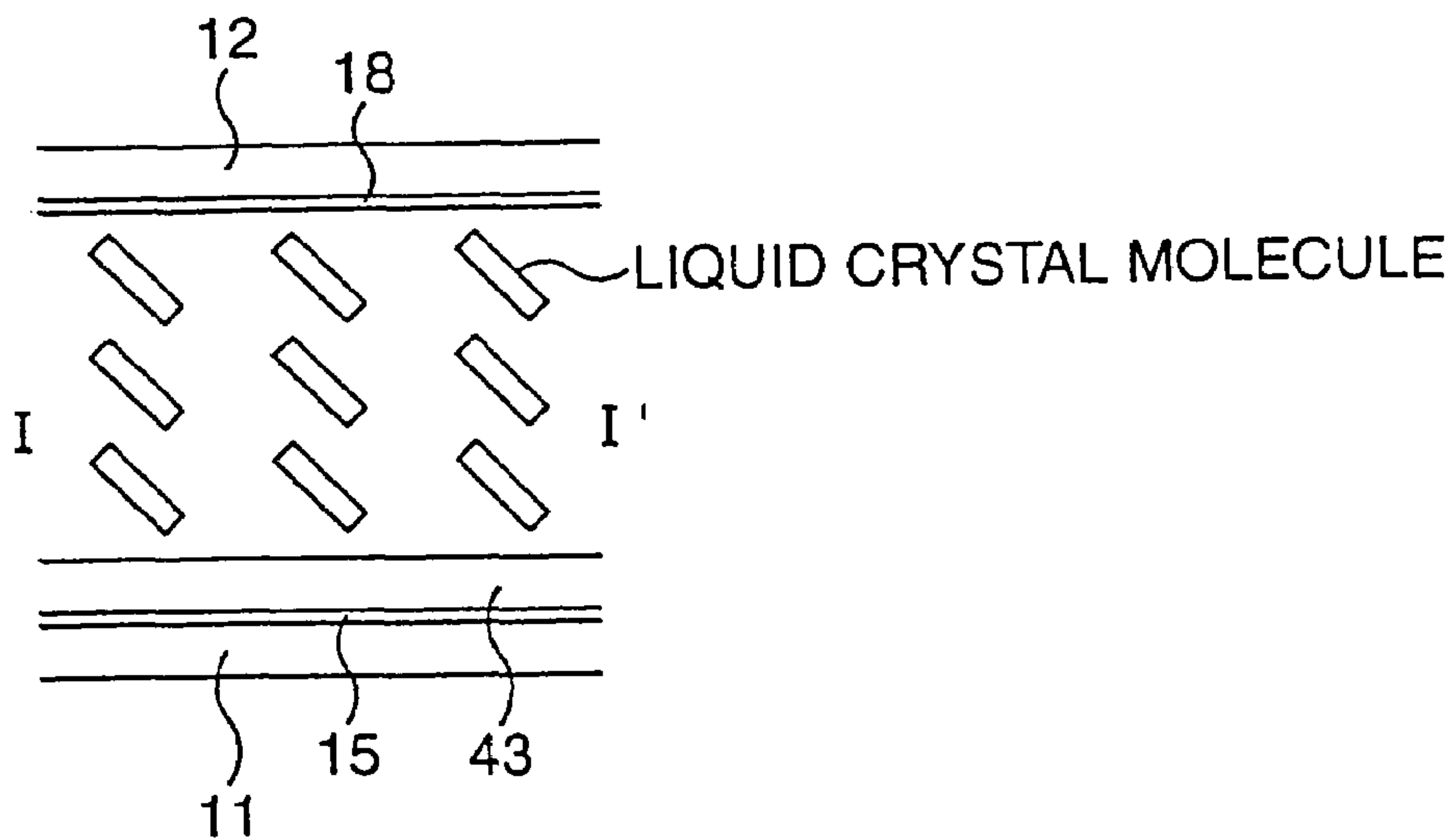
SECTIONAL VIEW
