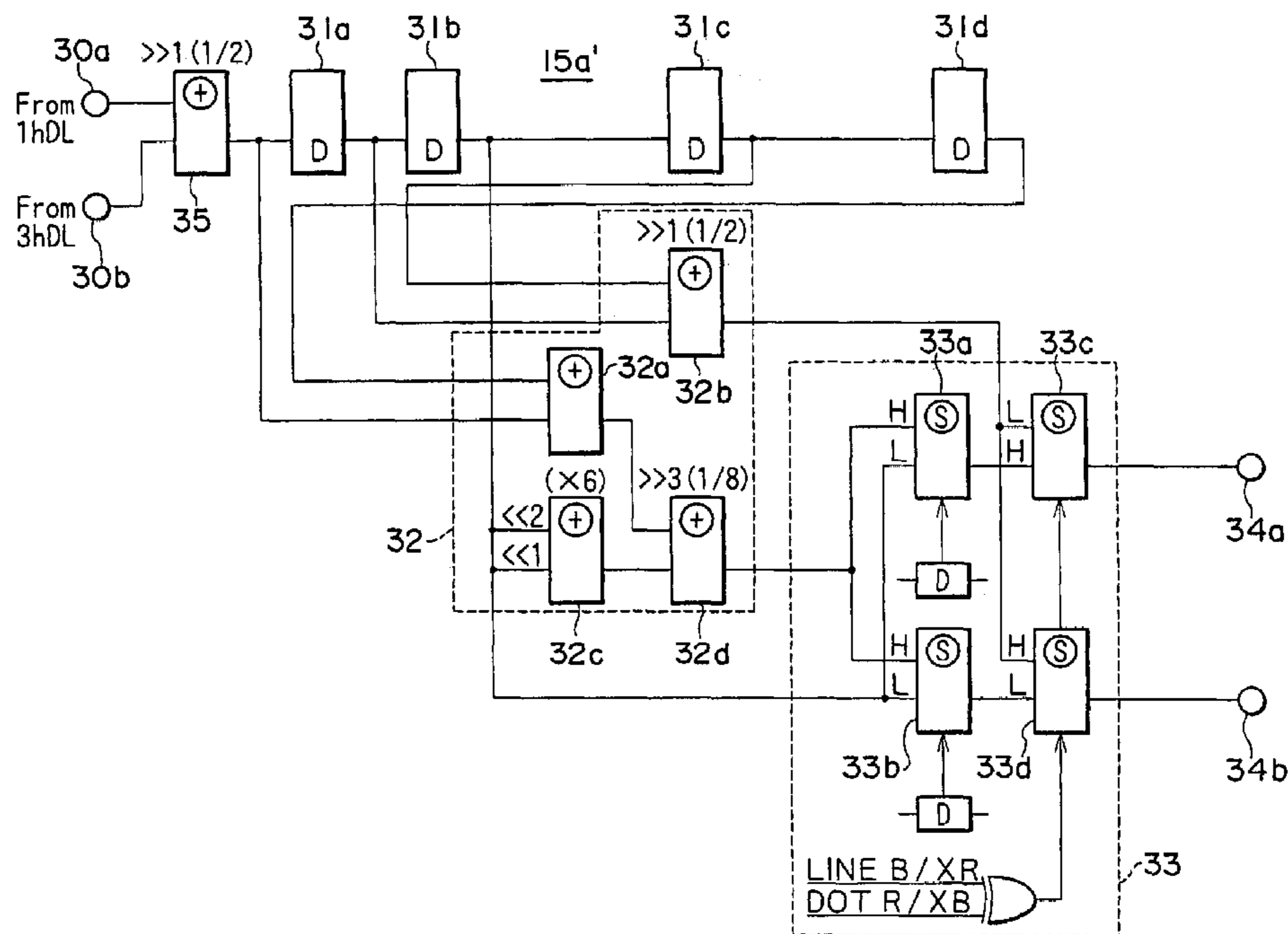
CONSTITUTION OF HORIZONTAL-DIRECTION INTERPOLATOR
