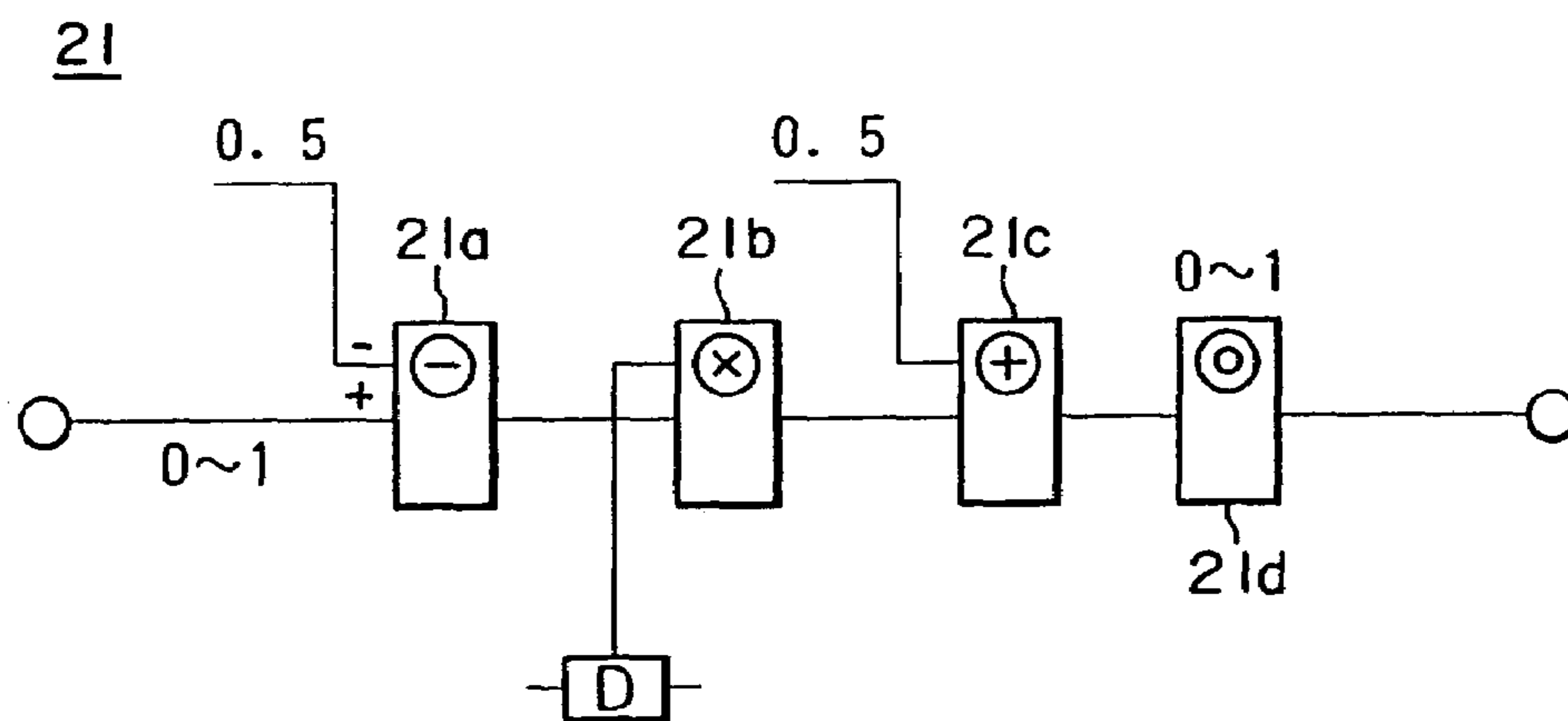
CONSTITUTION OF EMPHASIS/DEEMPHASIS CIRCUIT
