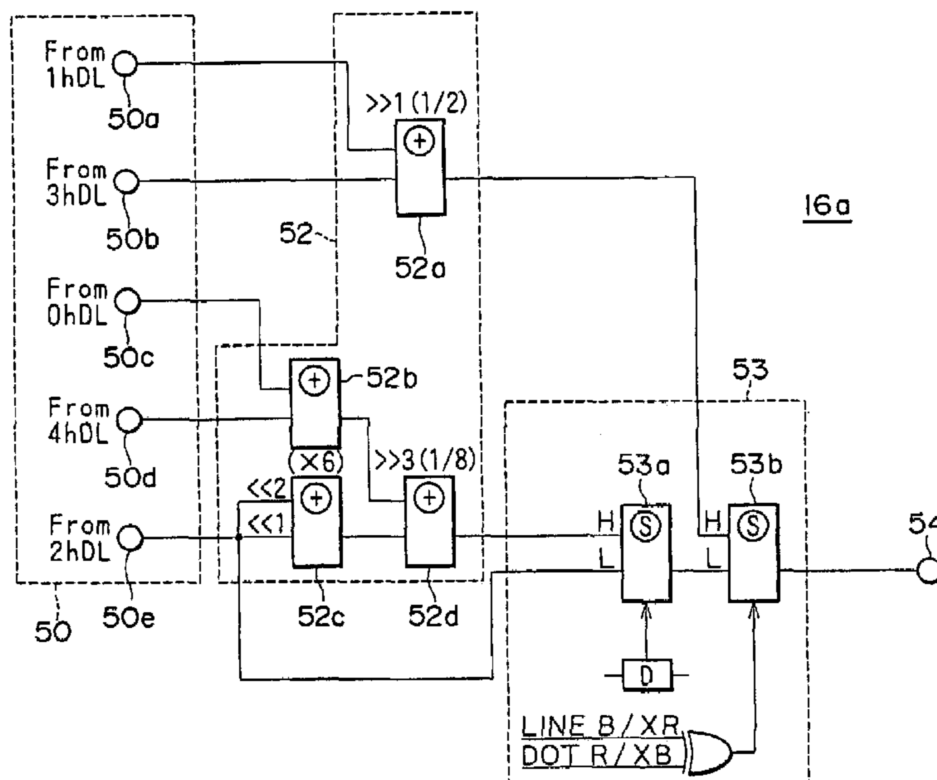
CONSTITUTION OF HORIZONTAL-DIRECTION CORRELATION DETECTOR
