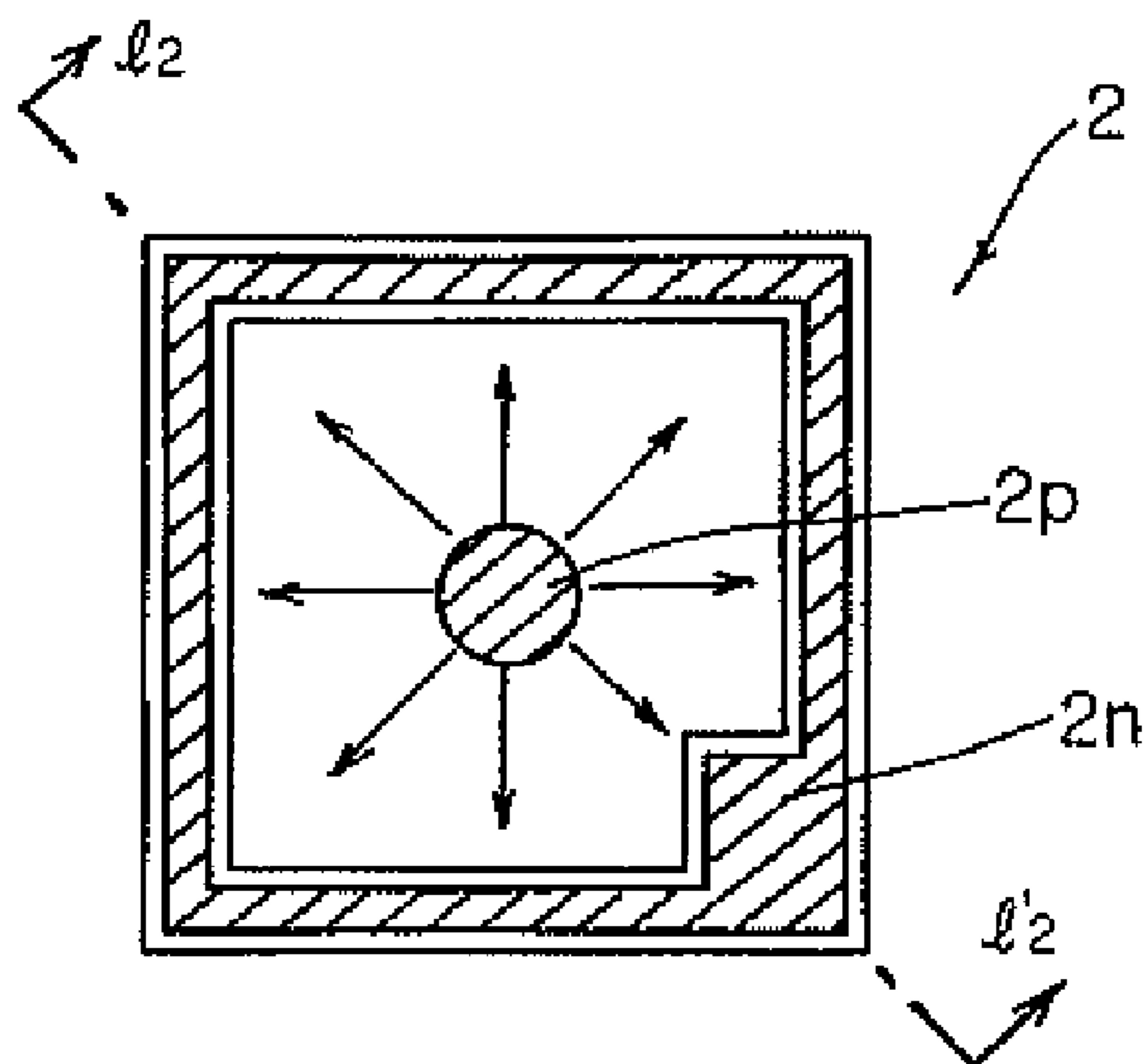
PRIOR ART FIG. 2a
