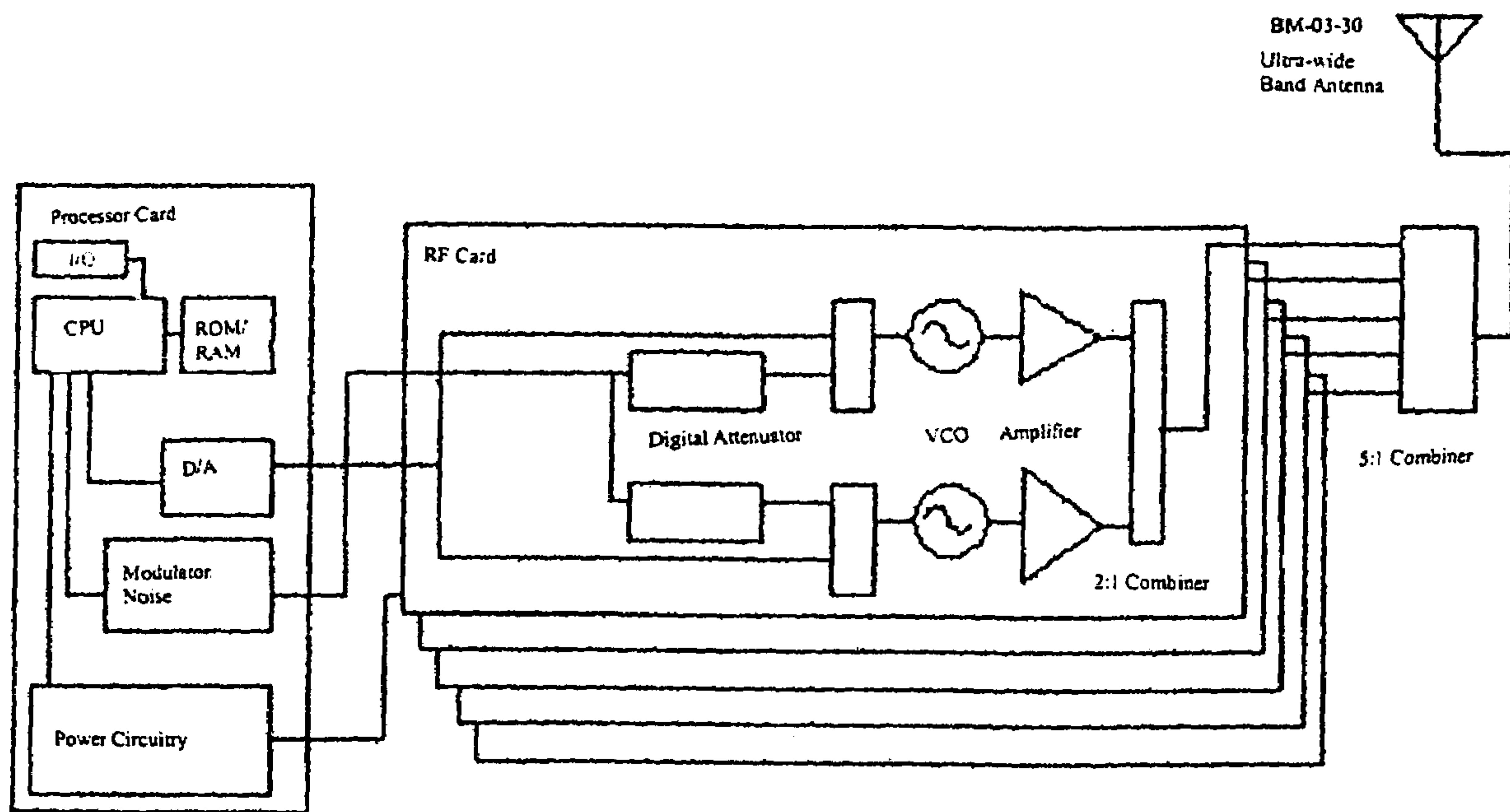
SSVJ Block Diagram
