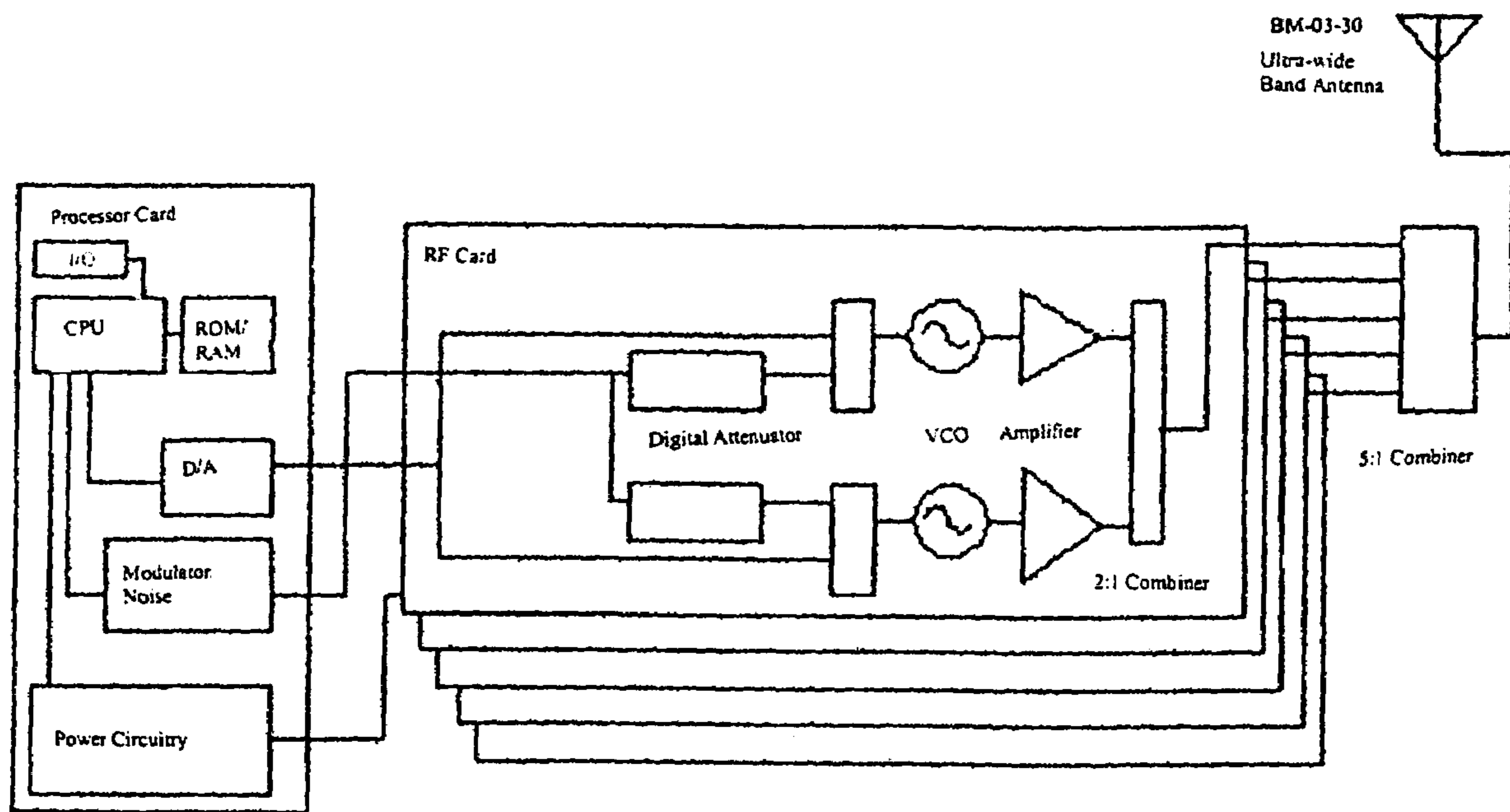
SSVJ Block Diagram
