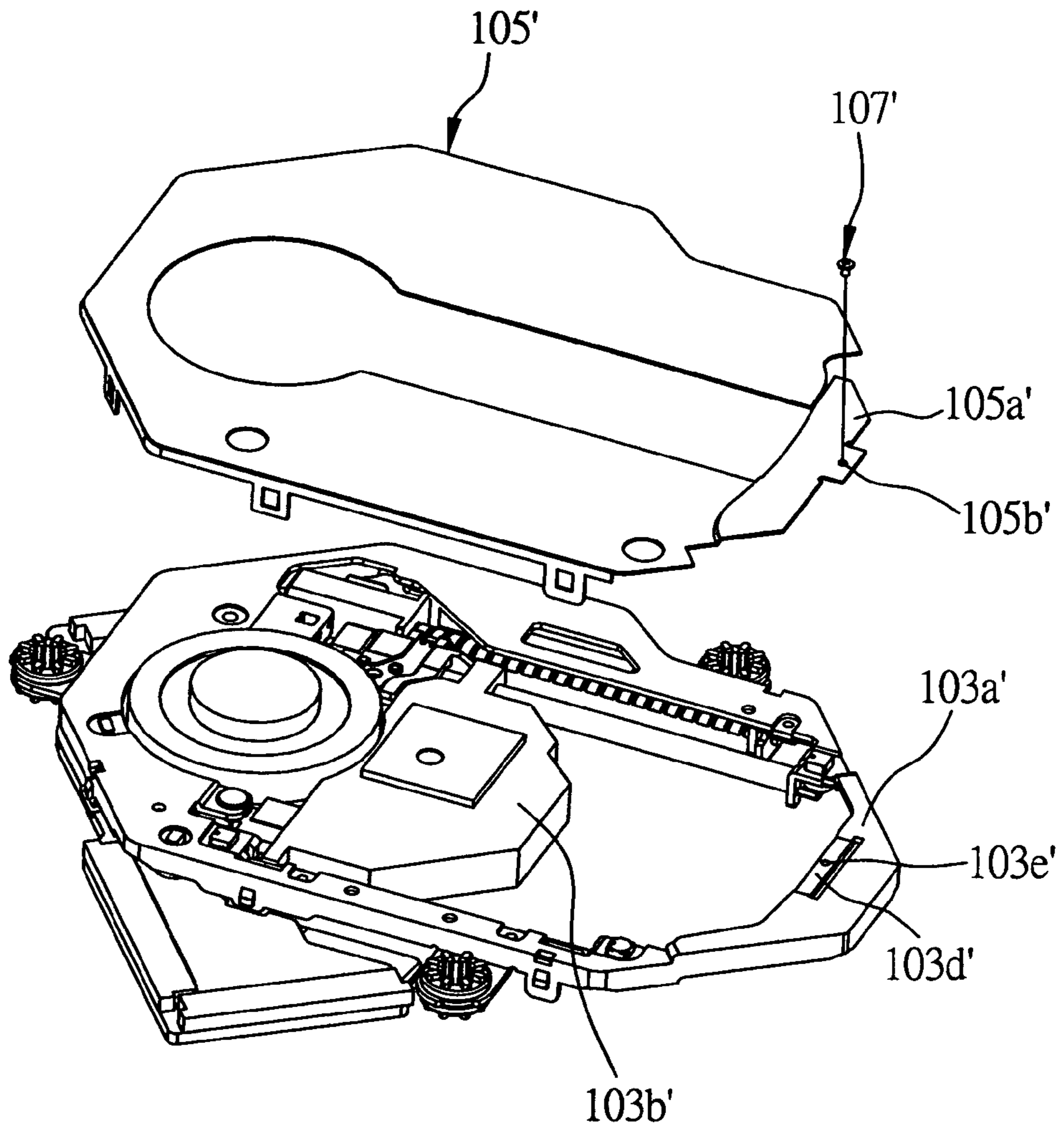
FIG. 10 (PRIOR ART)
