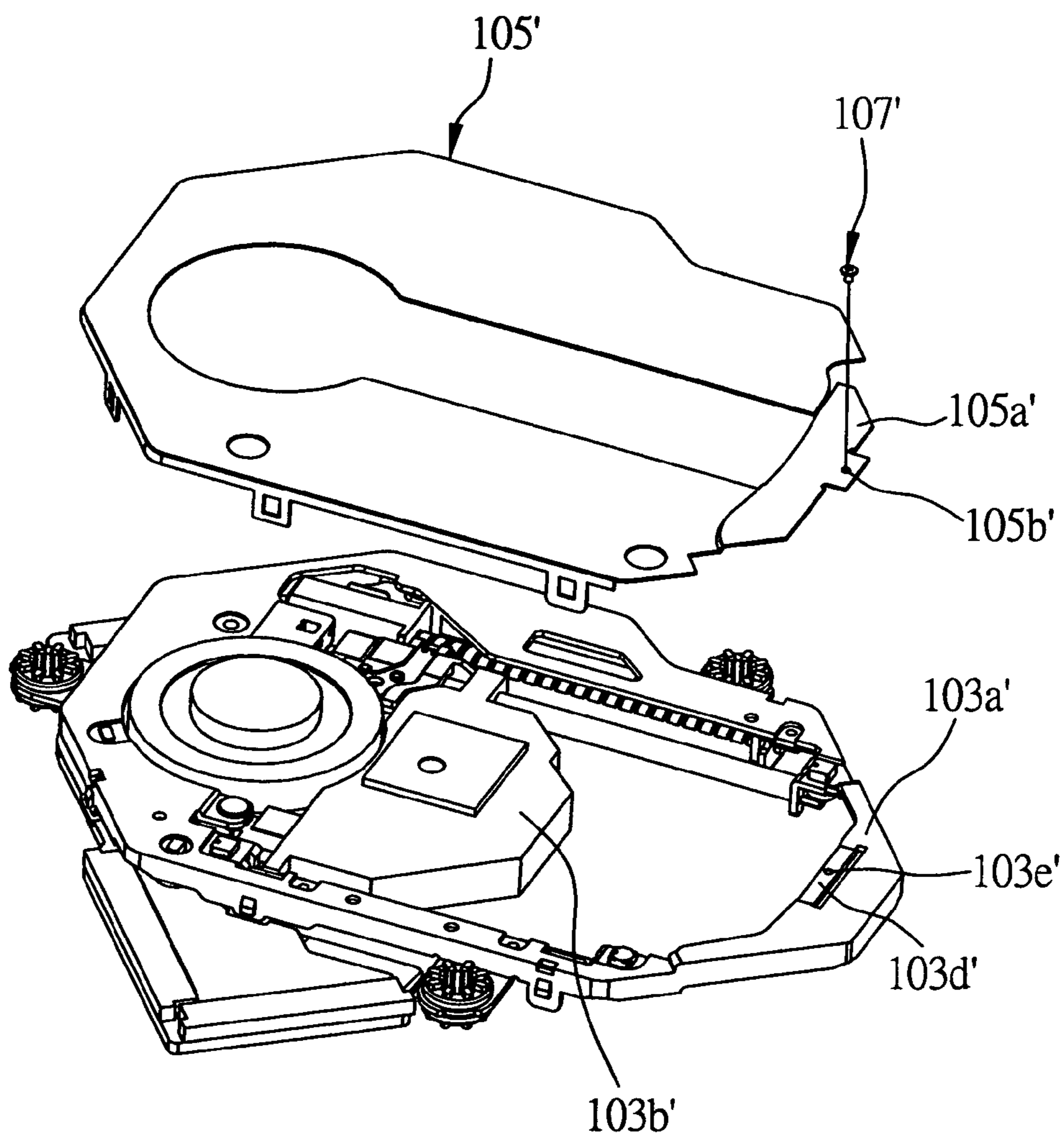
FIG. 10 (PRIOR ART)
