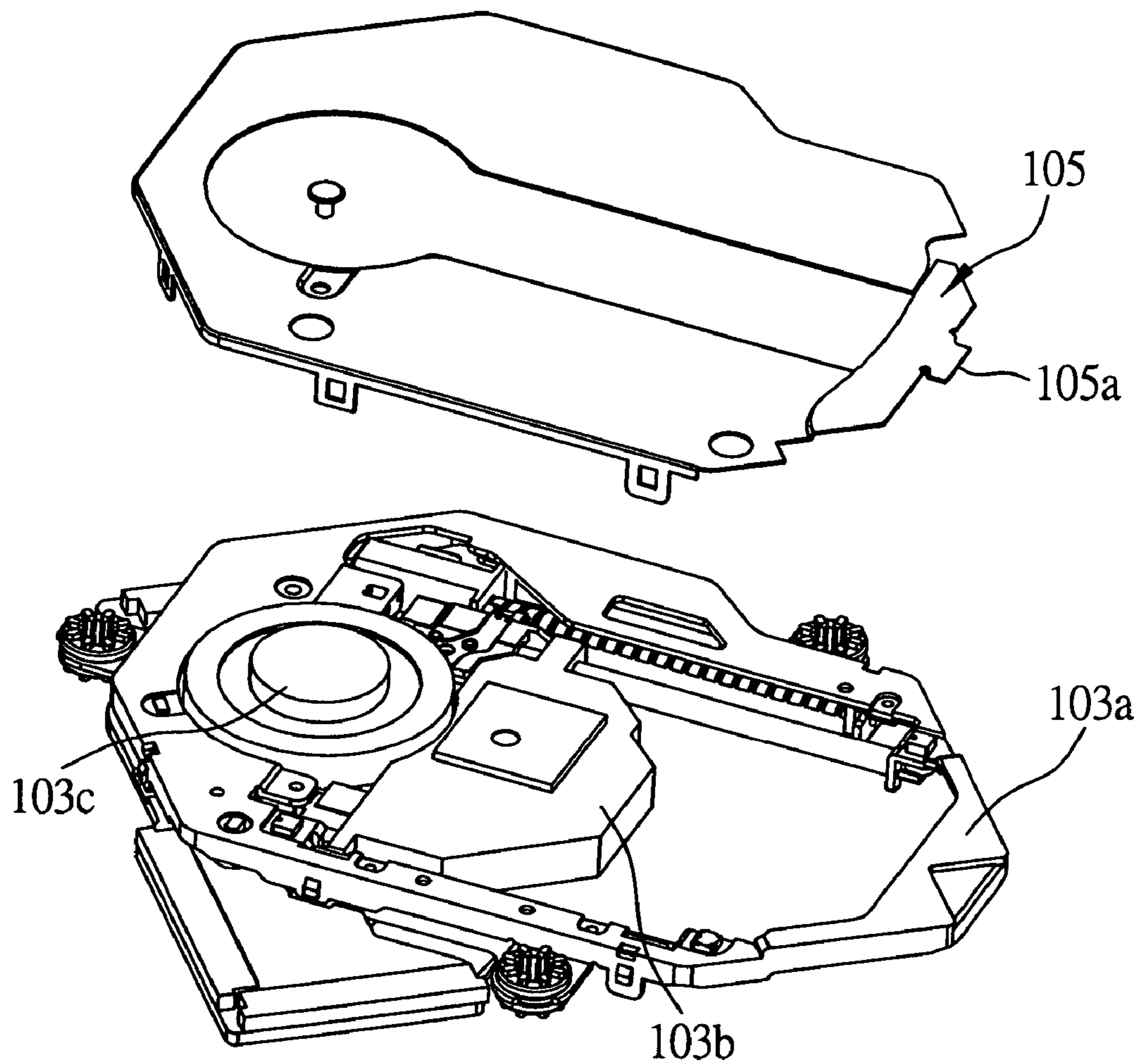
FIG. 8 (PRIOR ART)
