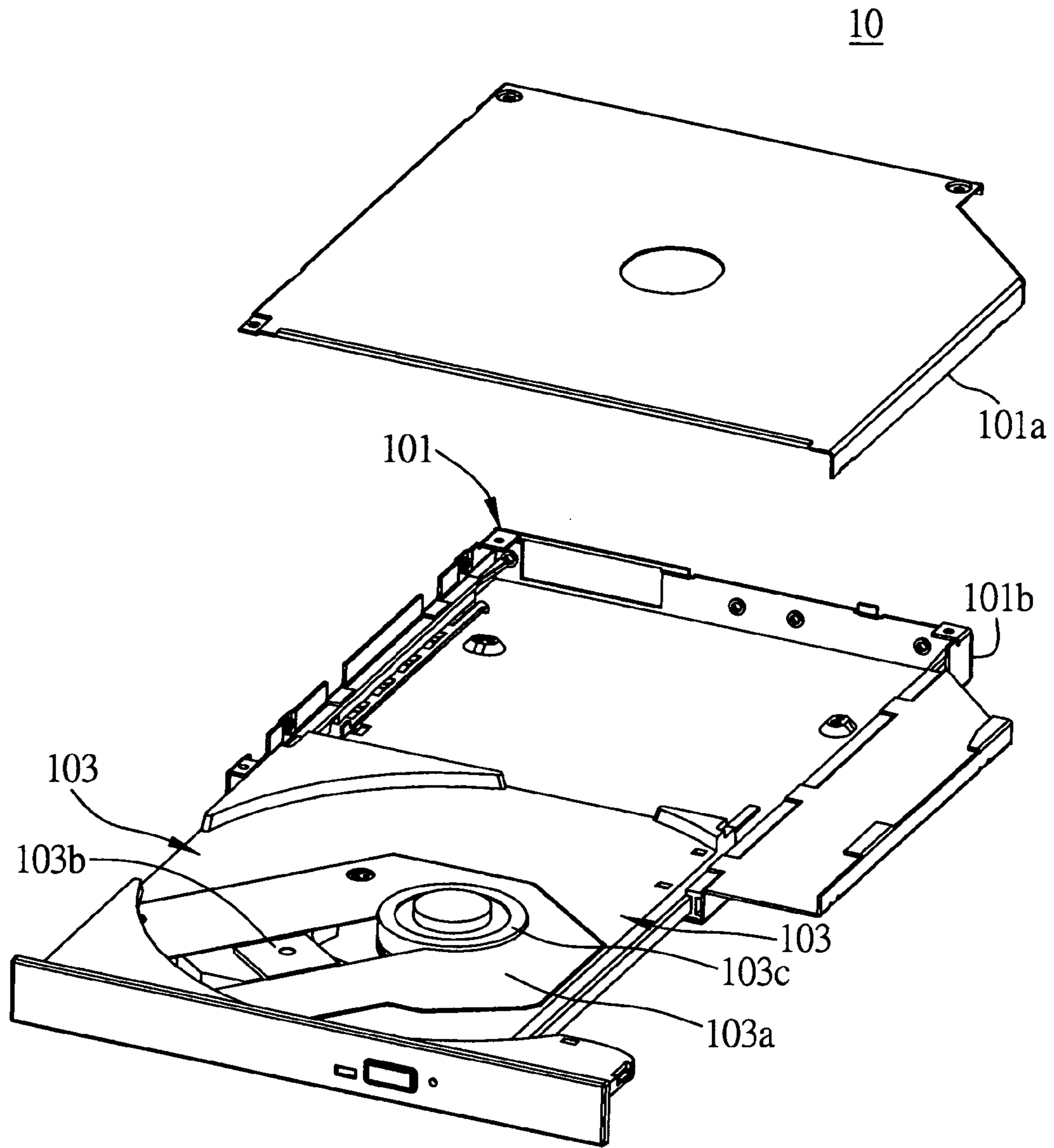
FIG. 7 (PRIOR ART)
