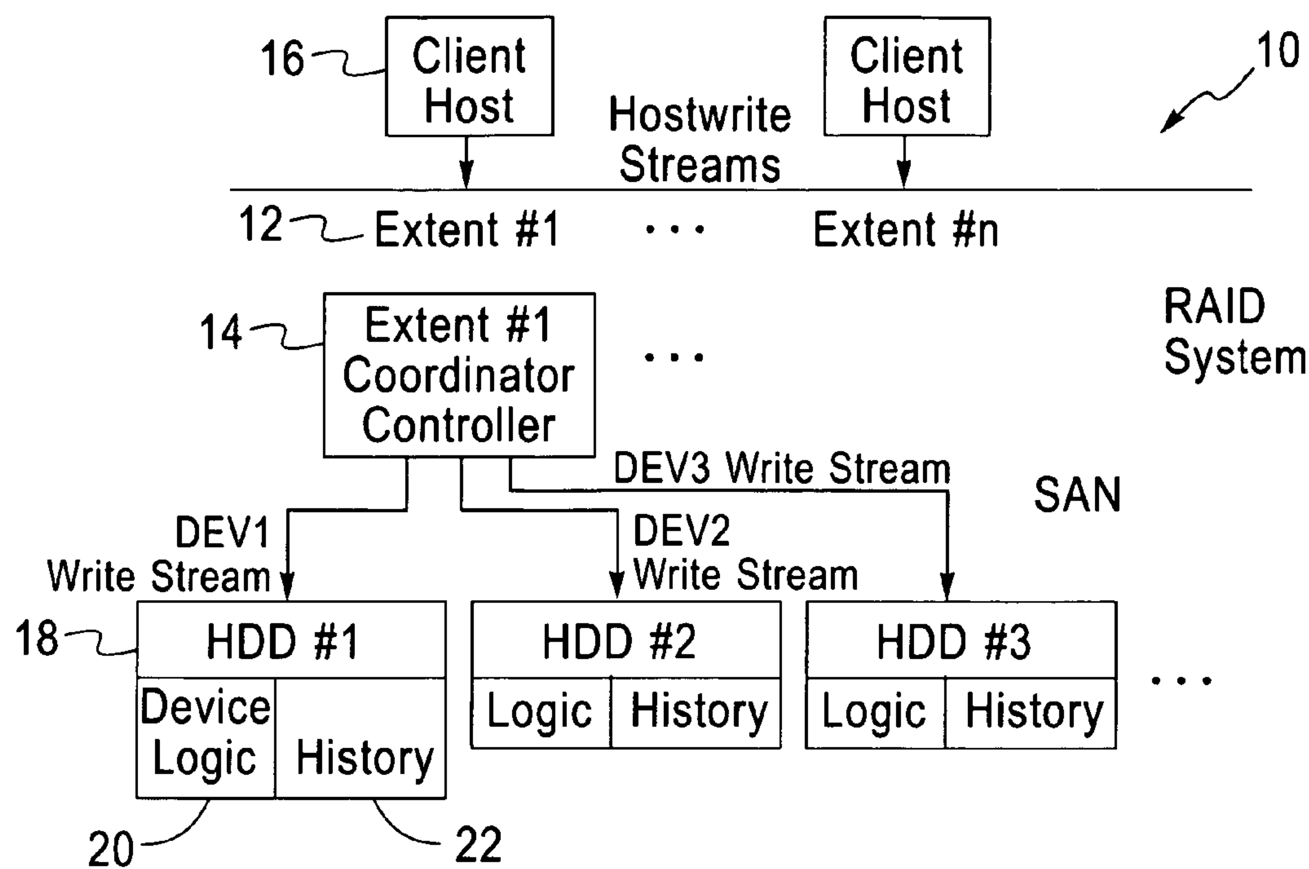
Fig. 1 System
