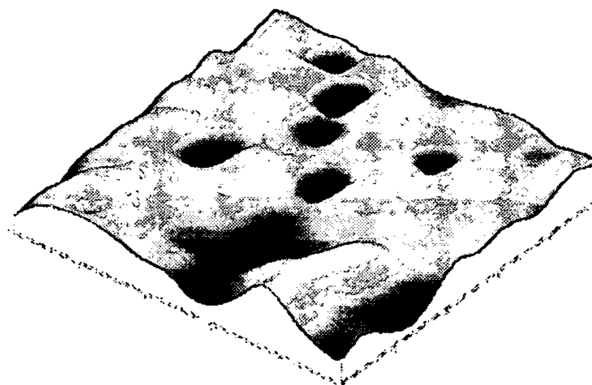
The surface of the UV curable resins with the thickness of 80nm on PET substrates.
