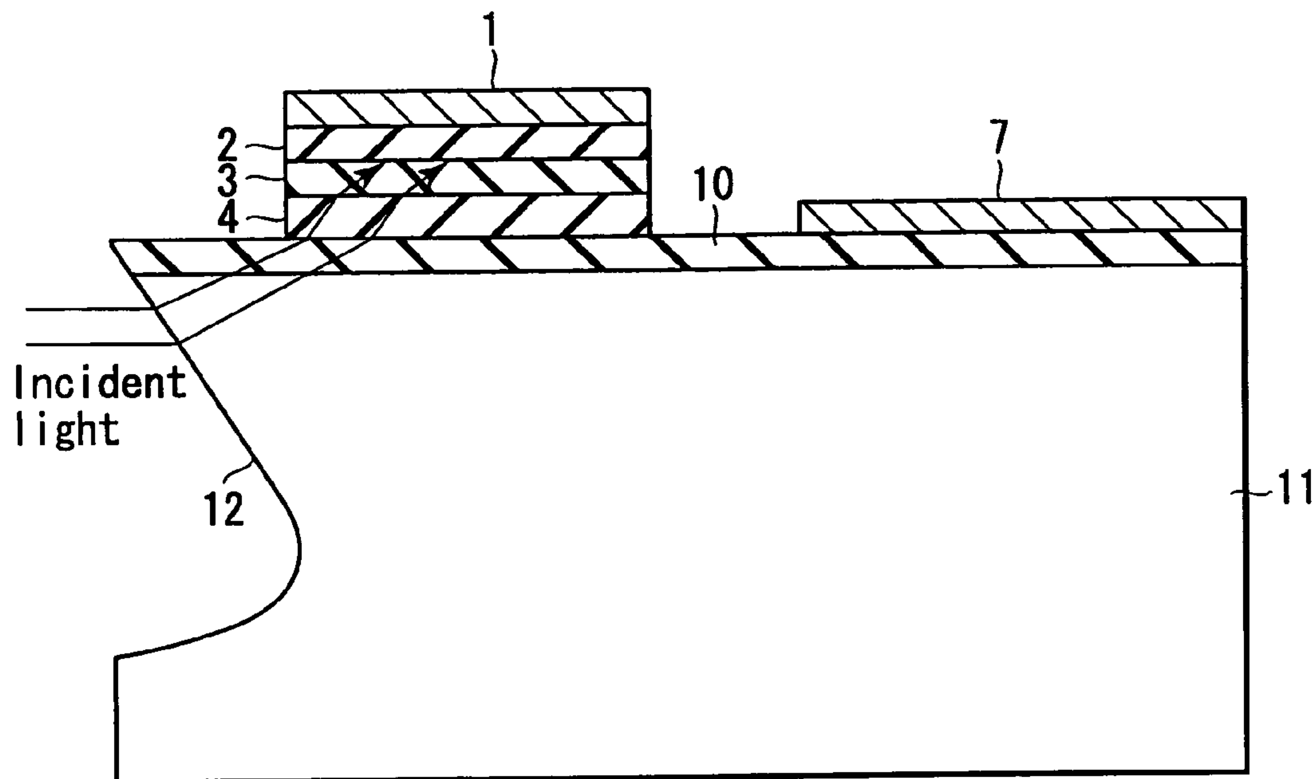
FIG. 42 (PRIOR ART)
