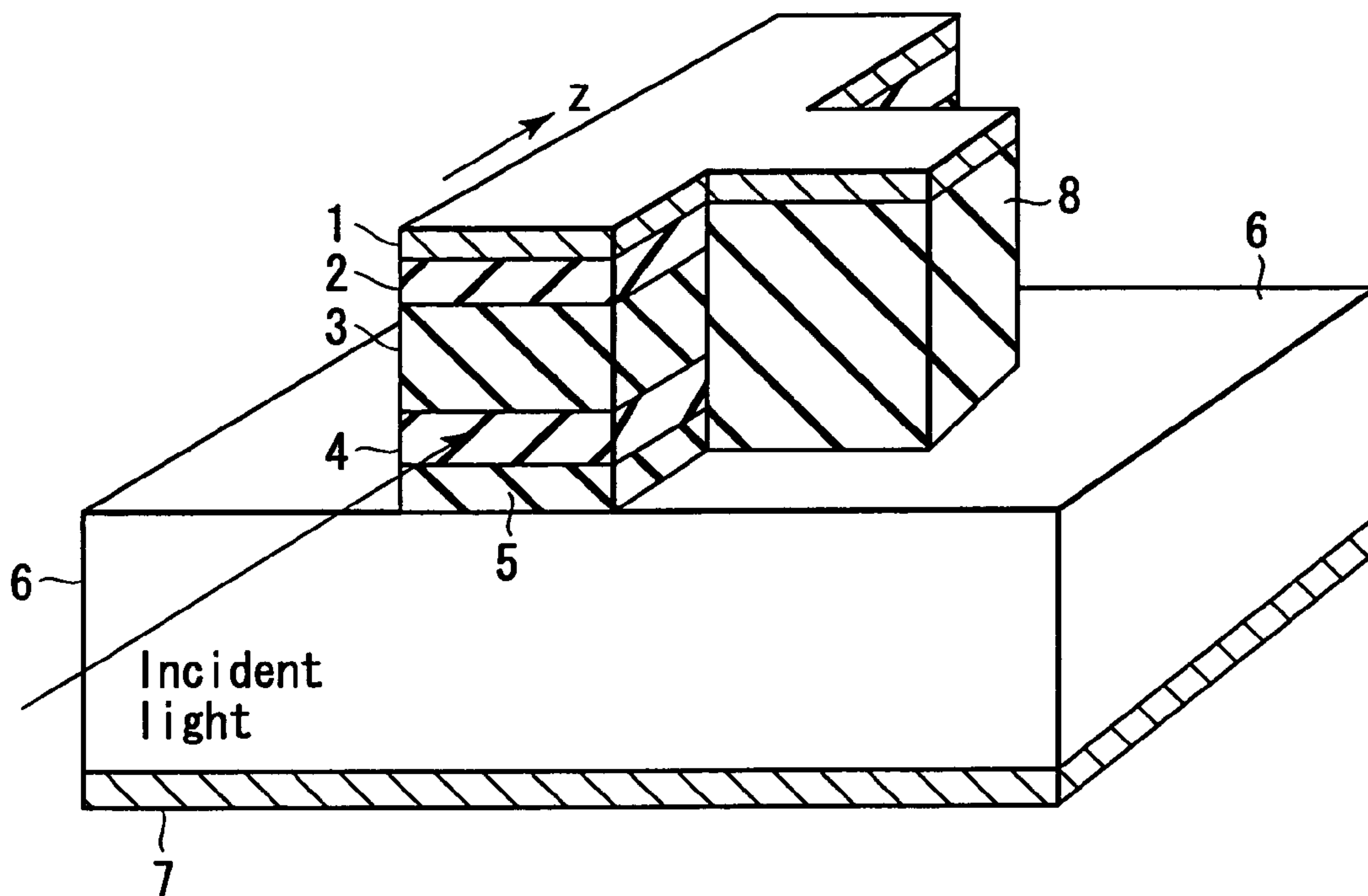
FIG. 36 (PRIOR ART)
