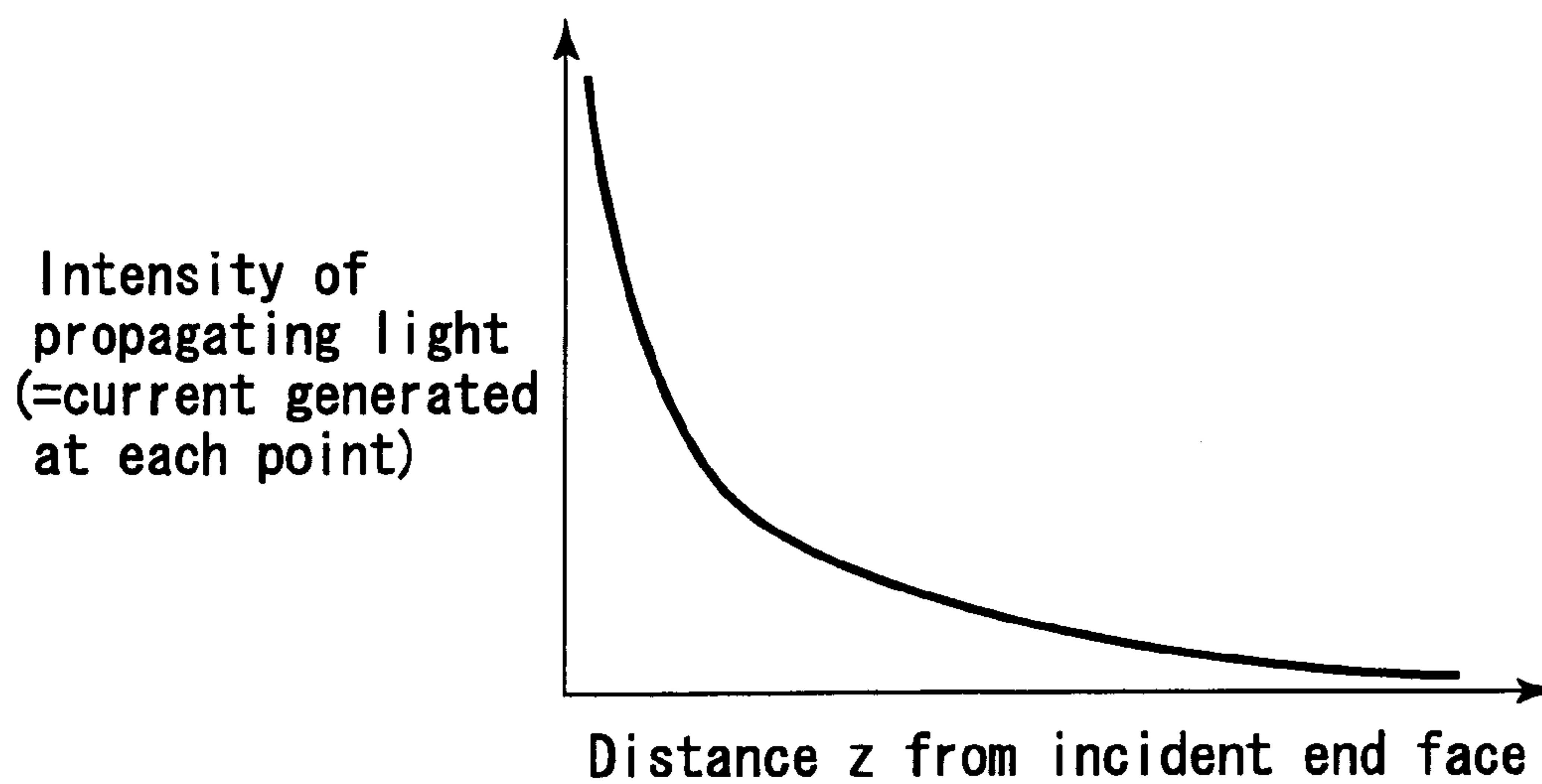
FIG. 37 (PRIOR ART)
