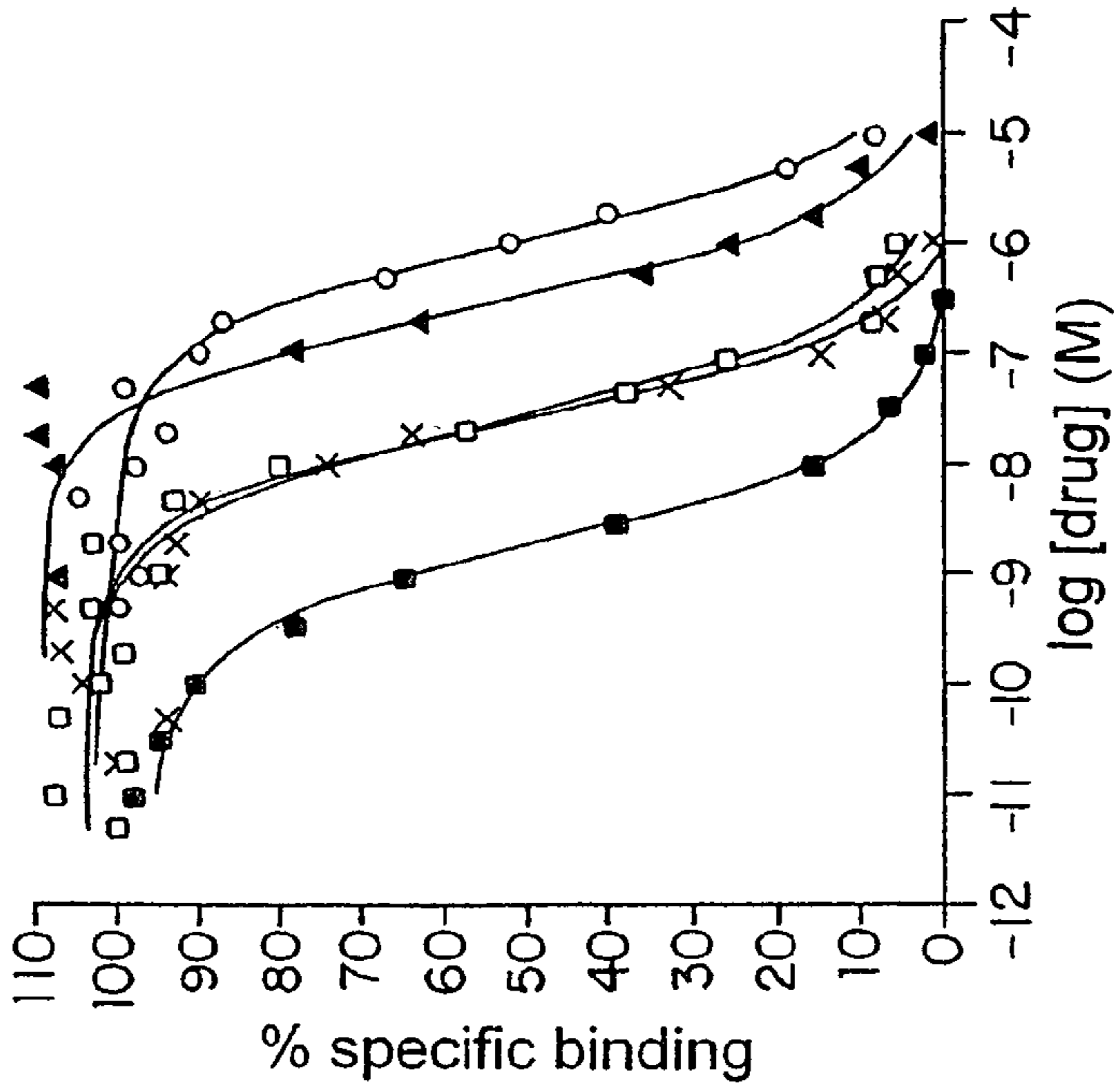
MUSCARINIC, M 2 (HUMAN RECOMBINANT) BINDING ASSAY
