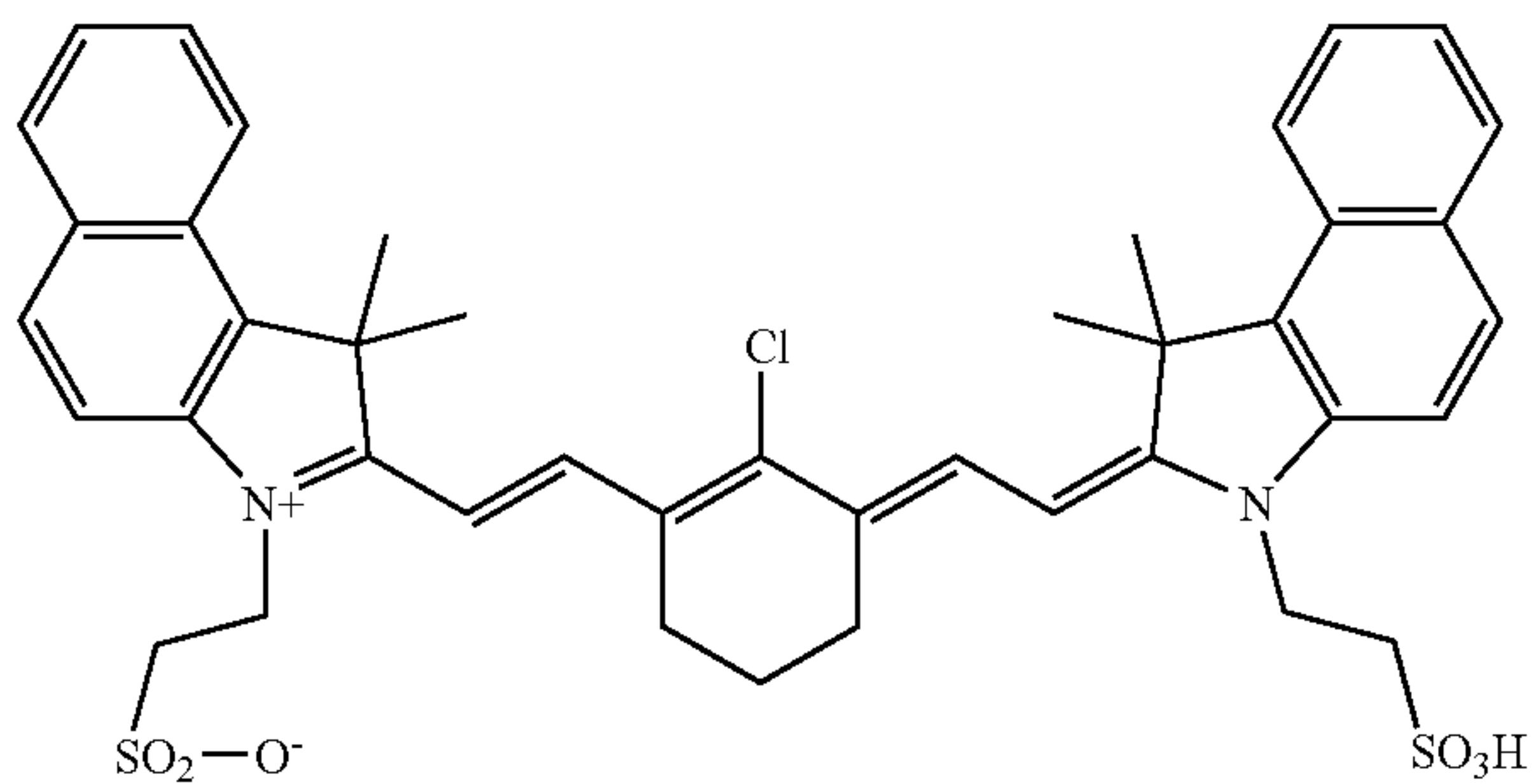
dye I
