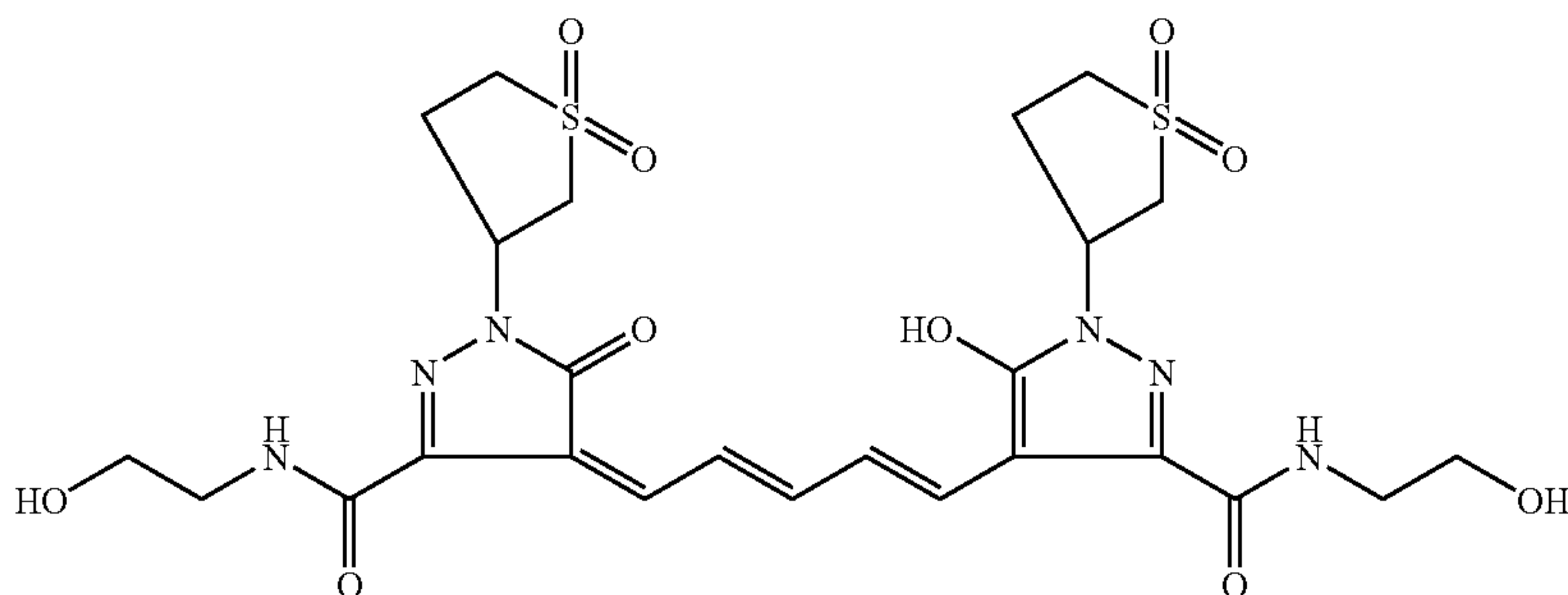
dye I
