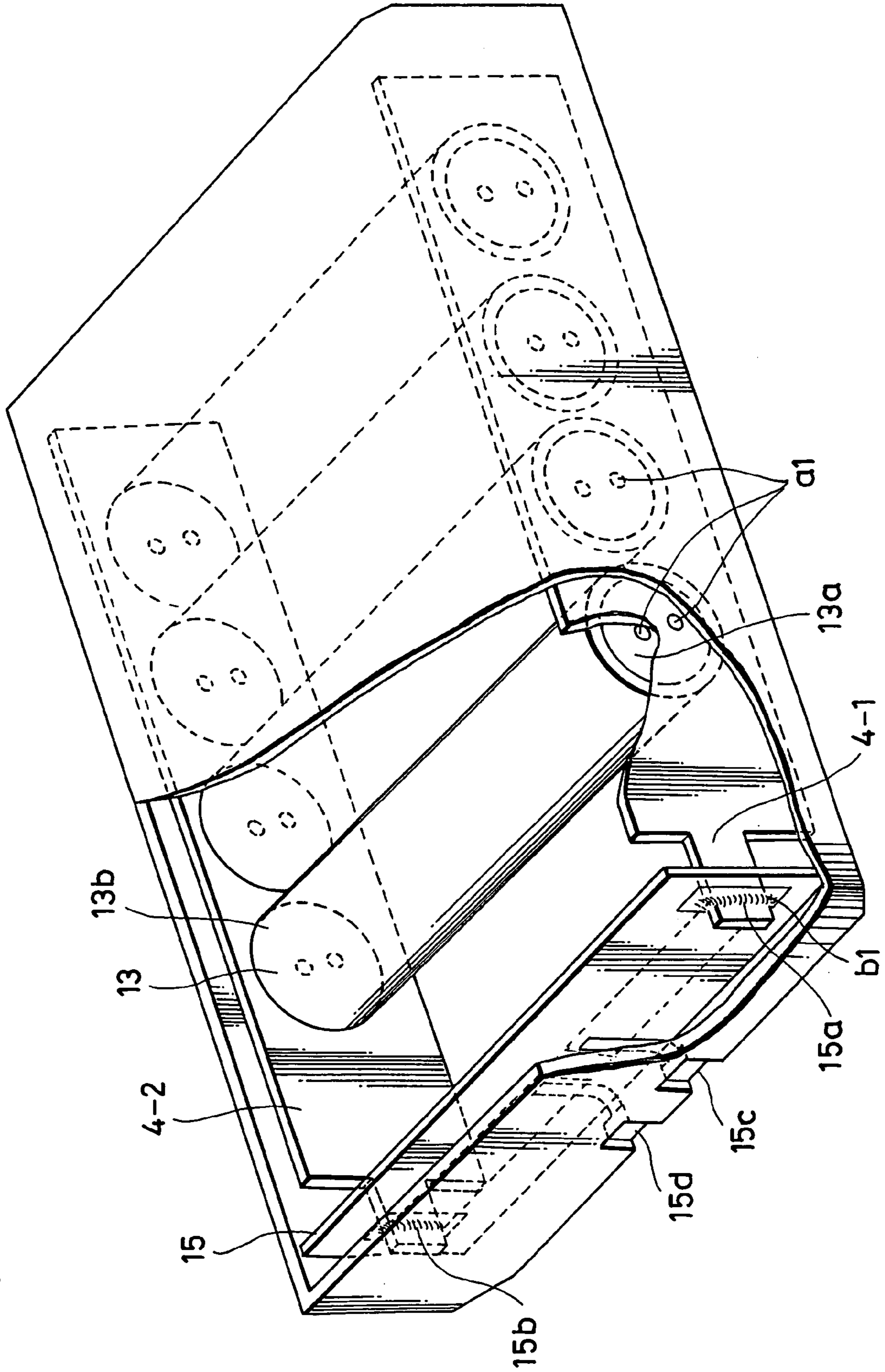
FIG. 1 (RELATED ART)
