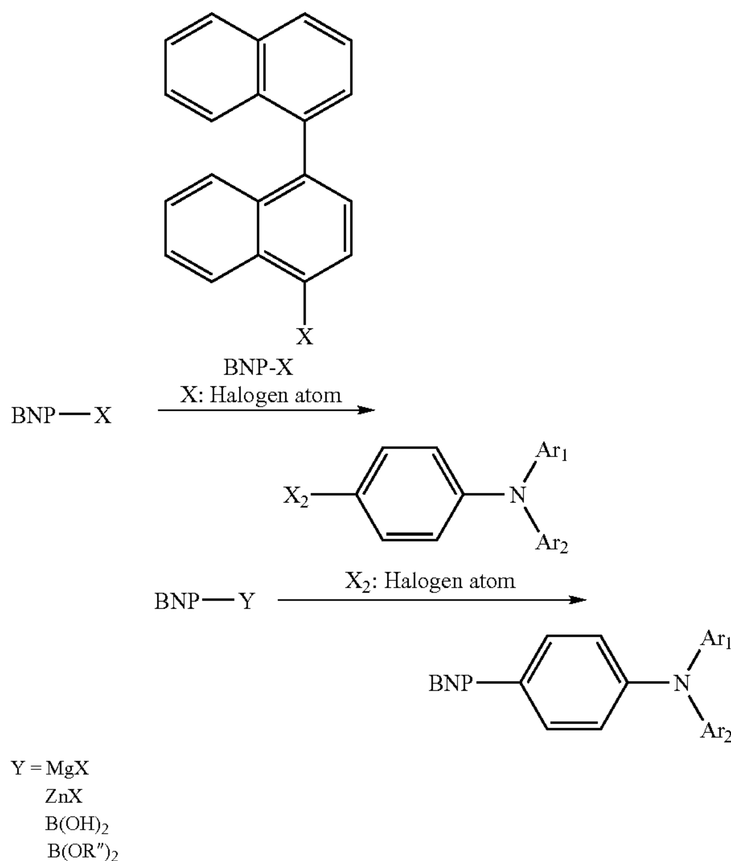
Scheme 2
