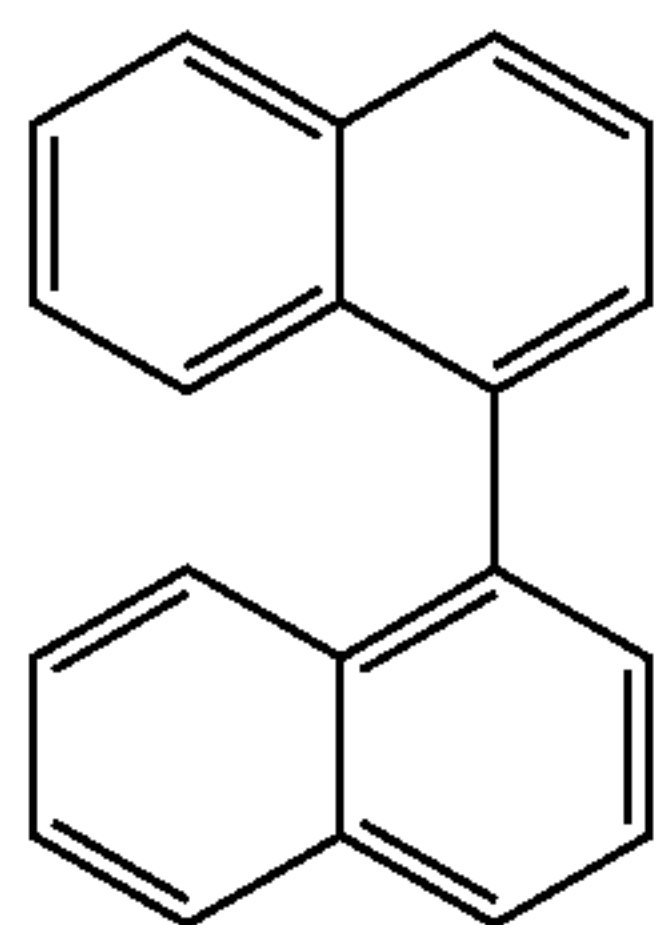
1, 1'-binaphthyl
