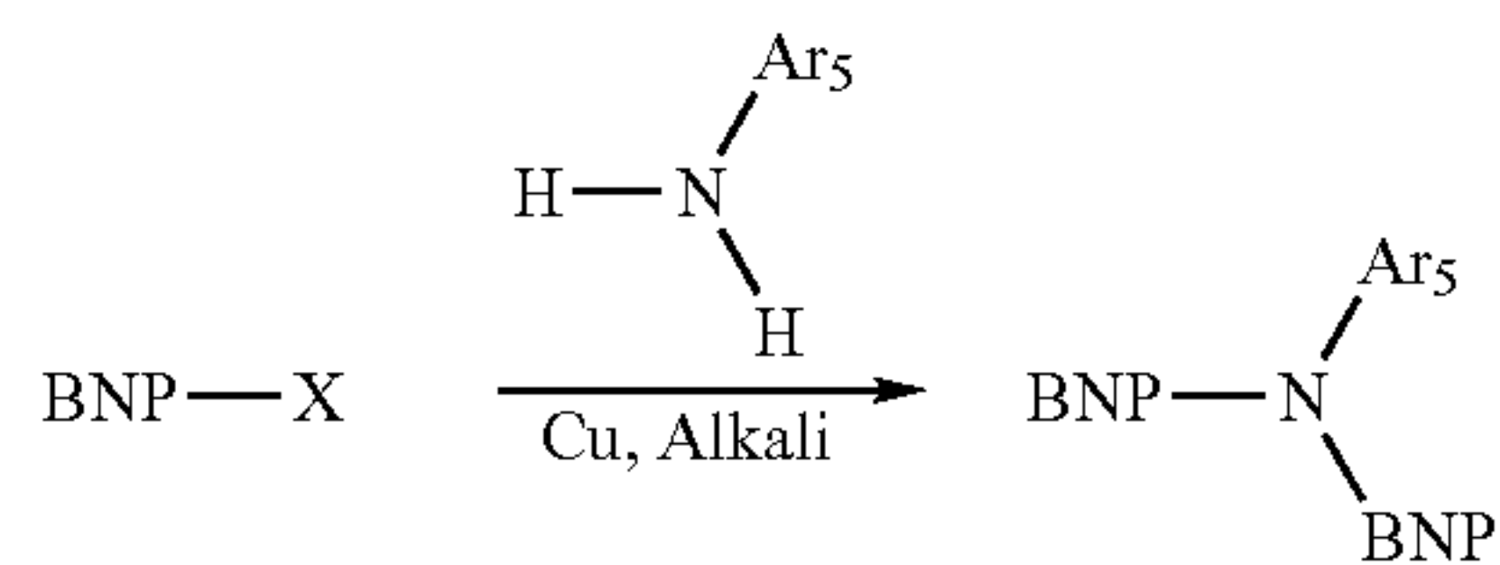
Scheme 5
