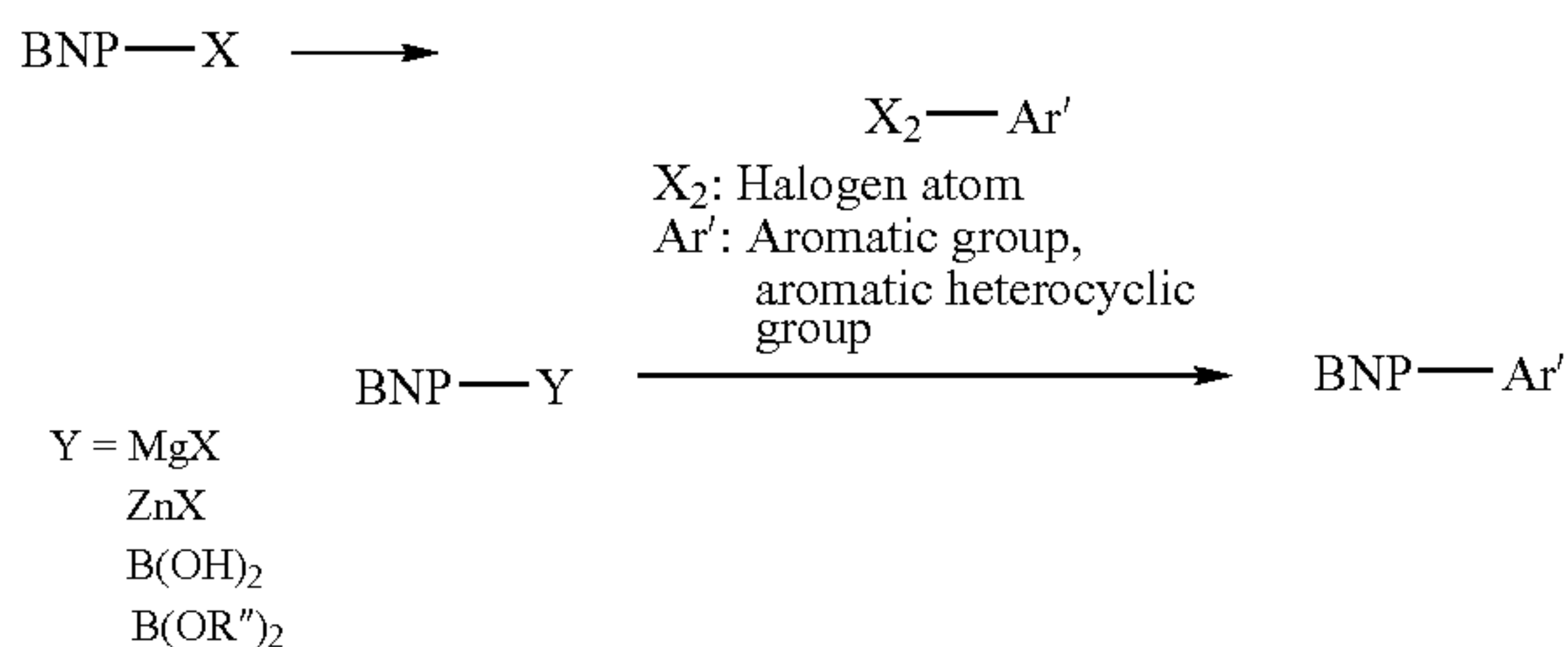
Scheme 3
