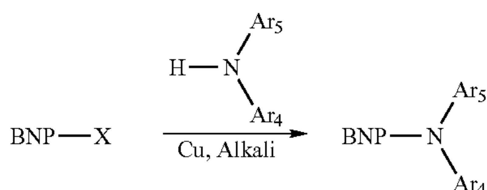
Scheme 4
