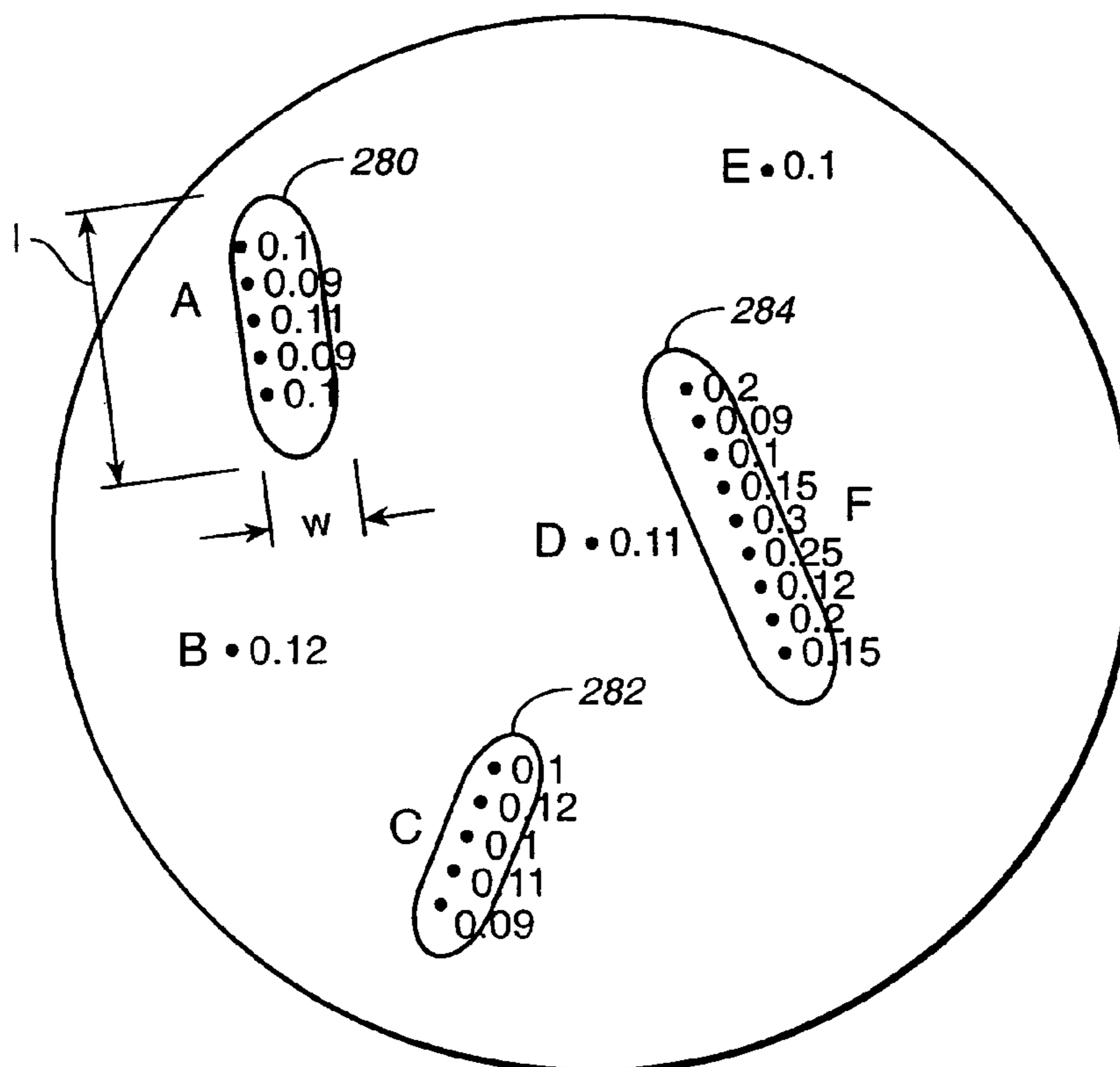
FIG. 5 Initial Clustering in Microscratch Algorithm
